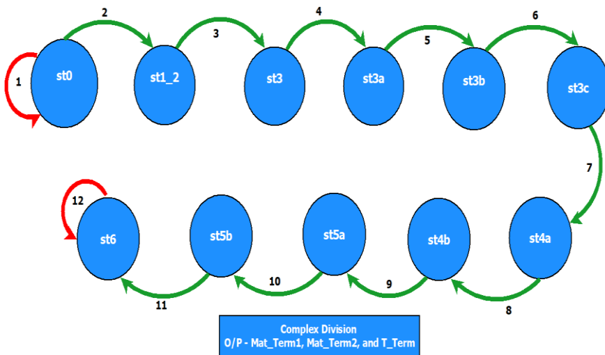
Figure 9. State diagram of the proposed Baudhayan-Pythagorean Triplet algorithm.
