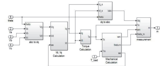
Fig. 6. Expanded PMSM Block.
