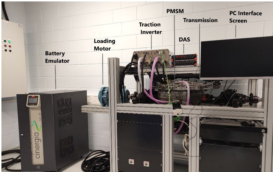
Figure 6. EV propulsion drive system testbench [70].
