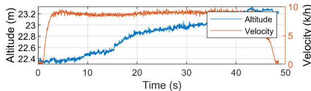
Figure 11. EV GPS-sensor data of vehicle velocity and altitude [Paper V].
