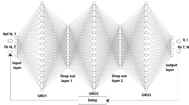
Figure 23. NARX architecture.
