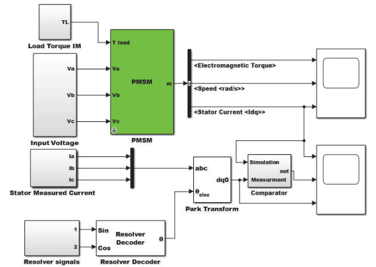
Fig. 4. Simulink model of PMSM testbench.
