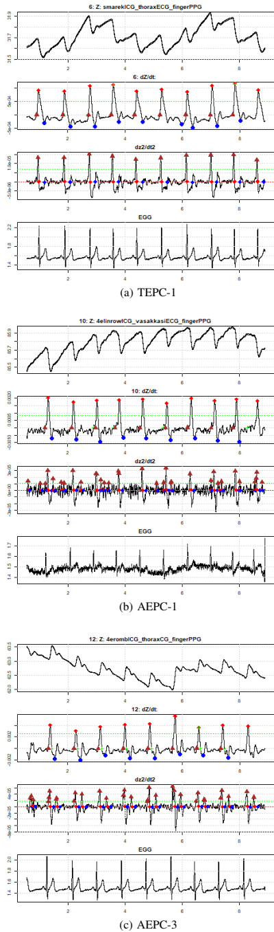
Fig. 11: Waveforms for setups TEPC-1, AEPC1 and AEPC-3
