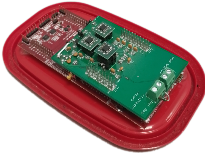
Figure 3: Photo of the first-generation DSP-based impedance measurement prototype, developed during this PhD work.
