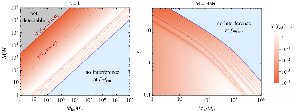
Figure 1. In the light blue region the left-hand side of the interference condition (2.13) is larger than one, and the dotted contour indicates where it is 0.1. In the light gray region |F(f_{\text{cut}})| < 1.0001 . The symmetric mass ratio of the source binary is fixed to \eta = 0.23 .
