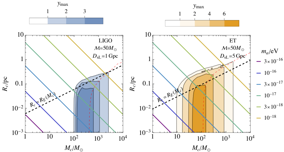
Figure 5. The color shading shows the maximum value of the impact parameter y_{\max} that allows for detection of the lens effect by a uniform density sphere of mass M_c and radius R_c . The binary chirp mass and luminosity distance are fixed as shown in the plot, the symmetric mass ratio of the binary is fixed to \eta = 0.23 and the lens distance to D_{\text{LL}} = 0.5D_{\text{sL}} . The lines show the M_c - R_c relation for DM core for different axion masses m_a , following eq. (3.6). Right from the red dashed curve y_{\max} is set by the interference condition, and the black dashed curve shows the point mass Einstein radius, R_c = R_E(M) .
