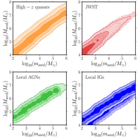
Fig. C.1. Fits to the stellar mass-BH mass data as functions of the seed BH mass m_{\text{seed}} and minimal halo mass M_{\text{seed}} where the seeds are inserted at z_{\text{seed}} = 20 , for p_{\text{BH}} = 1 without spread in the predicted relation in solid and with a log-normal spread ( \sigma = 0.5 ) in dashed.
