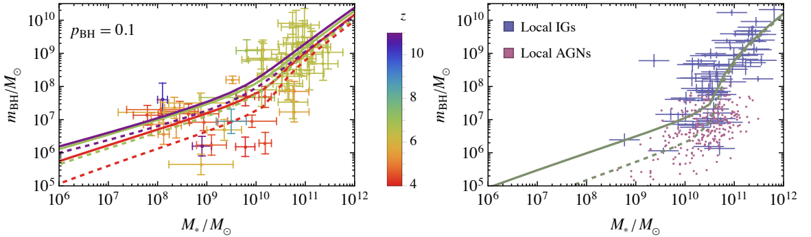
Fig. 5. Comparisons of model predictions for stellar mass-BH mass relation with high- z observations on the left and with low- z observations on the right. The solid lines show the best fit for p_{\text{BH}} = 0.1 to the JWST data, and the dashed lines show the best fit to the rest of the SMBH data. The best-fit parameter values are given in Table 1.
