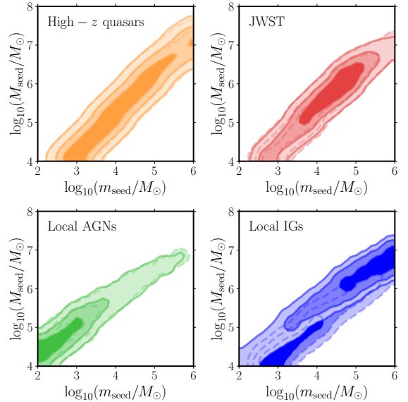
Fig. C.2. As in Fig. C.1 for p_{\text{BH}} = 0.1 .
