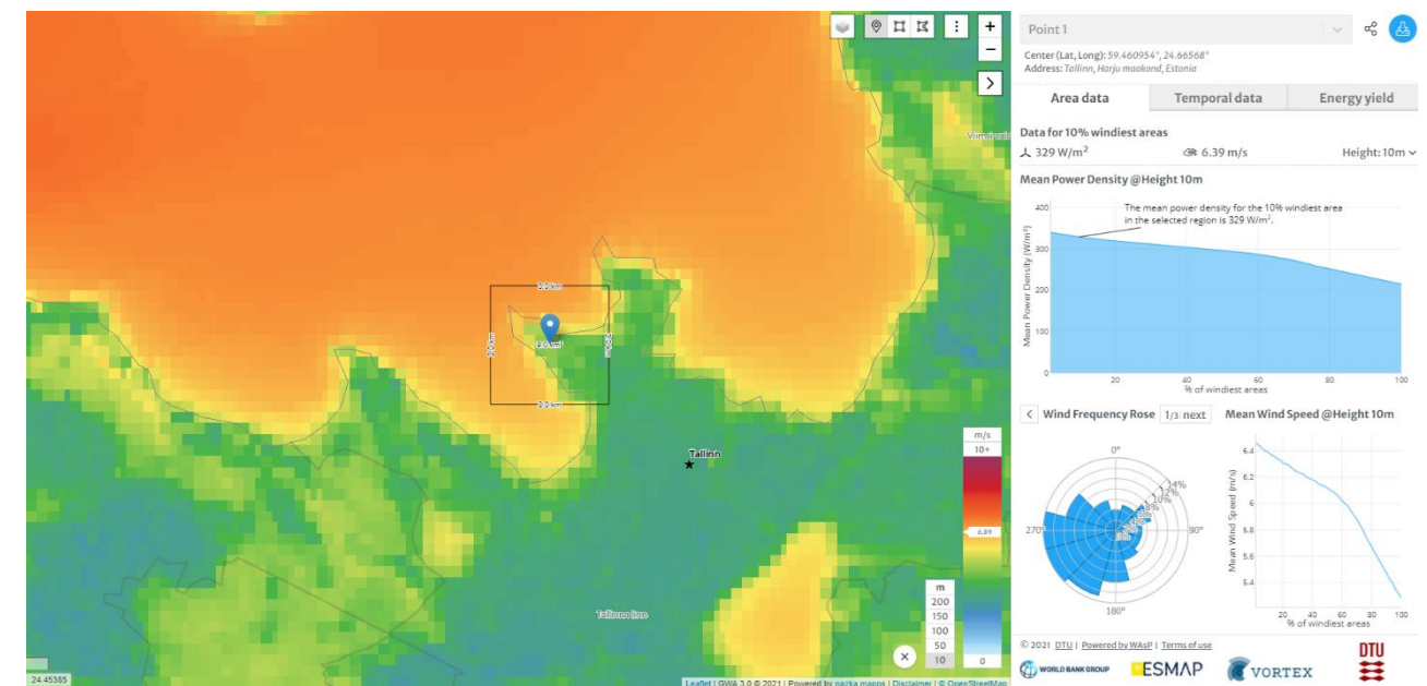
Image 25 Screenshot from Global Wind Atlas showing average wind speed and direction
