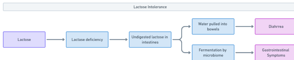
Figure 3.10. Mechanisms of Lactose Intolerance
