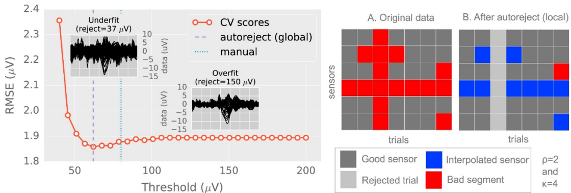
Figure 8. Artefact rejection process by Autoreject algorithm [72]. Left: global AR threshold estimation compared with manual human-set threshold where the used CV metric is the root mean squared error (RMSE) between the mean of the training set and the median of the validation set; for low threshold, the RMSE is high as most of the epochs are rejected (underfit) and for high threshold, the model does not drop any epochs (overfit); optimal threshold is in-between. Right: basis of local AR per each sensor (i.e., channel): the trial (i.e., epoch) is rejected if the number of bad channels > \kappa and otherwise, the worst \rho sensors are interpolated (i.e., repaired).
