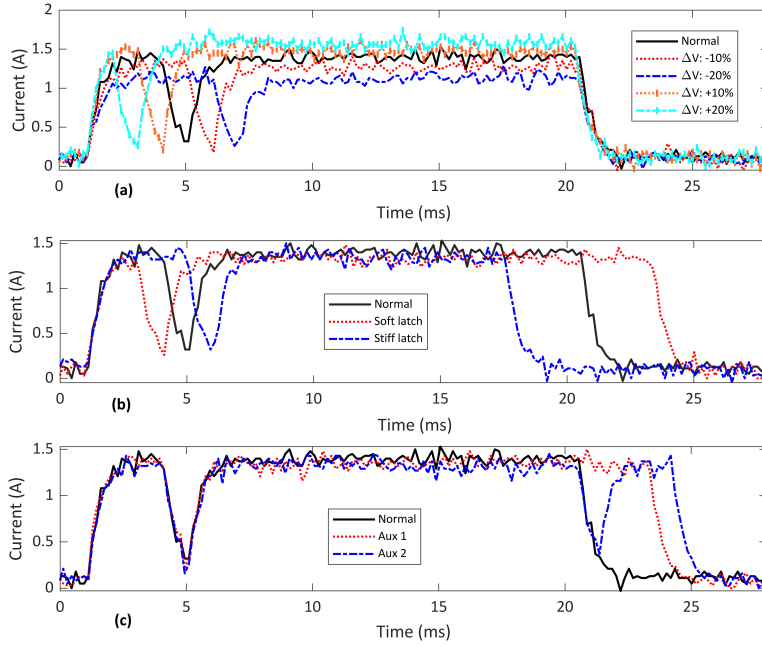
Figure 35: Illustration of the effects of various defects on the coil current waveform: (a) supply voltage, (b) latch operation, (c) auxiliary contact.
