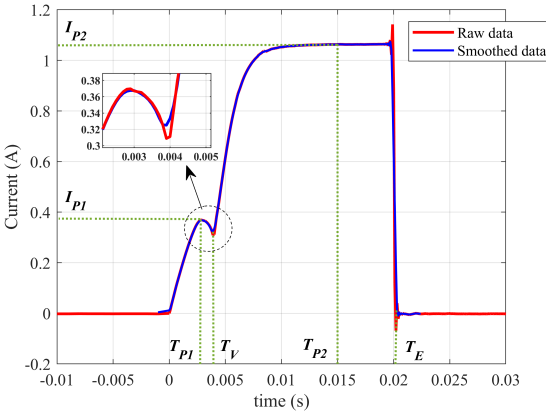
Fig. 1. Smoothing and feature extraction from CC measurement
