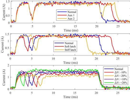
Fig. 3. Illustration of the effects of various defects on the CC waveform.
