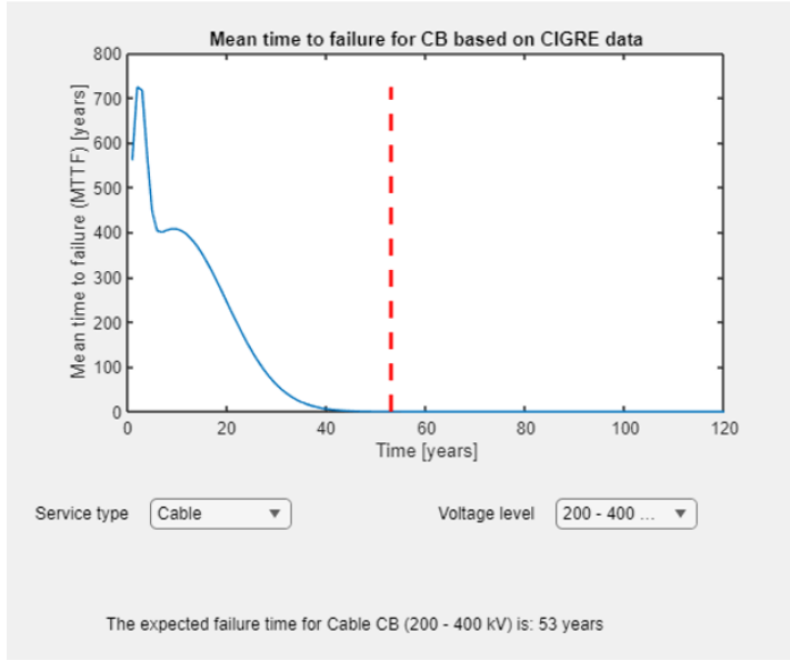
Figure 25: An output sample from the designed graphical user interface
