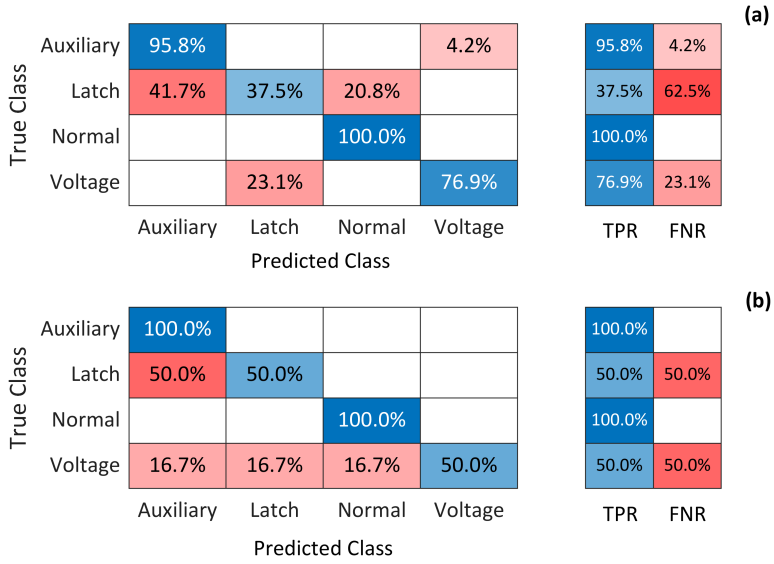
Figure 41: Confusion matrix, TPR, and FNR of the SVM model: (a) Training validation, (b) Testing
