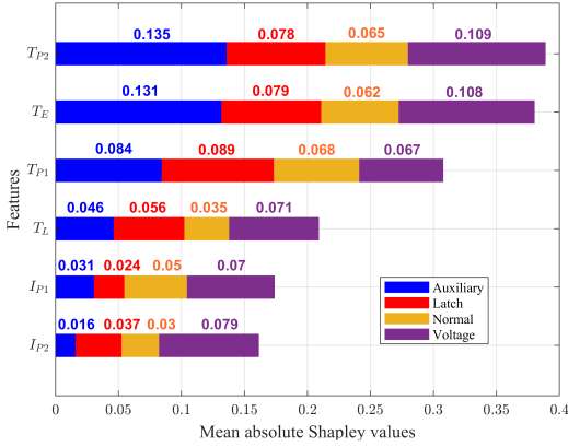
Fig. 11. Global feature importance plot showing the mean absolute Shapley values for each class.
