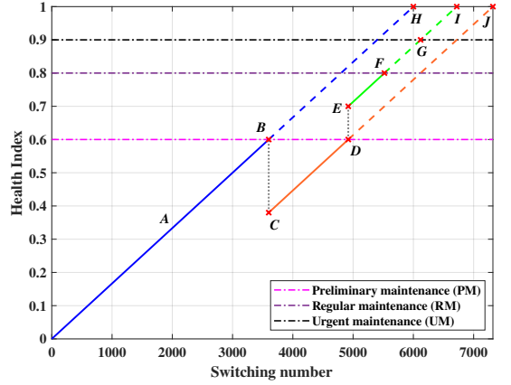
Fig. 4. Modification of expected aging curve of the HVCB using the proposed method (scenario 1)
