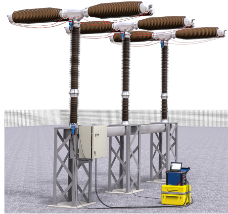
Figure 27: CIBANO 500 connected to a live tank HVCB (a typical field application) [57]
