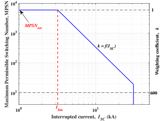
Fig. 1. Sample of MPSN graph for Siemens 3AP1 FG HVCB [18]
