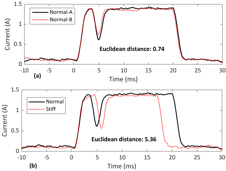
Figure 43: Euclidean distance assessment between filtered coil current signals: (a) comparison of two healthy signals; (b) comparison between a healthy and a defective signal.
