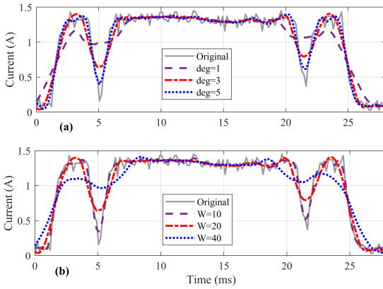
Fig. 5. Sensitivity analysis of the Savitzky-Golay parameters. (a) Effect of polynomial degree variation by constant window size ( W = 20 ). (b) Effect of window size variation by constant polynomial degree ( \deg = 3 ).
