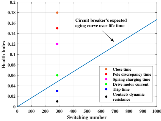
Fig. 3. Experimental measurement tests on Siemens 3AP1-FG model 110 kV HVCB
