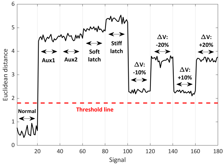
Figure 44: Euclidean distance metrics comparing a reference normal signal against various healthy and defective sample groups.
