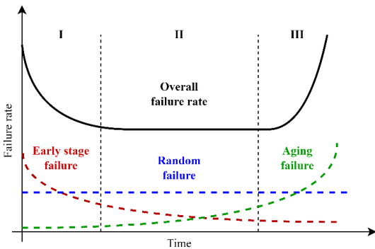
Fig. 1. Typical time-varying failure rate for the power system equipment throughout the lifetime [13]
