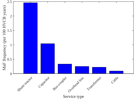
Fig. 2. MaF of HVCB according to the service type based on CIGRE survey [11]
