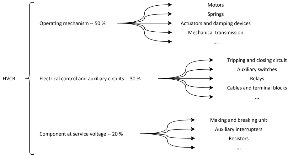
Figure 8: Distribution of HVCB failure per component responsible (data from [20])
