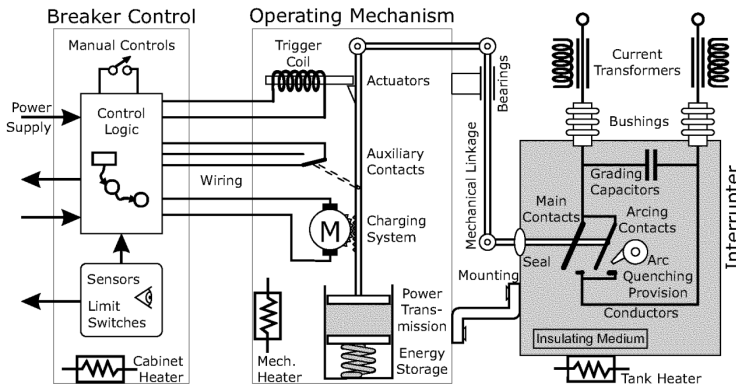
Figure 14: Generic model of HVCB components [48]
