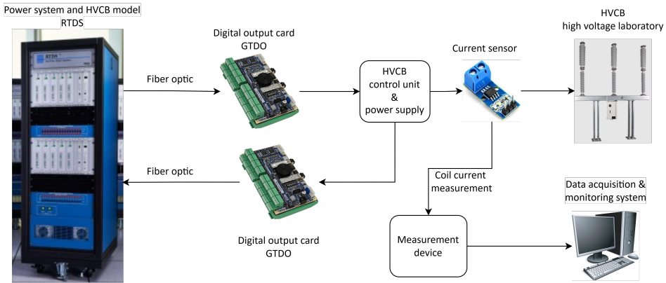
Figure 50: Schematic of the experimental setup
