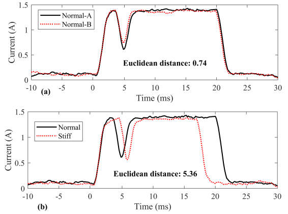
Fig. 6. Euclidean distance between two filtered coil current signals. (a) Both signals are normal and (b) normal versus defected signal.
