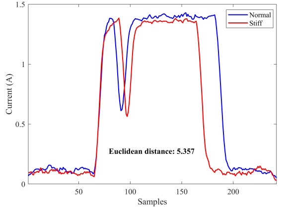
Fig. 5. Euclidean distance between normal and defected signals
