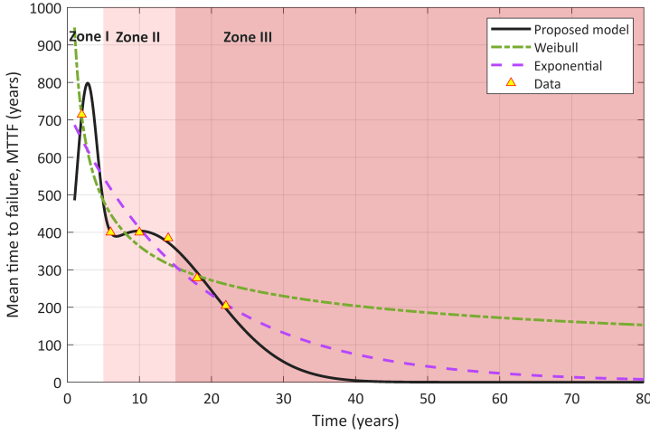
Figure 22: Comparison of the proposed model to Weibull and exponential models
