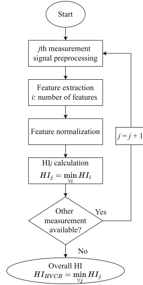
Fig. 1. Flowchart of the overall HI calculation for HVCB
