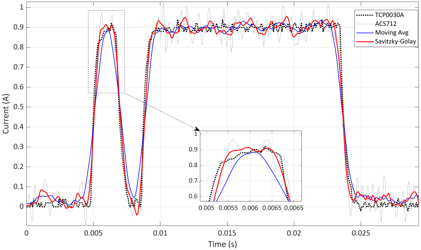
Figure 34: Time-domain comparison of denoising techniques.
