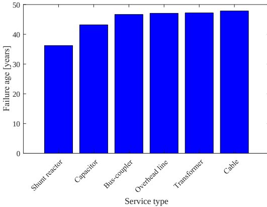
Fig. 4. Incorporating service type for failure age of HVCB based on the proposed model
