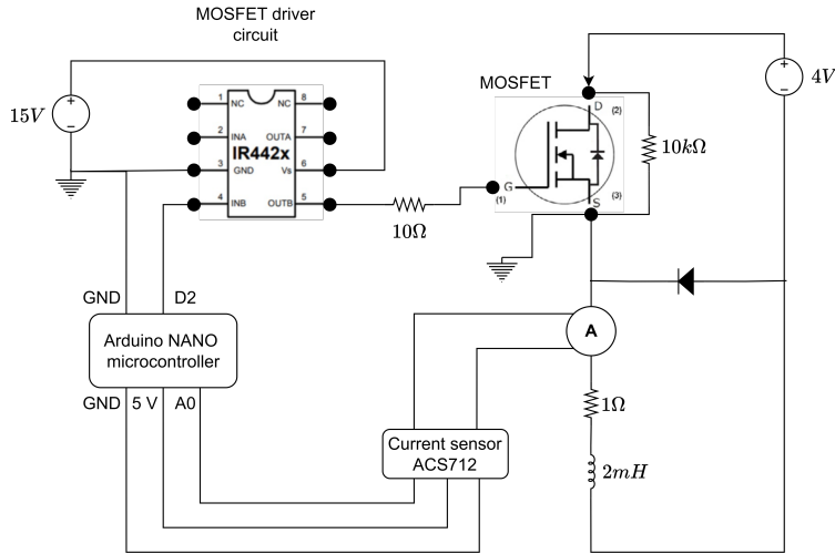
Figure 30: Coil current emulator circuit diagram
