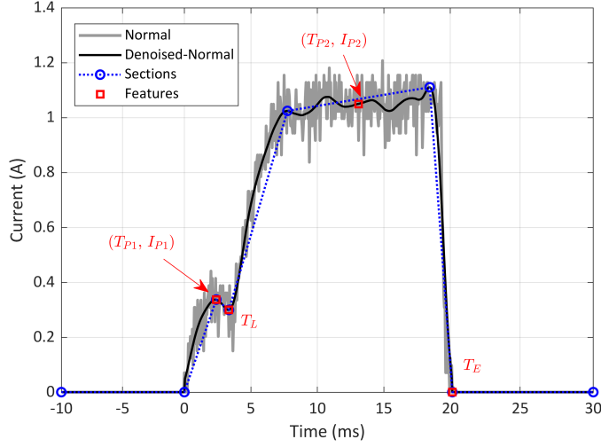
Figure 51: Feature extraction from a real coil current measurement (110 kV circuit breaker).
