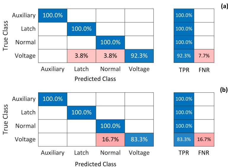
Figure 38: Confusion matrix, TPR, and FNR of the kNN model: (a) Training validation, (b) Testing
