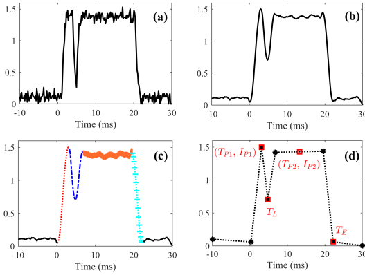
Fig. 2. Trip/close coil current signal feature extraction process. (a) Raw measurement. (b) Filtered signal. (c) Segmentation. (d) Extracting required features.
