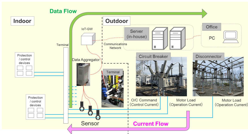
Figure 52: Layered architecture for the practical deployment of HVCB condition monitoring in a transmission network [62].
