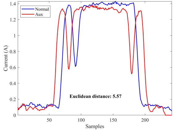
Fig. 8. Comparison of normal and defected signals with time discrepancy
