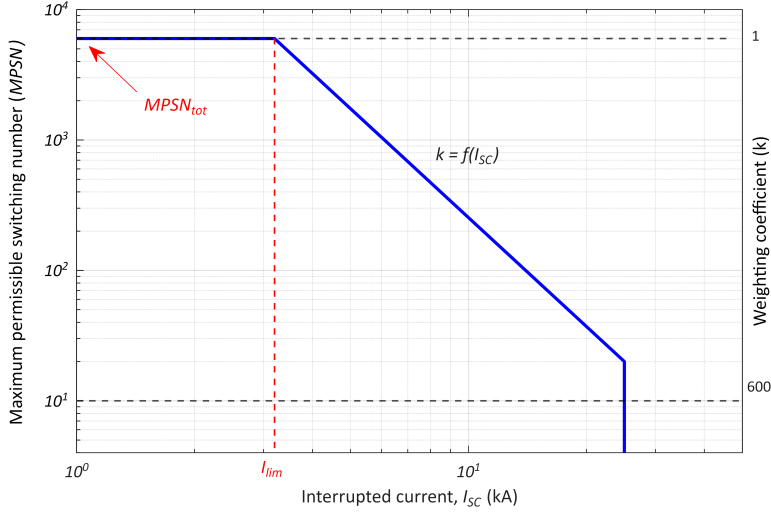
Figure 10: Sample of maximum permissible switching number graph for a 400 kV HVCB (data from [35])
