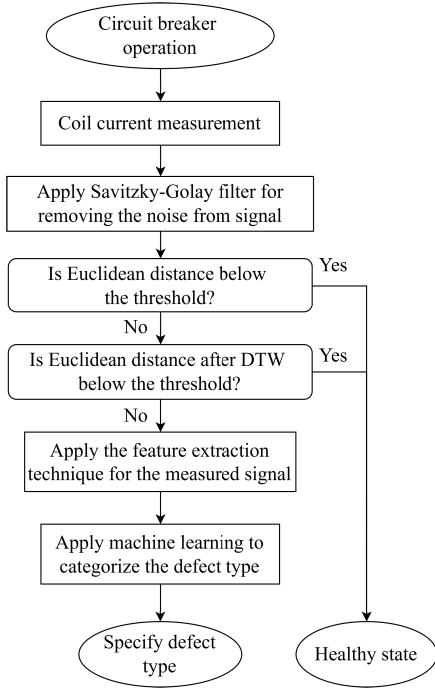
Fig. 9. Flowchart of detection and classification of defect in HVCB.
