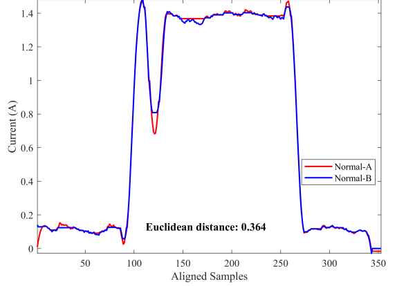
Fig. 7. Application of DTW for two normal signals' alignment
