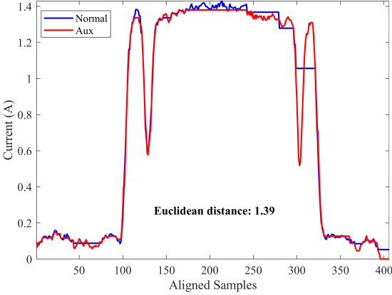
Fig. 9. Application of DTW for signal alignment
