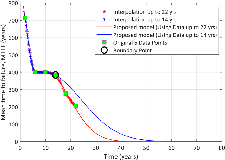
Figure 23: Comparison of Gaussian model extrapolation trajectories when fitted on data truncated at 14 years versus 22 years.
