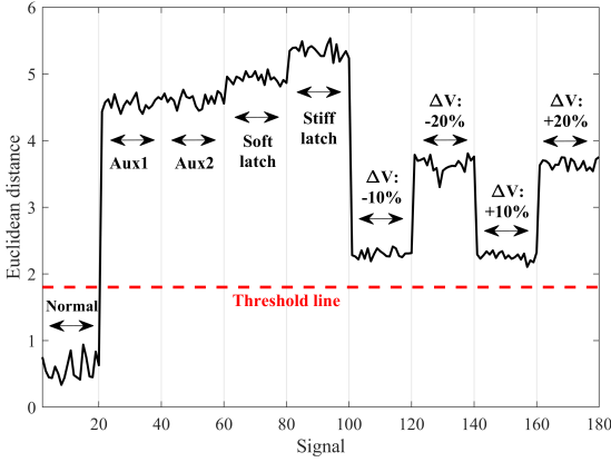
Fig. 7. Euclidean distance between normal and defected signals.
