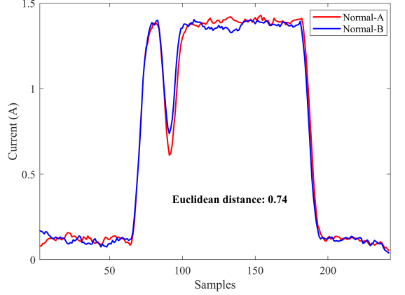
Fig. 4. Euclidean distance between two normal signals
