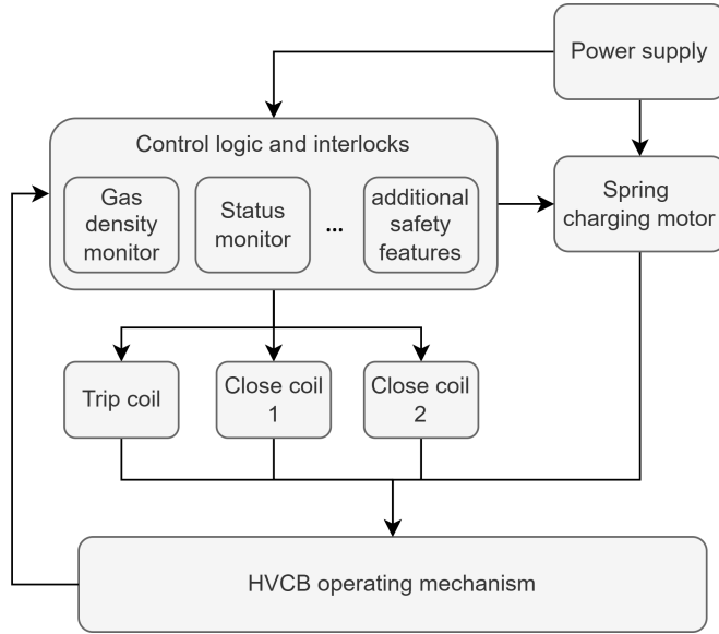
Figure 19: Schematic of a generalised HVCB control circuit
