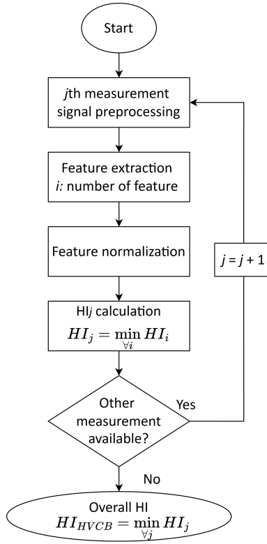
Figure 48: Flowchart of the overall HI calculation for HVCB.
