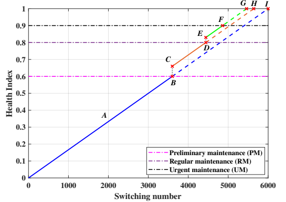
Fig. 5. Modification of expected aging curve of the HVCB using the proposed method (scenario 2)
