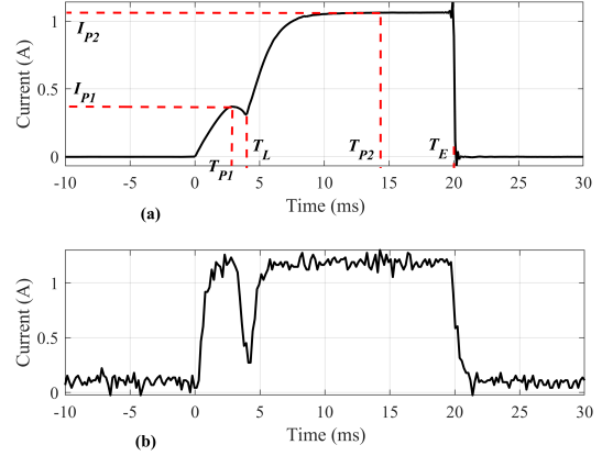
Fig. 1. Trip/close coil current signal and related diagnostic features. (a) Real HVCB coil current measured with a commercial device. (b) Emulator circuit current measured using an inexpensive sensor (normal coil current).
