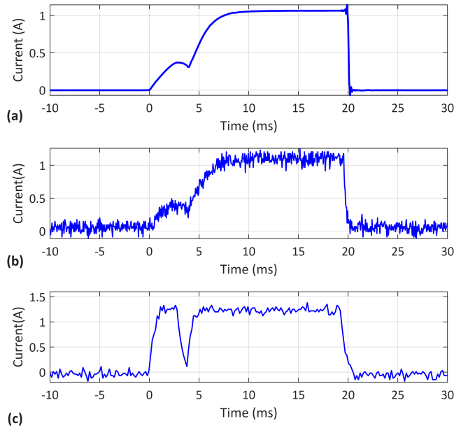
Figure 31: Trip/close coil current signal and related diagnostic features. (a) Real HVCB coil current measured with CIBANO 500. (b) Real HVCB coil current measured using Raspberry Pi. (c) Emulator circuit current measured using an inexpensive sensor.
