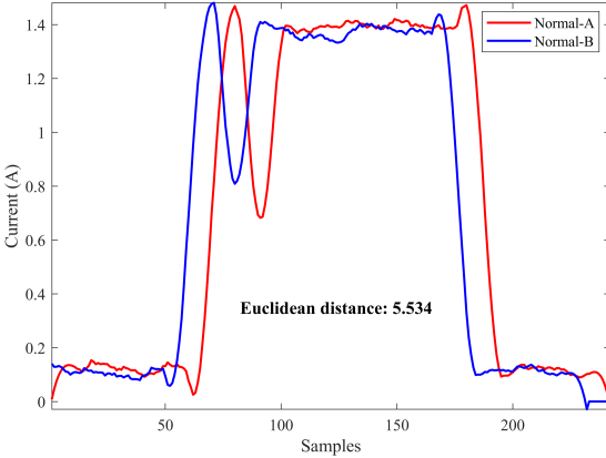
Fig. 6. Comparison of two normal signals with time discrepancy
