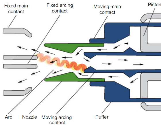
Figure 17: Interrupter principle [19]
