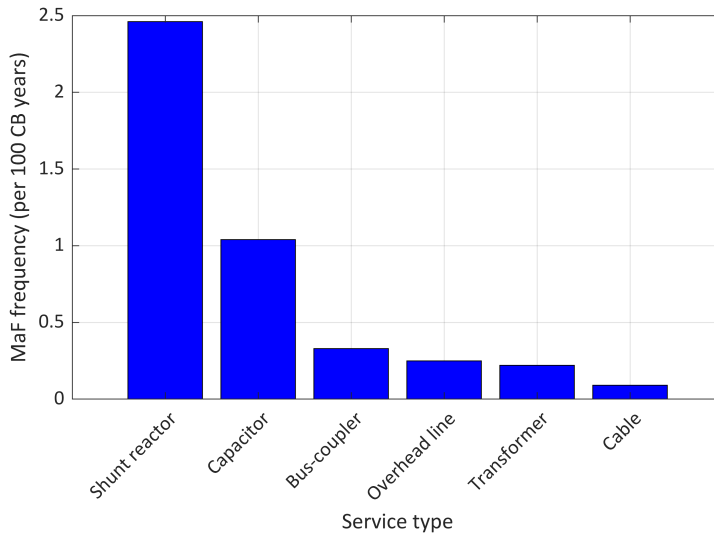
Figure 20: Major failure of HVCB according to the service type based on CIGRE survey [34]
