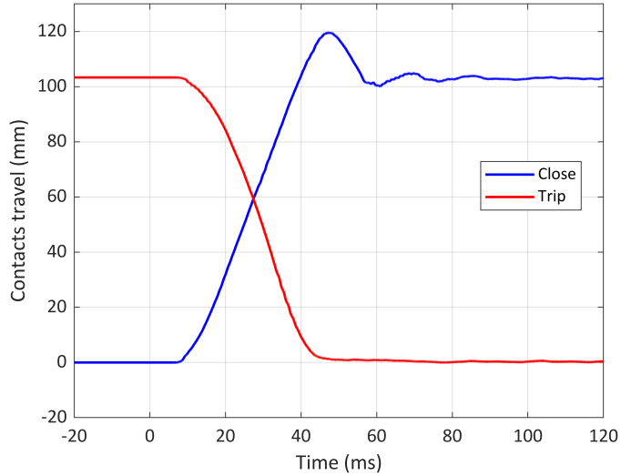
Figure 13: Circuit breaker contacts travel curve for trip/close operation [14]
