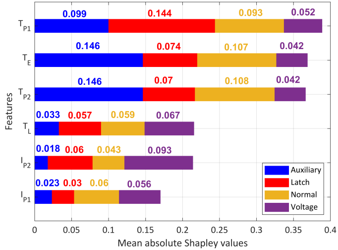
Figure 42: Global feature importance plot showing the mean absolute Shapley values for each class
