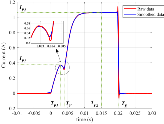
Fig. 2. Smoothing and feature extraction from CC measurement
