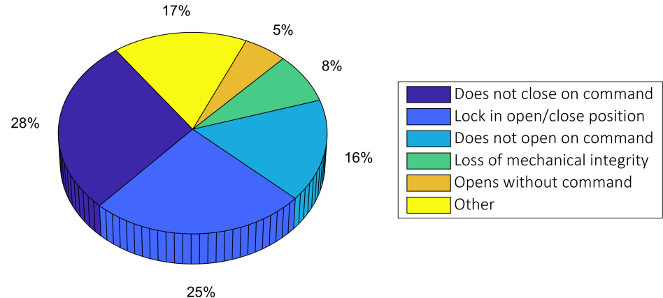
Figure 7: Failure modes of major failures for HVCB (data from [34])
