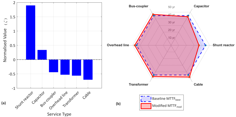
Figure 24: Impact of normalized service-type integration on HVCB life expectancy: (a) normalised failure rates ( \zeta ) per service-type; (b) comparison between MTTF_{base} and MTTF_{mod} .
