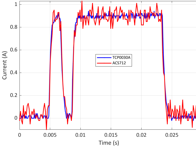
Figure 32: Time-domain comparison of signals captured by TCP0030A and ACS712
