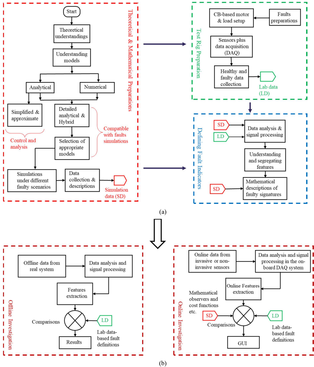
Fig. 4. (a) The simulations, test rig preparations and defining benchmark fault indicators, (b) implementation of rules in online and offline predictive maintenance environments
