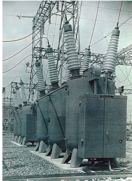
(b) 168 kV bulk-oil, dead tank oil circuit breaker, 1959
