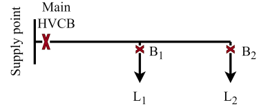
Fig. 4. The scheme of the network under study
