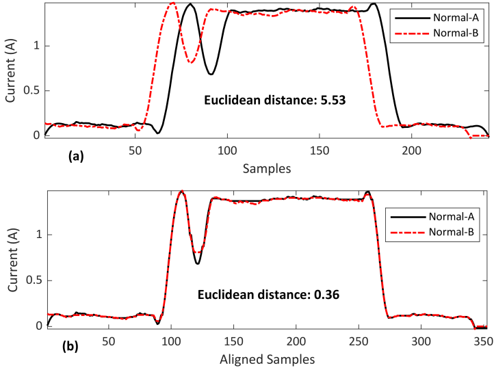
Figure 45: Impact of DTW on signal alignment: (a) misaligned normal signals yielding high Euclidean error; (b) signals aligned via DTW revealing true similarity.
