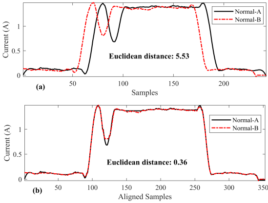
Fig. 8. Application of DTW for signal alignment. (a) Two misaligned normal signals and (b) aligned signals after applying DTW.
