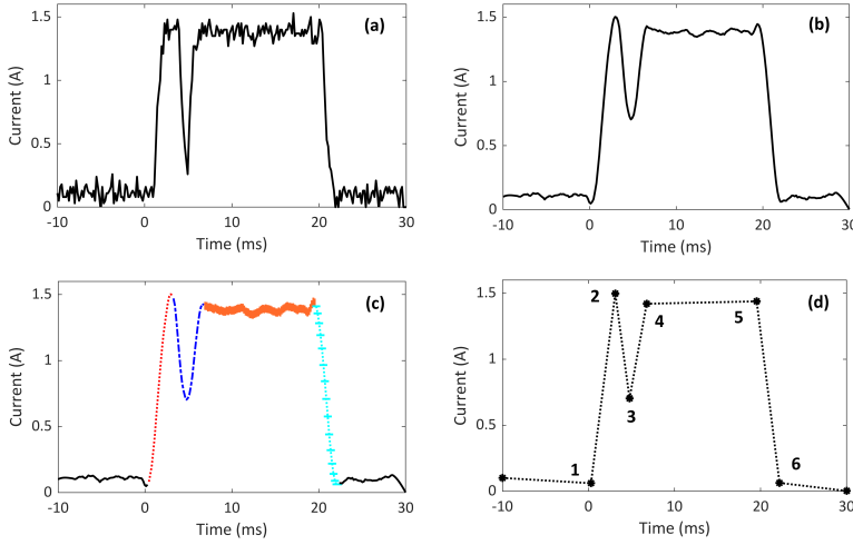
Figure 36: Trip/close coil current signal feature extraction process. (a) Raw measurement. (b) Filtered signal. (c) Segmentation. (d) Extracting critical points.
