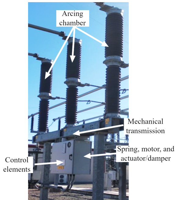
Figure 15: Component specification of a 110 kV HVCB
