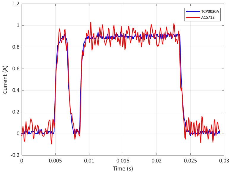
Figure 33: Demonstration of the reference (TCP0030A) and modified signal (ACS712)
