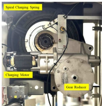
Fig. 1. Universal motor employed for circuit breaker spring charging.
