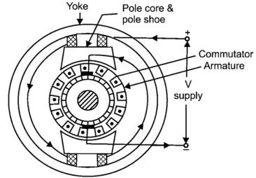
Fig. 2. Schematic of a universal motor [3]
