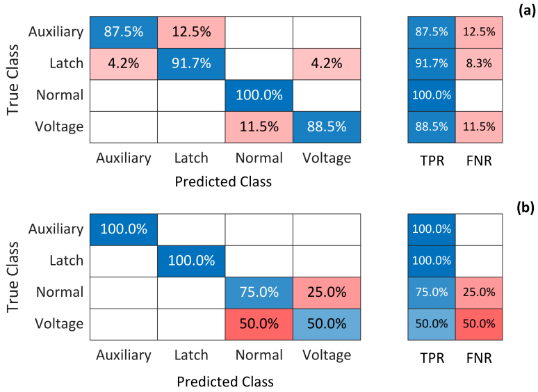
Figure 39: Confusion matrix, TPR, and FNR of the decision tree model: (a) Training validation, (b) Testing
