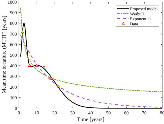
Fig. 3. Comparison of the proposed model to Weibull and exponential models
