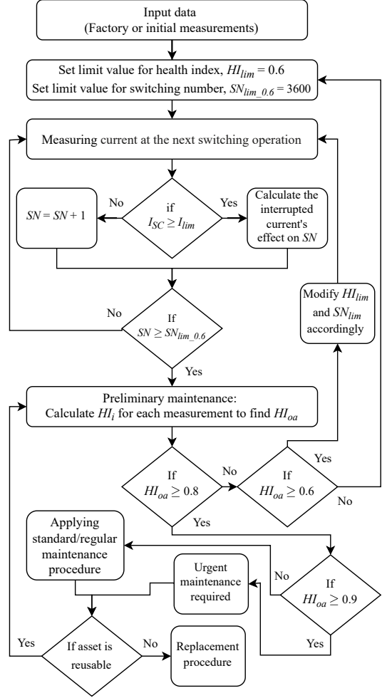
Fig. 2. Implementation process of the proposed method for HVCB's CBM
