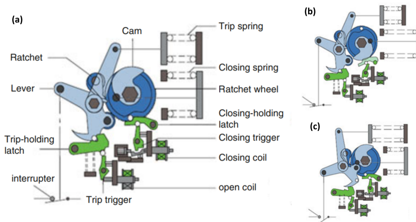
Figure 18: Schematic configuration of a spring operating mechanism: (a) components (b) close (c) trip [18]
