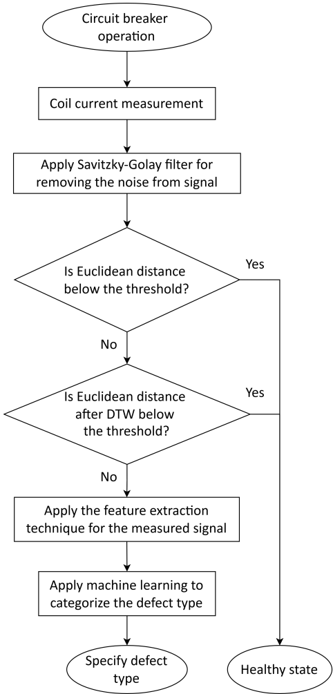
Figure 46: Operational flowchart for the automated detection and classification of HVCB defects.
