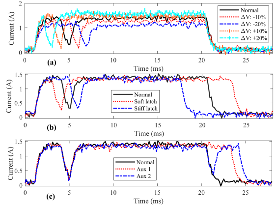
Fig. 4. Illustration of the effects of various defects on the coil current waveform. (a) Supply voltage. (b) Latch operation. (c) Auxiliary contact.
