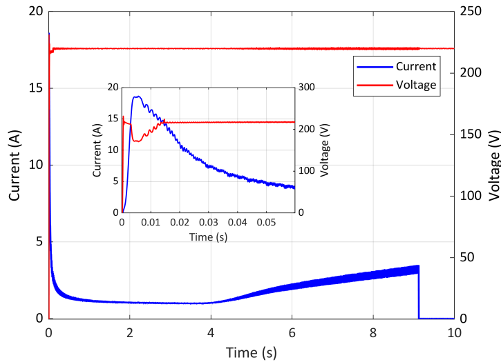
Figure 11: Circuit breaker's spring charging motor current and voltage characteristics
