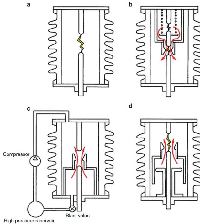
Figure 16: Cross-section comparison of \text{SF}_6 gas Interrupters: a) Plain break, (b) Self blast, (c) Double pressure blast, (d) Puffer blast [19]
