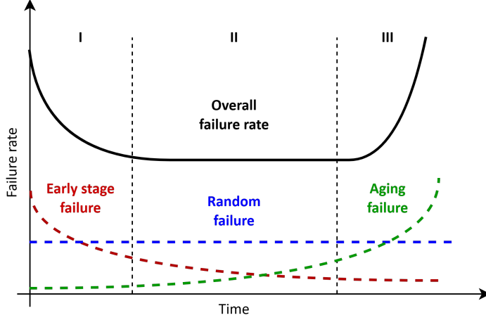
Figure 21: Typical time-varying failure rate for the power system equipment throughout the lifetime
