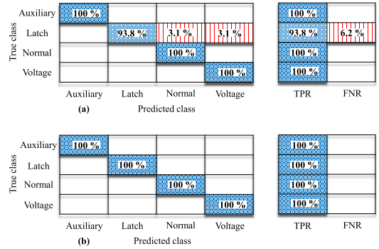
Fig. 10. Confusion matrix, TPR, and FNR of the KNN model. (a) Training validation. (b) Testing.
