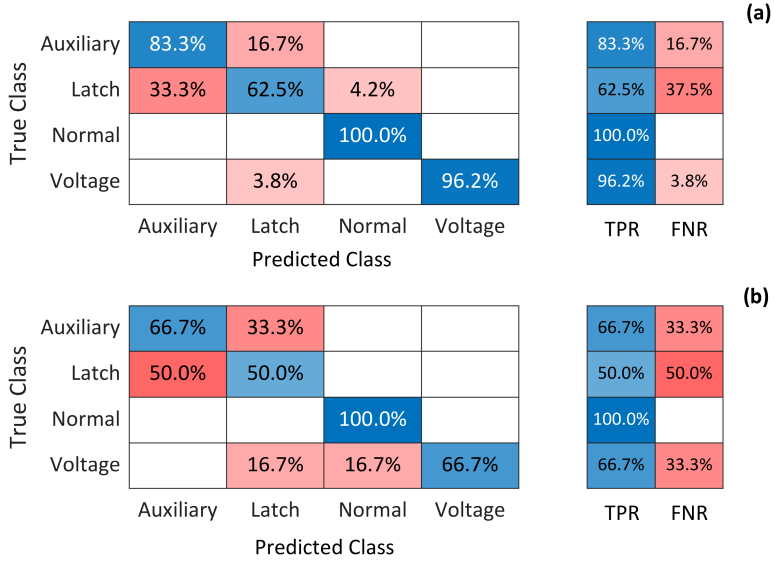
Figure 40: Confusion matrix, TPR, and FNR of the logistic regression model: (a) Training validation, (b) Testing
