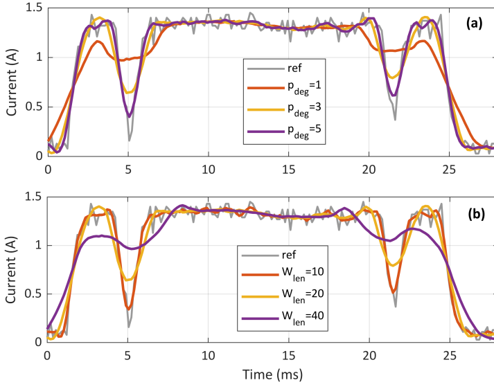
Figure 37: Sensitivity analysis of the Savitzky-Golay parameters. (a) Effect of polynomial degree variation by constant window size ( W_{len} = 20 ). (b) Effect of window size variation by constant polynomial degree ( p_{deg} = 3 ).
