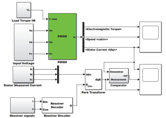
Fig. 4. Simulink model of PMSM testbench.
