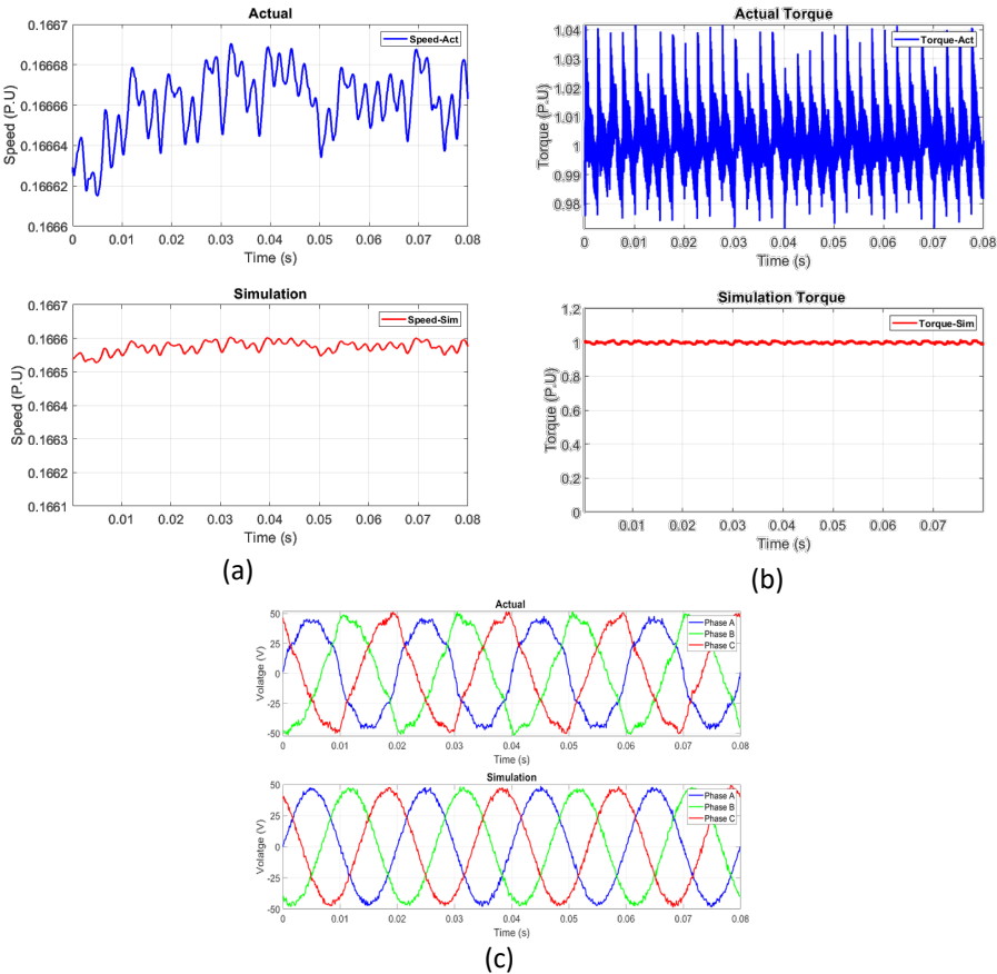
Figure 26. Case (X) Actual and virtual speed (a), torque (b), and input voltage (c).
