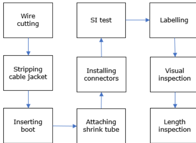
Figure 2.1 (Sample) production and testing process (Jem Electronics, 2018)
