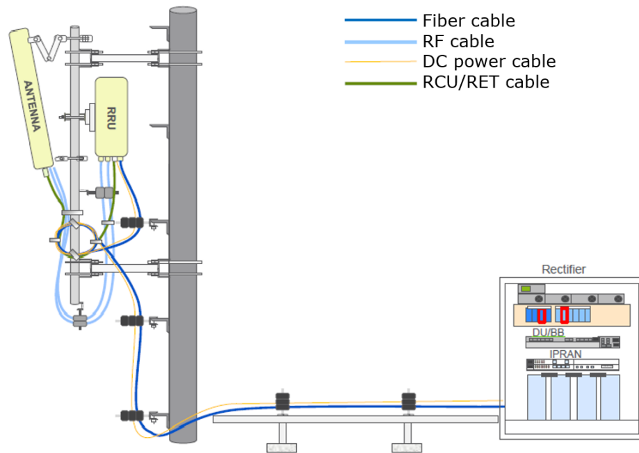
Figure 1.4 Example of a single sector (cell) site (Ericsson, 2016)
