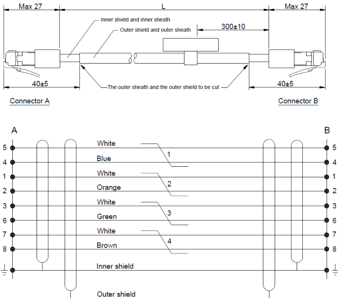
Figure 2.2 Drawing of RJ45-RJ45 signal cable with colour requirements and connection positions of the wires
