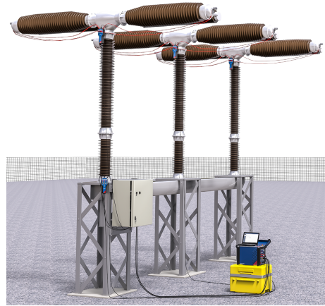
Figure 27: CIBANO 500 connected to a live tank HVCB (a typical field application) [58]
