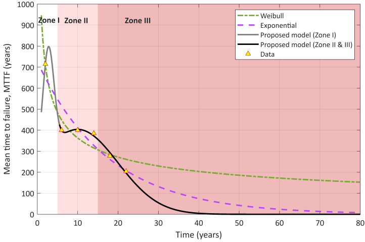
Figure 22: Comparison of the proposed model to Weibull and exponential models in analogy to the bathtub curve zones, shown in Fig. 21; Due to a lack of data in Zone I, the proposed model cannot be fully validated in this region, and this unvalidated section is denoted by the solid gray line.
