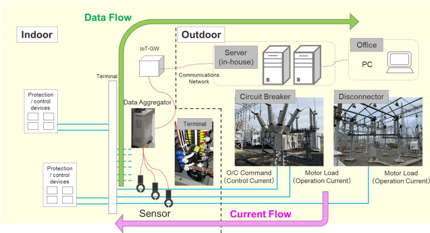
Figure 52: Layered architecture for the practical deployment of HVCB condition monitoring in a transmission network [63].
