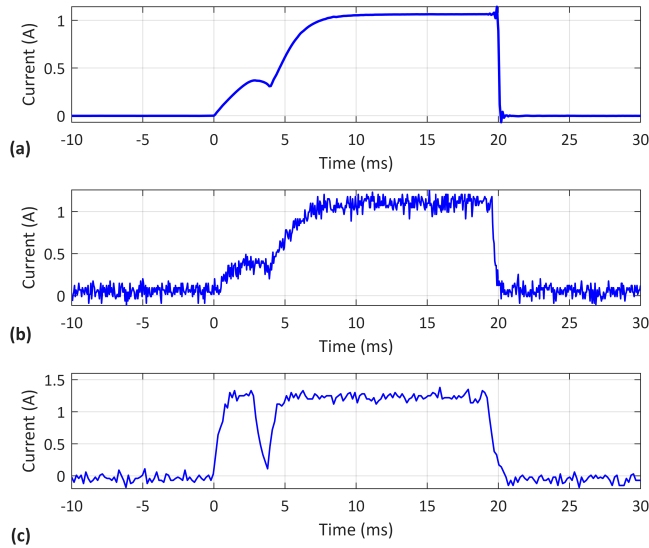
Figure 31: Trip/close coil current signal and related diagnostic features. (a) Real HVCB coil current measured with CIBANO 500. (b) Real HVCB coil current measured using Raspberry Pi. (c) Emulator circuit current measured using an inexpensive sensor.
