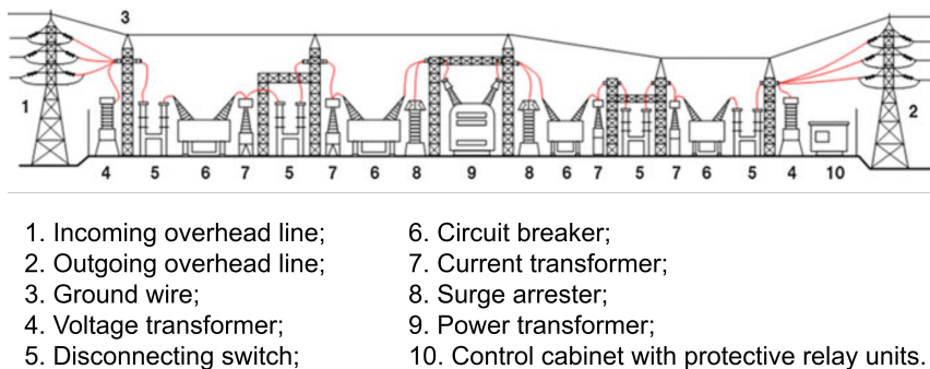
Figure 3: A typical AC substation schematics [19]
