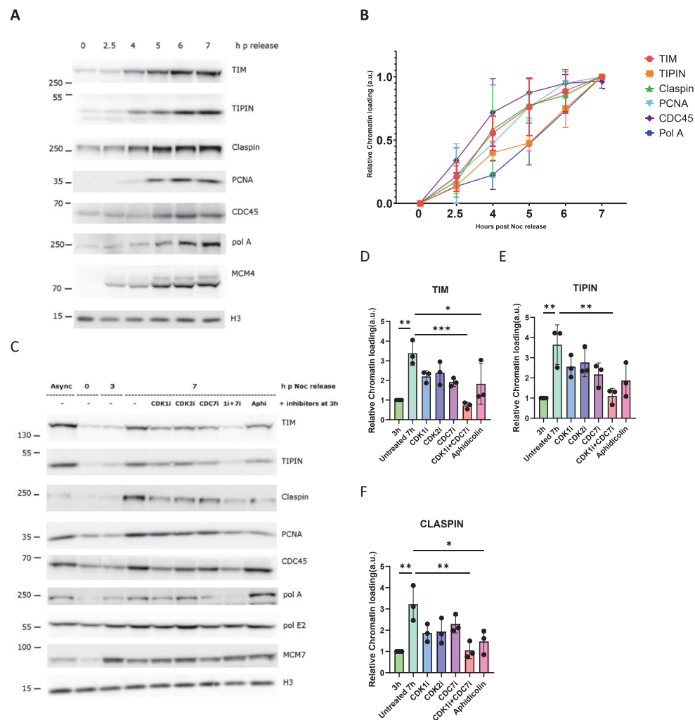
Figure 3: TIM loading to chromatin during origin firing occurs in multiple steps, is dependent on CMG assembly and on DNA synthesis
