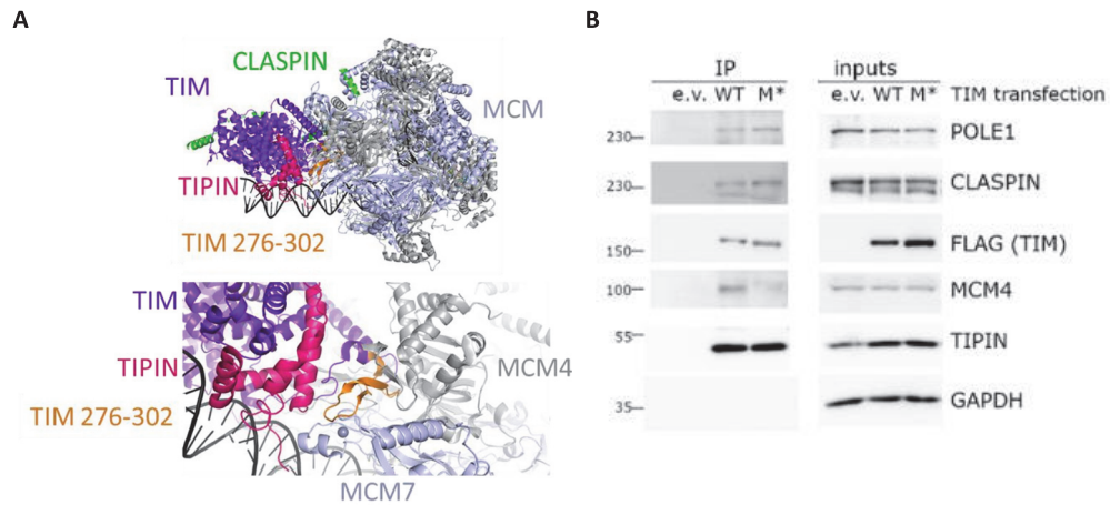
Figure 5: TIM mutant unable to interact with MCM cannot load to chromatin
