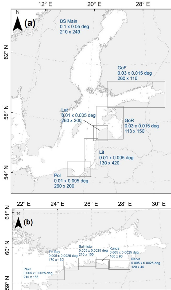
Figure 2. a) First level (BSMain, the entire Baltic Sea) and second level grids (boxes) and their spatial resolution used in various simulations with the SWAN model. See Section 1.2.1 for their description. b) Location and spatial resolution of the third level (the innermost) grids for the southern shore of the Gulf of Finland. The numbers below the name of the grid show resolution in degrees and number of grid cells in both directions. From Paper I.
