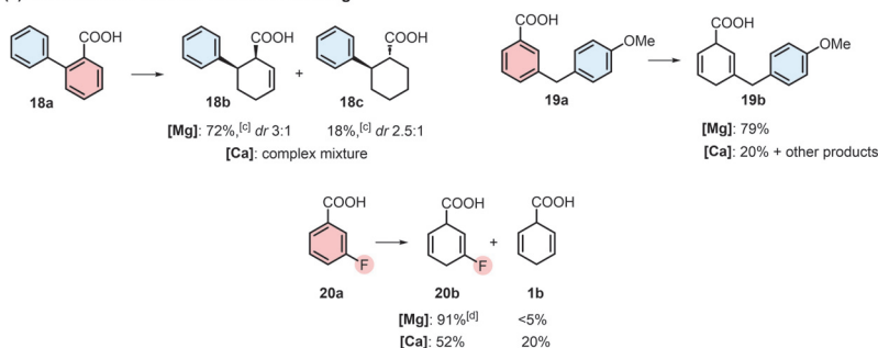
Scheme 6. Mechanochemical Birch reduction of arenes with Mg and its limitations (a), selectivity studies (b) and chemoselective Birch reductions (c). Unless stated otherwise, yields were determined by 1 H NMR with an internal standard after the hydrolytic workup (aq. HCl or aq. NH 4 Cl). See sections 7 and 8 in the Supporting Information for details. [a] Optimal conditions: Mg powder (10 equiv.), EDA (5 equiv.), THF (1 equiv.). [b] Determined by HPLC analysis of the crude reaction mixtures. 1 H NMR with an internal standard showed a similar outcome. [c] With 30 equiv. of Mg and 1.5 h of milling. Relative configuration is depicted for the major diastereomer ( cis -18b and trans -18c). [d] The product 20b was isolated by column chromatography on silica gel in 78% yield.
