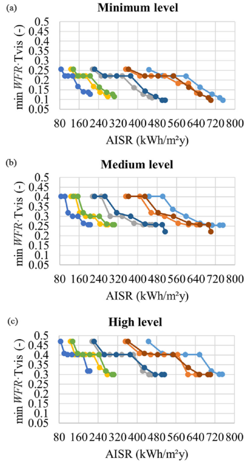
Fig. 9 Minimum recommended WFR \cdot Tvis depending on the room orientation and the accumulated AISR to achieve a minimum (a), medium (b), and high (c) level of daylight provision according to the method 2 (based on the sDA ) defined by the EN 17037:2018.
