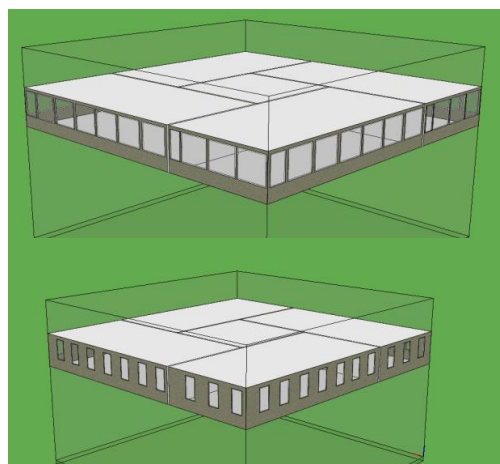
Figure 5 3d of the model with 2 different Window to Wall Ratio (WWR)
