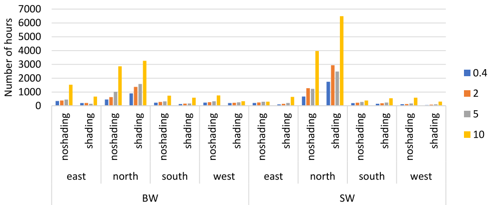
Fig. 16. The total hours when the temperature exceeded 25 °C when cooling devices were at maximum capacity in the 30 years of simulation data.
