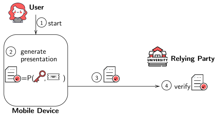
Figure 35: Anonymous credentials
