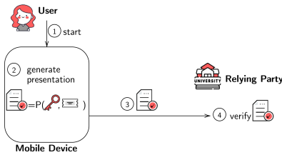
Fig. 3. Anonymous credentials
