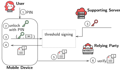
Fig. 4. Server-supported credentials
