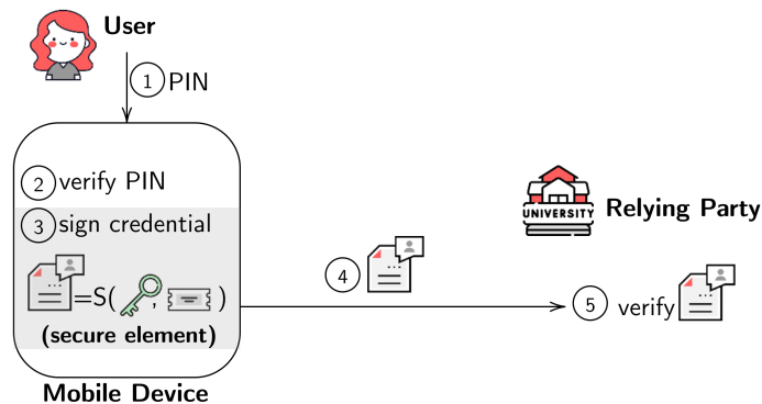
Figure 32: Hardware-based credential
