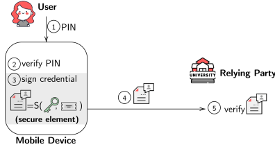
Fig. 1. Hardware-based credential
