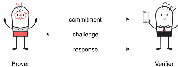
Figure 4: \Sigma -protocol message flow
