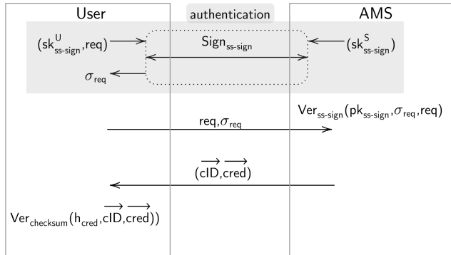
Figure 23: Prettiness get all credentials
