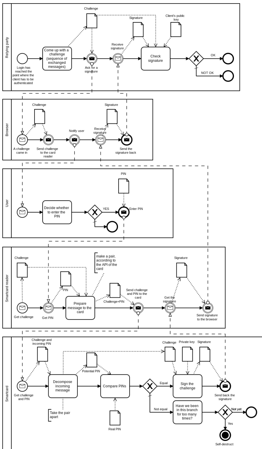
Figure 28: The smart card system
