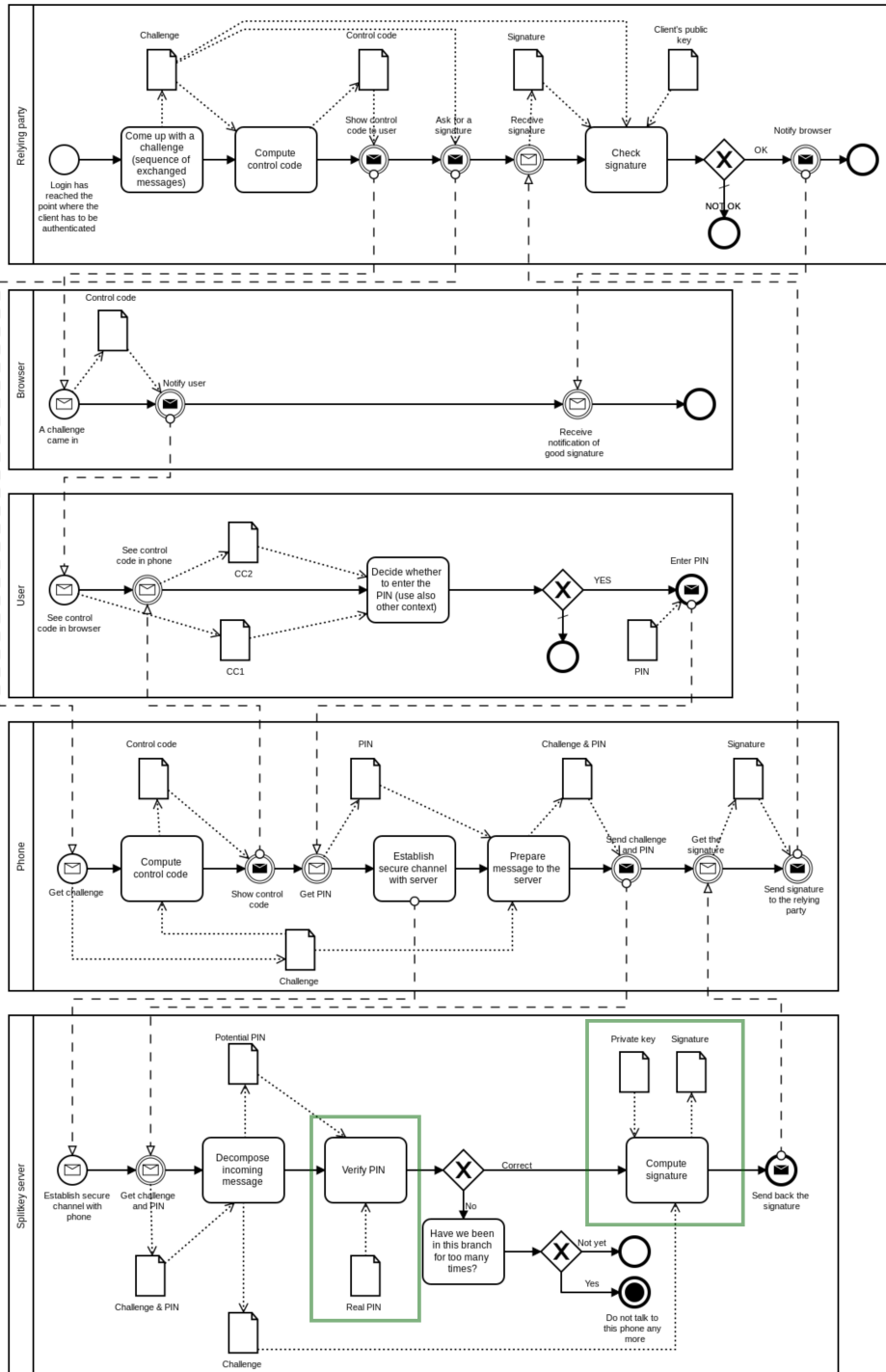
Figure 31: The second intermediate system. Highlighted in green boxes are main changes with the first intermediate system.
