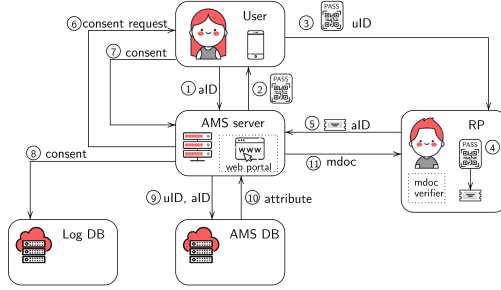
Figure 2: Presenting attributes
