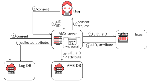
Figure 1: Issuing attributes
