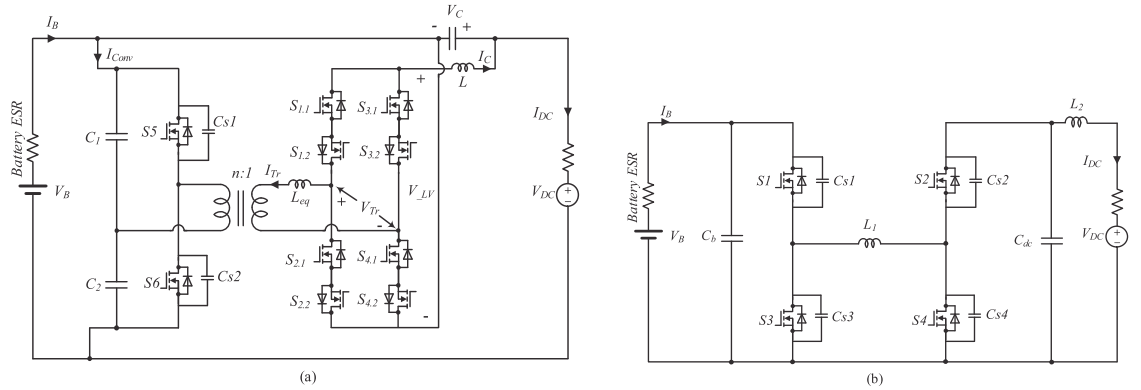
Fig. 1. Topology of CSFB S-PPC (a) and four-switch buck-boost converter (b)
