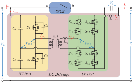
Fig. 1. Proposed bidirectional step-up/down (BDSUD) series partial power converter (S-PPC).
