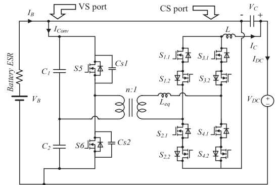
Fig. 5. Proposed S-PPC converter
