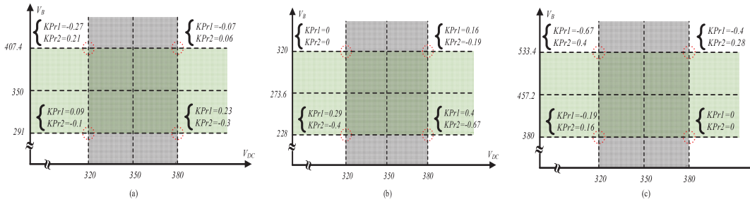
Fig. 4. Critical points based on Battery and DC-bus voltage variation for IPOS and ISOP configurations (a) Buck-Boost S-PPC (b) Boost S-PPC (c) Buck S-PPC
