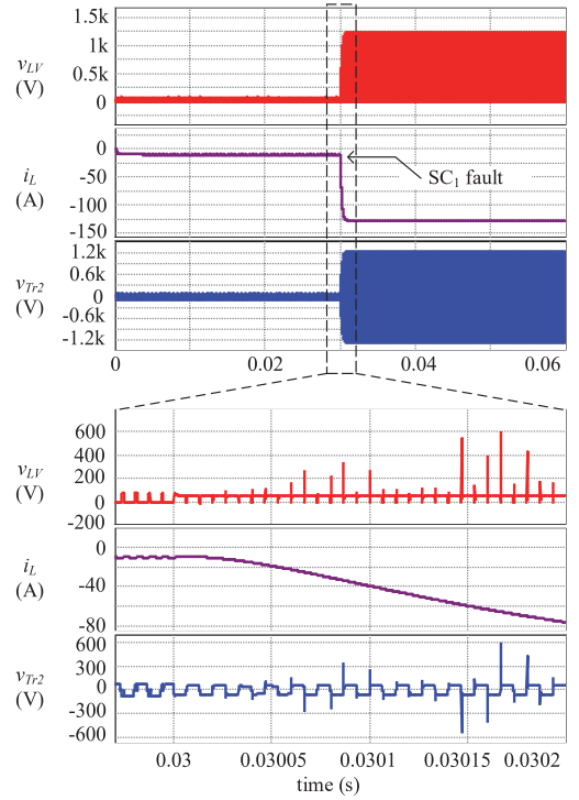
Fig. 2. Short circuit fault at input side (SC 1 ), during which the LV port voltage, inductor current, and transformer LV side voltage are shown.
