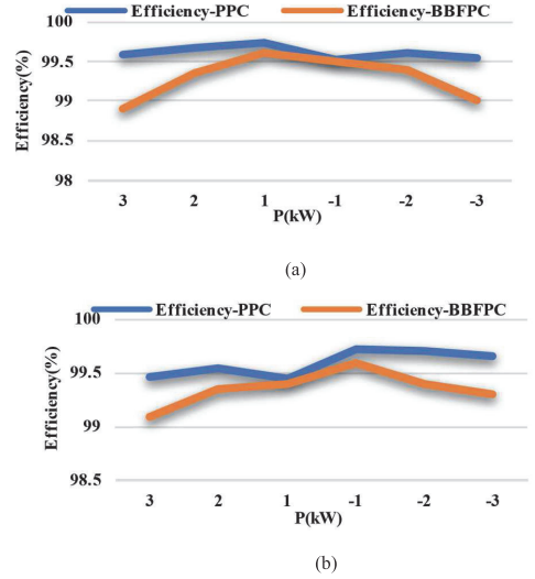
Fig. 4. The efficiency of both converters for (a) V_B=320 V and (b) V_B=380 V
