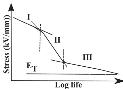
Figure 6. Representation of flat Z characteristics of insulation life in three regions adapted with permission from [44].
