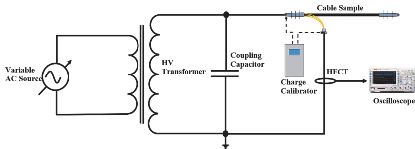
Fig. 3. Schematic of laboratory experimental setup for PD measurement.
