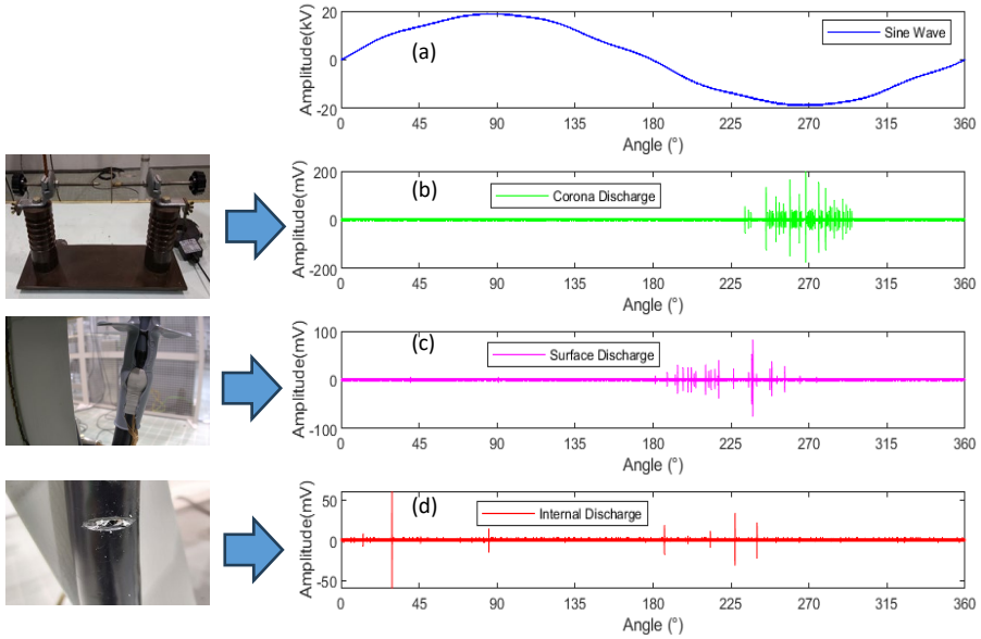
Figure 7. PRPD patterns of major types of PD sources found in power cables: a) Sine wave, b) Corona, c) Surface, d) Internal PD [Paper III].
