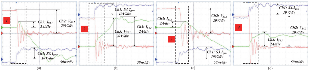
Fig. 11. Soft turn-ON of LV side switches. (a) S_{3,1} turn-ON [point 1 in Fig. 9(c)]. (b) S_{4,2} turn-ON [point 2 in Fig. 9(c)]. (c) S_{3,1} turn-ON (point 3 in Fig. 10(c)). (d) S_{4,2} turn-ON [point 4 in Fig. 10(c)].
