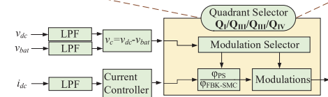
Fig. 14. Mode selection and control structure of PPC.
