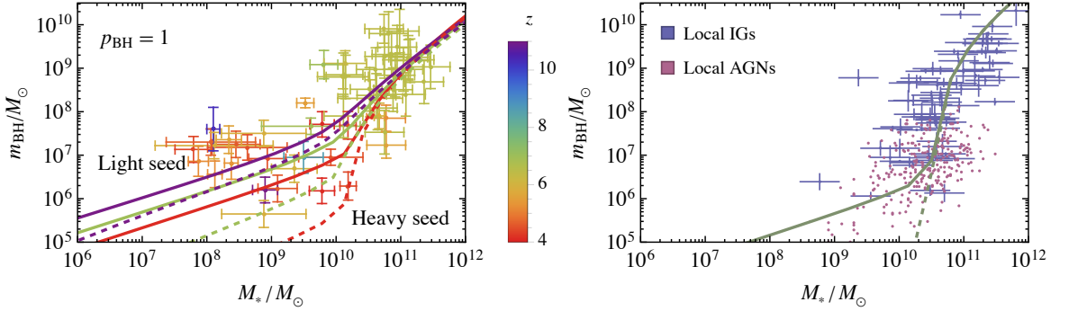
Fig. 2. Comparisons of model predictions for stellar mass-BH mass relation with high- z observations on the left and low- z observations on the right. The solid lines show the evolution of light seeds ( m_{\text{seed}} = 100 M_{\odot} with M_{\text{seed}} = 3 \times 10^4 M_{\odot} ), and dashed lines show the evolution of heavy seeds ( m_{\text{seed}} = 10^5 M_{\odot} with M_{\text{seed}} = 3 \times 10^7 M_{\odot} ), both for p_{\text{BH}} = 1 . The right panel shows the predictions of the same two models at z \approx 0 as full and dashed lines, respectively, compared to the local observations.
