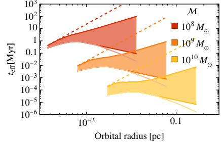
FIG. 4. Effective timescales t_{\text{eff}} for fits to the NG15 data shown as functions of the separations at which binaries are emitting GWs in the NANOGrav band (1–30 nHz), and for chirp masses \mathcal{M} \in (10^8, 10^{10}) M_{\odot} , which is the range found in [63] to dominate the stochastic GW background. The dashed lines are for energy loss by GWs alone, and the shaded regions are those favored at the 68% CL for a combination of energy loss by environmental effects and GWs. The two lower lines are computed with \alpha < 4 and \alpha < 6 as priors.
