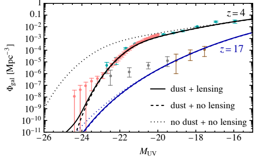
Fig. 5. UV luminosity function at z = 4 (black) and z = 17 (blue) with and without corrections due to lensing magnification and dust attenuation. The cyan and pink points show respectively the HST z = 4 data from Bouwens et al. (2021) and Harikane et al. (2022), and the brown and grey points the JWST z = 17 data from Pérez-González et al. (2025) and Castellano et al. (2025).
