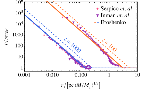
FIG. 1. The PDM minihalo profile (1) (solid lines) at redshifts z = 1000 and z = 100 compared to the estimate in Ref. [63] (dashed lines) and profiles of isolated PBHs obtained via N -body simulations [46,65] (points).
