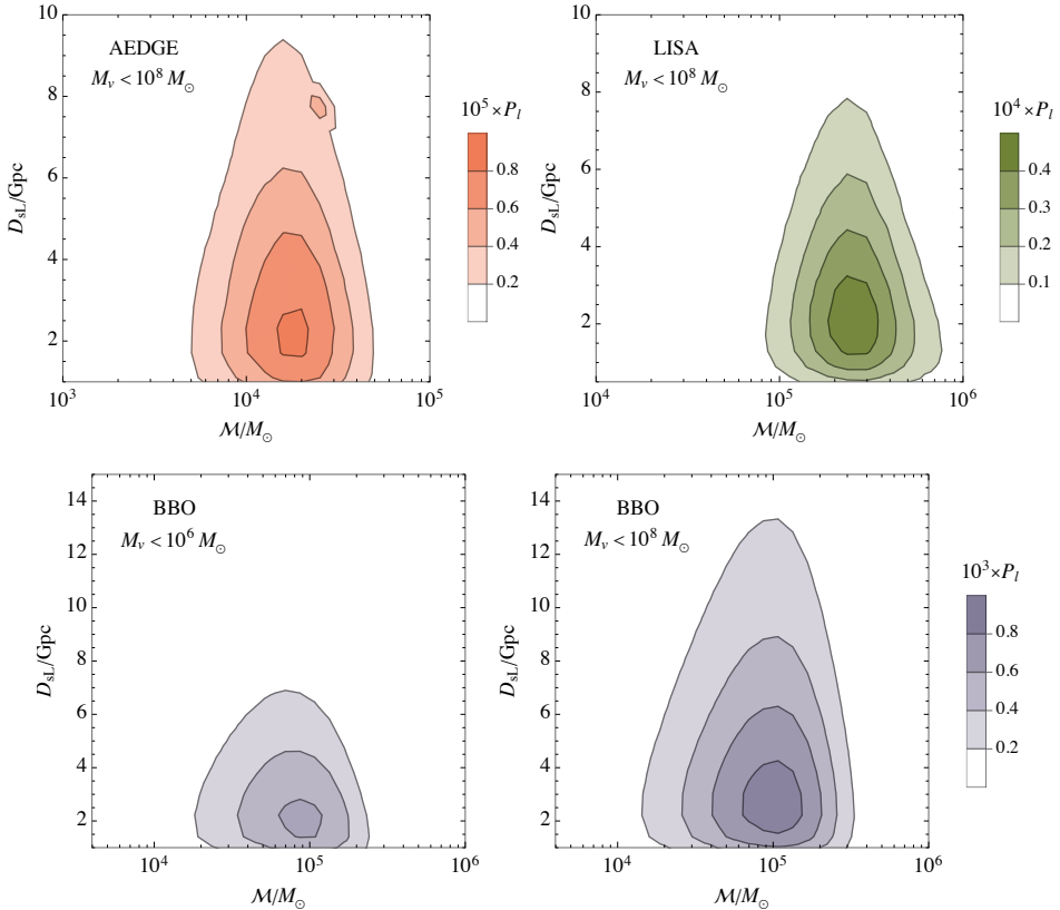
Figure 7. Probability P_l that a GW signal emitted by a binary of chirp mass \mathcal{M} and symmetric mass ratio \eta = 0.23 at distance D_{\text{sL}} is lensed by a NFW halo. The probabilities are integrated over the virial mass range shown in each panel with the CDM halo mass function.
