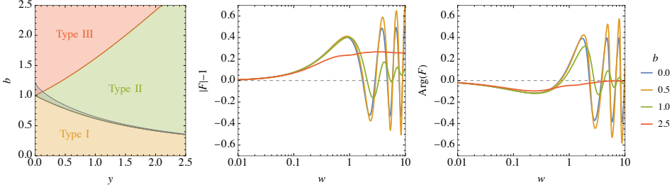
Figure 12: The left panel illustrates the three lensing regimes of a uniform sphere described in the main text. The modulus and argument of the amplification function F are shown in the middle and right panels, respectively, as a function of the dimensionless frequency w for y = 1 and various lens sizes b . The limiting case b = 0 recovers the point mass lens, while b = 0.5 , b = 1 , and b = 2.5 correspond to type I, type II, and type III lensing, respectively, as defined in the left panel. Reproduced from Paper I [61], © IOP Publishing Ltd and Sissa Medialab 2023.
