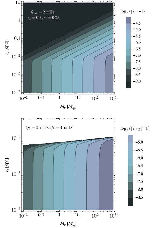
FIG. 1. Upper panel: the absolute value of the lensing amplification as a function of the halo mass and the projected distance of the source in the lens plane, for a source with f_{\text{GW}} = 2 mHz at z_s = 0.5 and a lens at z_l = 0.25 . Lower panel: the magnitude of the relative amplification factor (7) for the same source-lens configuration as in the upper panel.
