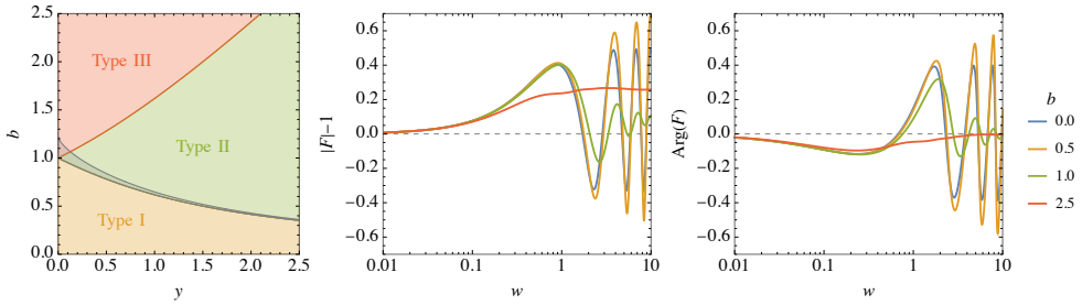
Figure 2. The left panel shows the regions corresponding to the three types of lensing by a uniform sphere discussed in the main text. The middle and right panels show the modulus and argument of the amplification function F as a function of the dimensionless frequency w for different lens sizes b and y = 1 . The b = 0 case corresponds to the point mass lens, b = 0.5 is what we refer to as type I, b = 1 as type II, and b = 2.5 as type III lensing, as shown in the left panel.
