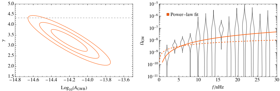
Figure 5: Left panel: Posteriors on A_{\text{GWB}} and \gamma from a fit of the power law of Eq. (76) to the NANOGrav 15-year measurements; the dashed line marks the value \gamma = 13/3 predicted for a GW-driven population of inspiralling SMBH binaries. Right panel: Best-fit power law (solid) compared with the NANOGrav 15-year measurements (violins); the dashed line shows the best fit when \gamma = 13/3 is imposed. Adapted from Paper VII [53], © 2024 American Physical Society.
