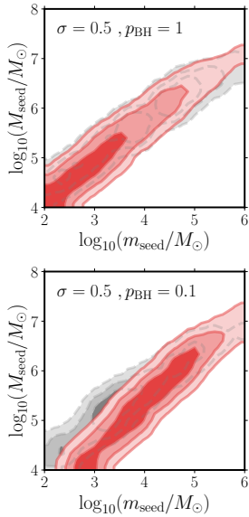
Fig. C.3. As in Fig. 4, allowing for a lognormal spread in the model predictions with \sigma = 0.5 for p_{\text{BH}} = 1 in the left panel and for p_{\text{BH}} = 0.1 in the right panel.
