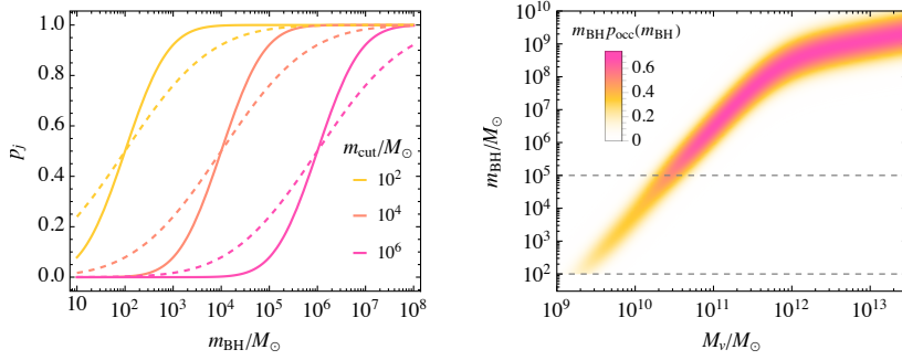
Figure 16: Left panel: The occupation probability p_j as a function of BH mass for selected values of the low-mass cut m_{\text{cut}} , with width parameters w = 1 (solid) and w = 2 (dashed). The error-function ansatz provides a smooth transition between zero and the asymptotic fraction f_j , capturing the crossover from halos too shallow to retain a seed to those hosting a fully formed BH. Right panel: The halo mass–BH mass plane, colour-coded by the occupation fraction p_{\text{occ}} for a two-component seeding model with f_1 = f_2 = 0.5 , w_1 = w_2 = 1 , m_{\text{cut},1} = 100 M_\odot , and m_{\text{cut},2} = 10^5 M_\odot . The figure illustrates how the coexistence of light and heavy seed populations gives rise to occupation in distinct regions of the M_v – m_{\text{BH}} plane. Reproduced from Paper VIII [57], © AAS 2024.
