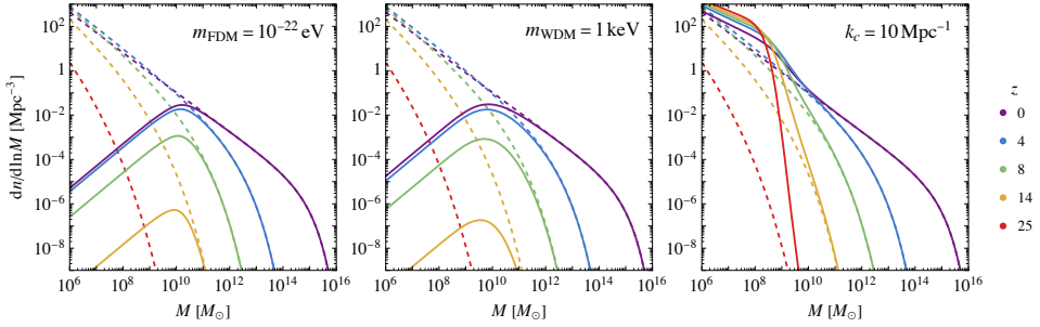
Figure 10: HMF at various redshifts z in the FDM (left) and WDM (middle) models, and in models where white noise dominates the matter perturbations at k > k_c (right). The dashed contours show the HMF in the CDM model for comparison. Reproduced from Paper V [133], © ESO 2025.
