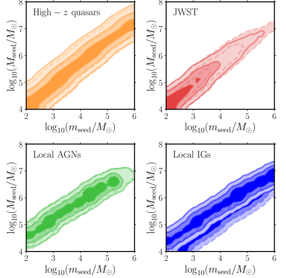
Fig. C.1. Fits to the stellar mass-BH mass data as functions of the seed BH mass m_{\text{seed}} and minimal halo mass M_{\text{seed}} where the seeds are inserted at z_{\text{seed}} = 20 , for p_{\text{BH}} = 1 without spread in the predicted relation in solid and with a log-normal spread ( \sigma = 0.5 ) in dashed.
