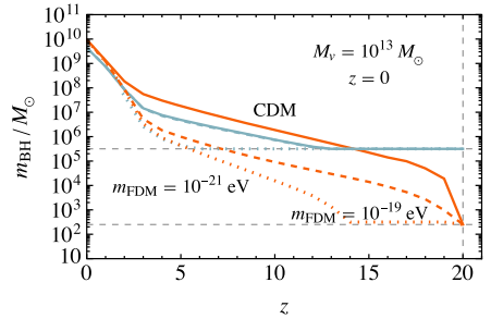
FIG. 2. Growth of individual SMBHs in both the light- and heavy-seed scenarios (orange and blue, respectively). CDM calculations are shown with solid curves and FDM with dashed ( m_{\text{FDM}} = 10^{-19} eV) and dotted ( m_{\text{FDM}} = 10^{-21} eV) curves. The host DM halo mass at z = 0 is fixed to M_v = 10^{13}M_\odot .
