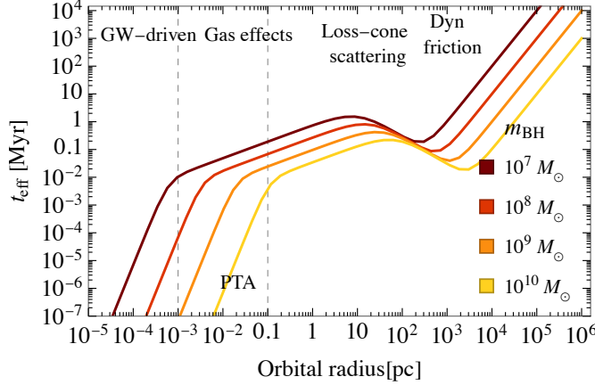
Figure 15: Effective orbital decay timescale t_{\text{eff}} of SMBH binaries of different masses as a function of the orbital separation, taking into account dynamical friction, loss-cone scattering, gas effects from a circumbinary disc and, finally, GW emission from a circular orbit. The separations at which the binaries emit GWs in the PTA band are indicated. Adapted from Paper VII [53], © 2024 American Physical Society.
