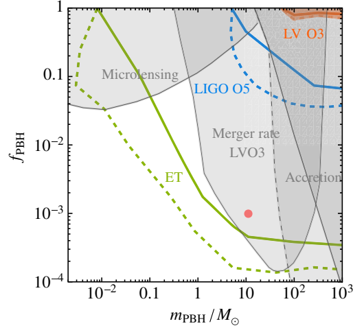
FIG. 3. The blue and green curves show the projected sensitivities of LIGO O5 and ET, and the orange curve shows the region disfavored at 1\sigma by the current (O3) LIGO-Virgo observations. The gray curves show PBH constraints from microlensing [30], merger rate measurements [17], and accretion [46]. The solid and dashed curves show the results with and without the effect of the PDM minihalo. The red dot corresponds to the scenario in which all observed BH mergers would be primordial [17–19].
