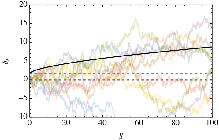
Figure 7: Random path demonstration to illustrate the EPS formalism, the dashed lines represent the spherical collapse and the moving barrier, the elliptical collapse.
