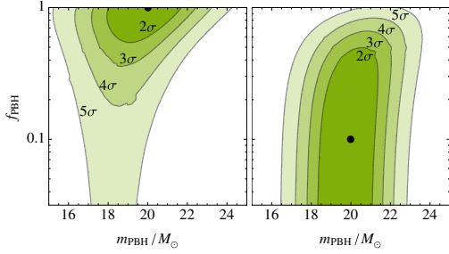
FIG. 4. Sensitivity of ET to the lens profile for two benchmark cases with \mathcal{M}_z = 40M_\odot , \eta = 0.23 , D_L = 5 Gpc, m_{\text{PBH}} = 20M_\odot , and y = 5 . The GW signal is assumed to correspond to a naked PBH lens ( f_{\text{PBH}} = 1 ) in the left panel and to a dressed lens (with f_{\text{PBH}} = 0.1 ) in the right panel. The shading shows parameter regions in which ET can distinguish the assumed waveform (black dot) from a lensed signal characterized by (m_{\text{PBH}}, f_{\text{PBH}}) at the 2\sigma – 5\sigma confidence levels.
