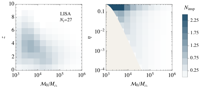
Fig. 6. Expected numbers of near-monochromatic GW signals generated more than a day before the merger that would be detectable in a year of LISA observation, as functions of the chirp mass M_0 and redshift z (left panel) and of the chirp mass and symmetric mass ratio \eta (right panel). The merger rates assume the abundance of IMBHs described by Eq. (6) for BHs heavier than 10^3 M_\odot and a universal merger efficiency factor of p_{\text{BH}} = 0.17 inferred from IPTA data, as discussed in the text.
