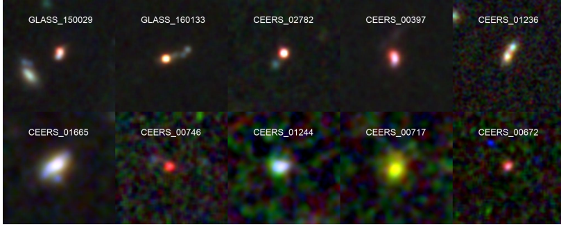
Figure 17: JWST/NIRCam images of broad-line AGNs at z = 4-7 . Reproduced from Harikane et al. [73], © AAS 2023.
