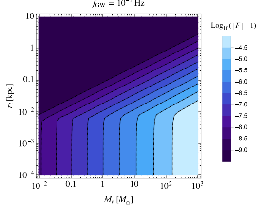
FIG. 5. Comparison between the amplification function for a single lens computed without (solid contours) and with (dashed contours) the expansion in \omega \psi_j .
