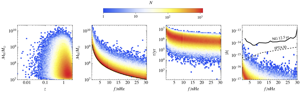
Fig. 3. Distributions of the binary parameters for a sampling of the BH binary population with 0 < z < 3 , 1 \text{ nHz} < f < 30 \text{ nHz} and M_0 > 10^9 (f/\text{nHz})^{-3} . The symmetric mass ratio is integrated with the lower bound \eta > 0.001 . In the right panel, the black curve shows the NANOGrav 95% CL constraint on continuous GW sources (Arzoumanian et al. 2023) and the projected sensitivity of IPTA30 at SNR = 8.
