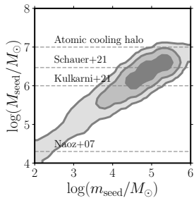
Fig. C.4. Comparison of our best fit to all the data, with p_{\text{BH}} = 0.1 , with respect to different values from simulations on M_{\text{seed}} (Schauer et al. 2021; Kulkarni et al. 2021; Naoz & Barkana 2007), as well as the atomic cooling halo estimation at z = 20 . The implications of the fit for the viability of posteriors in astrophysical terms are discussed in Sec. C.
