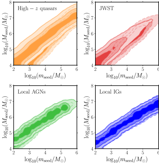
Fig. 3. Fits to stellar mass-BH mass data as functions of seed BH mass m_{\text{seed}} and minimal halo mass, M_{\text{seed}} , where the seeds are inserted at z_{\text{seed}} = 20 with p_{\text{BH}} = 1 in solid and p_{\text{BH}} = 0.1 in dashed. The contours indicate the 68%, 95%, and 99% credible regions. Upper left: High- z quasar data compiled by Izumi et al. (2021). Upper right: High- z observations with JWST (Übler et al. 2023; Larson et al. 2023; Harikane et al. 2023a; Bogdan et al. 2024; Ding et al. 2023; Maiolino et al. 2024; Yue et al. 2024). Lower left: Low- z AGNs as compiled by Reines & Volonteri (2015). Lower right: Low- z IGs from Reines & Volonteri (2015).
