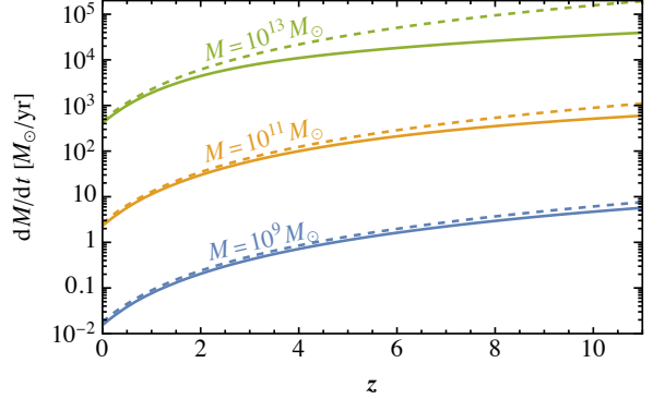
Fig. A.1. Calculations of the growth rates of DM halos. The solid curves are obtained using Eq. (A.8) and used in our analysis. The dashed curves show for comparison the estimates derived in Correa et al. (2015), which are based on finding the average mass of the main progenitor.
