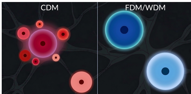
Figure 19: In this sketch, we illustrate the difference in growth through mergers in CDM versus DM models for which there is suppressed small-scale structure like in FDM or WDM.
