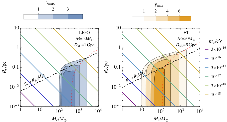
Figure 5. The color shading shows the maximum value of the impact parameter y_{\text{max}} that allows for detection of the lens effect by a uniform density sphere of mass M_c and radius R_c . The binary chirp mass and luminosity distance are fixed as shown in the plot, the symmetric mass ratio of the binary is fixed to \eta = 0.23 and the lens distance to D_{\text{LL}} = 0.5D_{\text{sL}} . The lines show the M_c - R_c relation for DM core for different axion masses m_a , following eq. (3.6). Right from the red dashed curve y_{\text{max}} is set by the interference condition, and the black dashed curve shows the point mass Einstein radius, R_c = R_E(M) .
