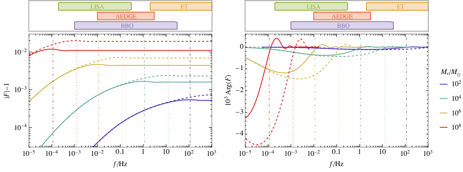
Figure 13: The modulus and argument of the amplification function F for an NFW halo lens are shown as a function of frequency for various halo virial masses. Solid and dashed curves correspond to y = 1 and y = 0.3 , respectively, with source and lens luminosity distances fixed to D_{\text{sL}} = 5 Gpc and D_{\text{IL}} = 2.5 Gpc. Vertical lines mark the frequency at which |F| is maximised. The frequency bands relevant to different experiments are indicated for reference. Reproduced from Paper I [61], © IOP Publishing Ltd and Sissa Medialab 2023.
