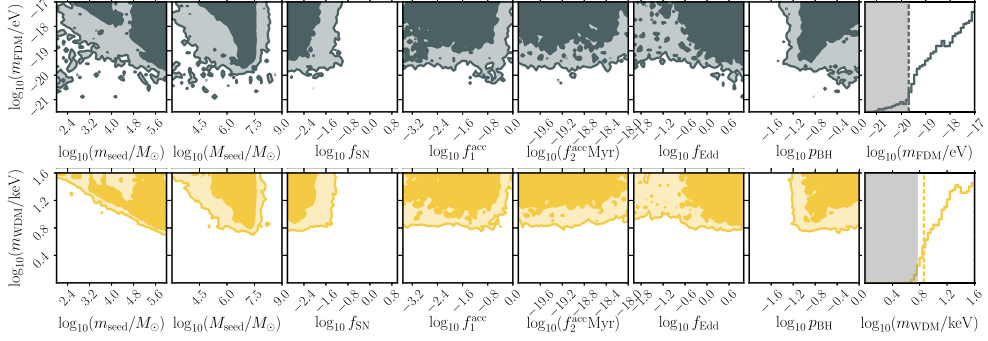
FIG. 3. Posteriors of the stellar-BH mass fit parameters as functions of the FDM mass (upper panels) and WDM mass (lower panels). The vertical dashed lines are our 95% CL lower bounds on these masses. The gray band in the \log_{10}(m_{\text{FDM}}/\text{eV}) posterior shows the most stringent 95%CL exclusion of m_{\text{FDM}} from a Lyman- \alpha analysis [77], namely < 2 \times 10^{-20} eV, and the gray band in the \log_{10}(m_{\text{WDM}}/\text{keV}) posterior shows the most stringent 95%CL exclusion of m_{\text{WDM}} from a joint analysis of strong gravitational lensing, the Lyman- \alpha forest, and Milky Way satellites [78], namely < 6.0 keV. The full corner plots are shown in Supplemental Material [56].
