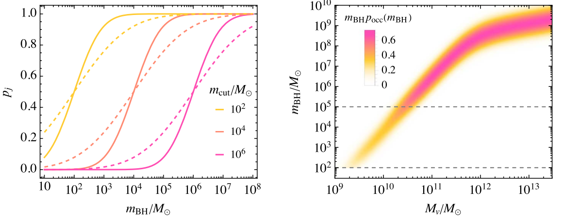
Figure 1. Left panel: the low-mass cut on the massive BH population for different values of m_{\text{cut}} , for w = 1 (solid) and w = 2 (dashed). Right panel: the halo mass–BH mass relation. The color coding shows the BH occupation fraction p_{\text{occ}} as a function of the halo mass M_v and the BH mass m_{\text{BH}} for a scenario with f_1 = f_2 = 0.5 , w_1 = w_2 = 1 , m_{\text{cut},1} = 100 M_\odot , and m_{\text{cut},2} = 10^5 M_\odot .
