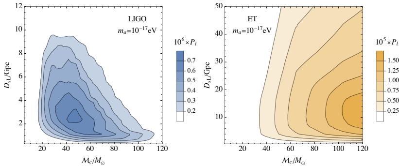
Figure 10. Probability to detect the lensing by fuzzy DM cores for m_a = 10^{-17} eV as a function of the source parameters.
