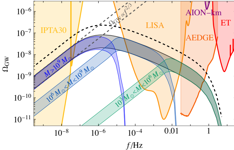
Figure 6: The GW energy density spectrum \Omega_{\text{GW}} as a function of frequency for merging SMBHs of different mass ranges (coloured bands), compared with the design sensitivity curves of a representative set of current and future GW observatories. Reproduced from Paper VI [54], © ESO 2023.
