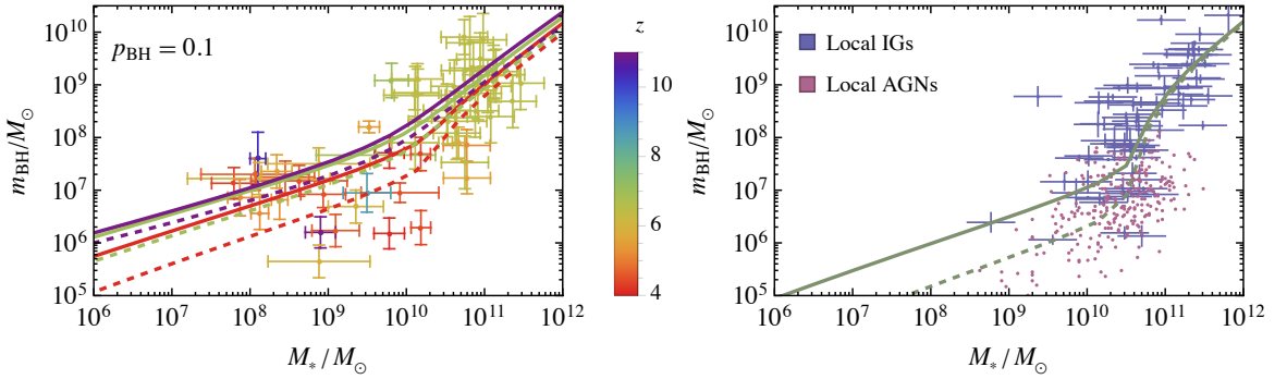
Fig. 5. Comparisons of model predictions for stellar mass-BH mass relation with high- z observations on the left and with low- z observations on the right. The solid lines show the best fit for p_{\text{BH}} = 0.1 to the JWST data, and the dashed lines show the best fit to the rest of the SMBH data. The best-fit parameter values are given in Table 1.
