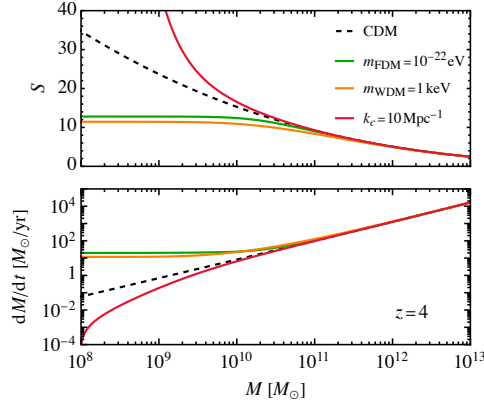
Figure 9: Variance S = \sigma^2 of matter perturbations (upper panel) and halo growth rate (lower panel) in the models considered in this work: CDM (dashed black line), FDM (green line), WDM (orange line), and an enhanced matter power spectrum (red line). Reproduced from Paper V [133], © ESO 2025.
