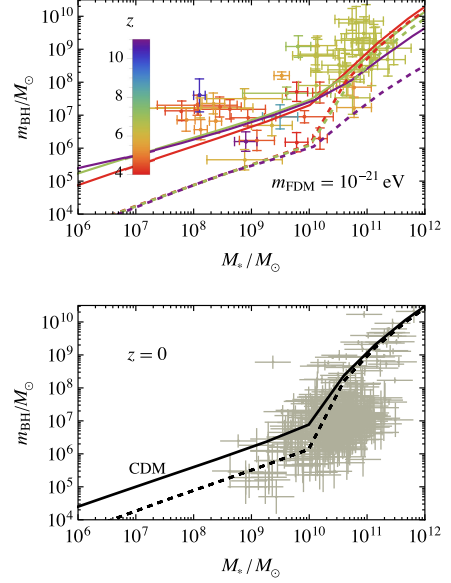
FIG. 1. Stellar-BH mass relation in a heavy-seed scenario. Solid lines show the CDM results and dashed lines the FDM result with m_{\text{FDM}} = 10^{-21} eV. The different colors in the top panel represent the different redshifts, while the lower panel represents the local universe.
