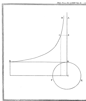
Figure 1: First sketch of the orbits around a “dark star”, the precursor of the BH concept. Reproduced from Michell (1784) [99], Philosophical Transactions of the Royal Society ; public domain.
