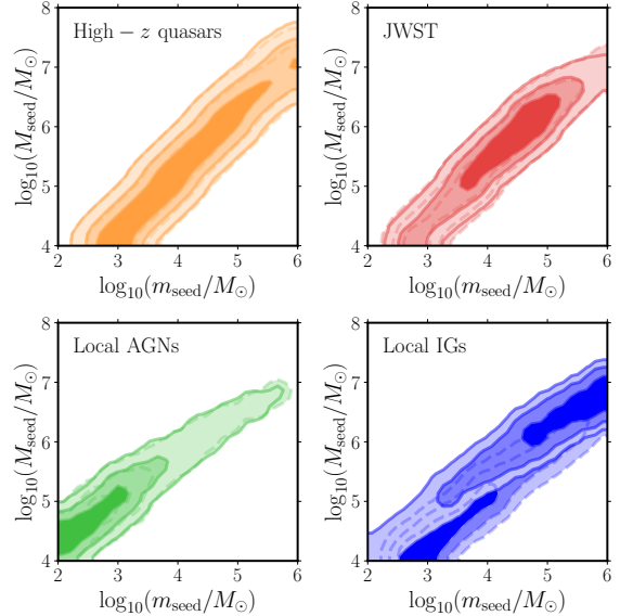
Fig. C.2. As in Fig. C.1 for p_{\text{BH}} = 0.1 .
