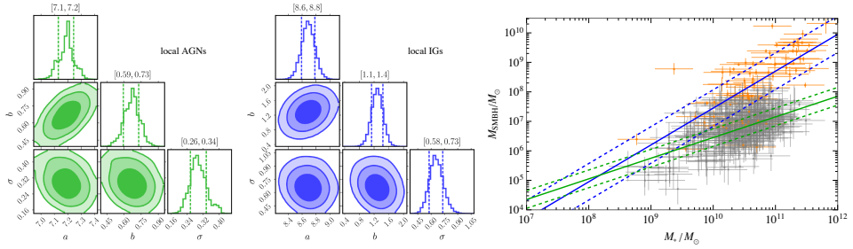
Figure 14: The left panel shows the posteriors of the fit of Eq. (188) to the local AGNs of Ref. [118], and the central panel the posteriors of the fit to the local dynamically measured SMBHs in inactive galaxies (IGs) [86]. In the right panel we show in orange the dynamically measured SMBHs and in grey the local AGNs, compared with their respective fits. Adapted from Paper IX [55], © ESO 2024.
