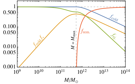
Fig. 1. Baryon fractions as functions of DM halo mass M . f_{\text{ej}} is the cold gas fraction that is ejected from the halo by SNe, f_{\text{cold}} is the fraction of the remaining gas that is cold, f_{\text{rem}} is the fraction of gas available for accretion, and f_* is the fraction of cold gas that is used for star formation.
