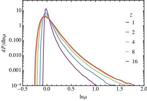
Fig. 4. Distributions of lensing magnifications at different source redshifts.
