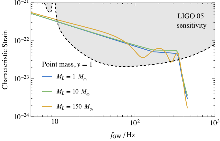
Figure 11: Illustrative example on the same binary as in Fig.4, but now lensed by point masses of different masses at impact parameter y = 1 . We can see how the lens produces a diffractive increase in the amplitude, a wave optics oscillation and finally the geometric optics interference between paths, the case of a 1 M_\odot lens is indistinguishable by eye from the unlensed waveform.
