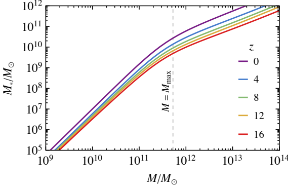
Fig. B.1. The evolution of the halo mass-stellar mass relation given by the star formation rate (B.5), the EPS estimate for the halo growth (A.8) and the growth of stellar masses by mergers (B.3).
