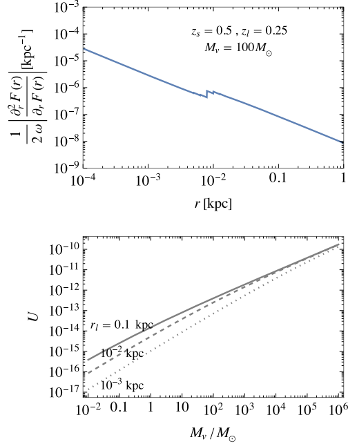
FIG. 4. Upper panel: comparison of the second and first derivatives of F . Lower panel: values of U for the typical impact parameters that contribute to the dark timbre.
