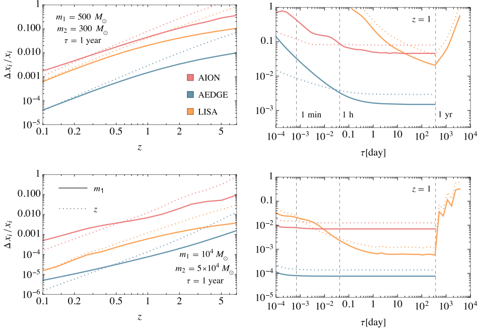
Figure 3. Measurement accuracies for the binary parameters: the upper and lower panels correspond to two binaries whose component masses are fixed. In the left panels, the binary is observed for the last 1 yr and the errors are shown as a function of its redshift. In the right panels, z = 1 and the errors are shown as a function of the binary coalescence time at the beginning of a 1 yr observation. The errors for the masses of both BHs are almost the same.
