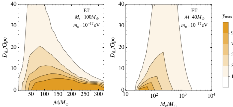
Figure 6. Maximum value of the impact parameter y_{\max} for which ET can detect microlensing by a fuzzy DM core for the DM mass m_a = 10^{-17}\text{eV} as a function of the luminosity distance and the binary chirp mass (left panel) or the core mass (right panel).
