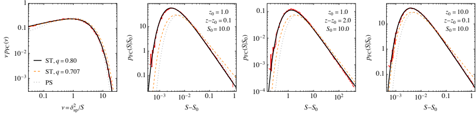
Figure 8: Left panel: Unconditional first-crossing distribution v p_{\text{FC}}(v) for the spherical (PS) and ellipsoidal (SMT) barriers. Other panels: Conditional first-crossing distributions p_{\text{FC}}(S|S_0) for random walks starting at S_0 = 10 , for different values of z_0 and z - z_0 . The red histograms are Monte Carlo random walks; the black solid, orange dashed and grey dotted lines are the ellipsoidal-collapse estimates with q = 0.80 and q = 0.707 and the spherical-collapse (PS) result, respectively. Reproduced from Paper V [133], © ESO 2025.
