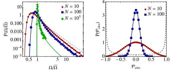
Fig. A.1. Distributions of the total signal strengths from 1, 10, 100, and 10^5 sources whose independent signal strengths have identical \Omega^{-\frac{5}{2}} tails (left). Distribution of \mathcal{P}_{\text{circ}} for 1, 10 and 100 identical sources (right). The dashed line shows the distribution from a single source, the solid lines show the analytic estimates, and the distributions obtained from an explicit Monte Carlo analysis are shown by the points.
