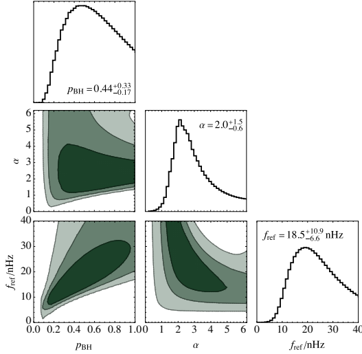
FIG. 3. Fit of the SMBH binary model with environmental effects parametrized by f_{\text{ref}} , \alpha , and p_{\text{BH}} to the NG15 data [5], for \beta = 2/5 .
