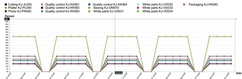
Figure 5. Time-series analysis of workstation OEE based on one-month virtual factory simulation data. The results serve as input for subsequent clustering analysis.
