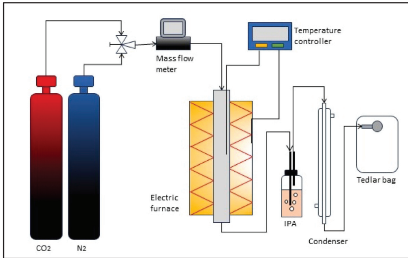
Fig. 1. Schematics of the used fixed-bed reactor.
