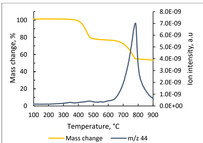
Figure 6. TGA–MS analysis of the same OS under N_2 atmosphere, showing mass change and CO_2 evolution ( m/z = 44 ). The data are obtained from a repeat experiment performed under the same conditions as in Paper I
