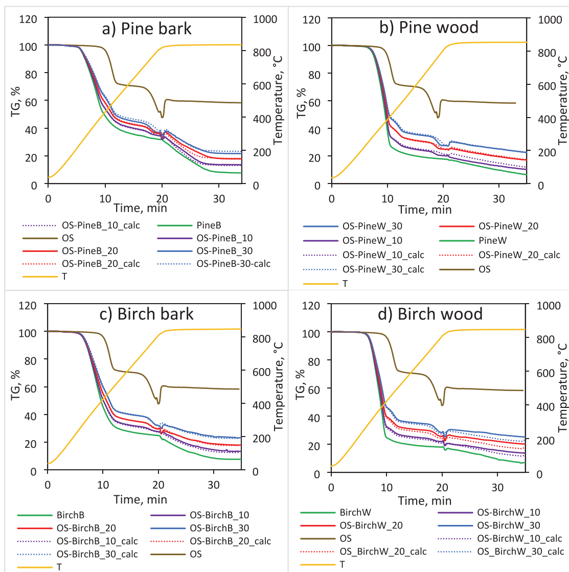
Fig. 4. Comparison of experiment and calculated values of TGA.
