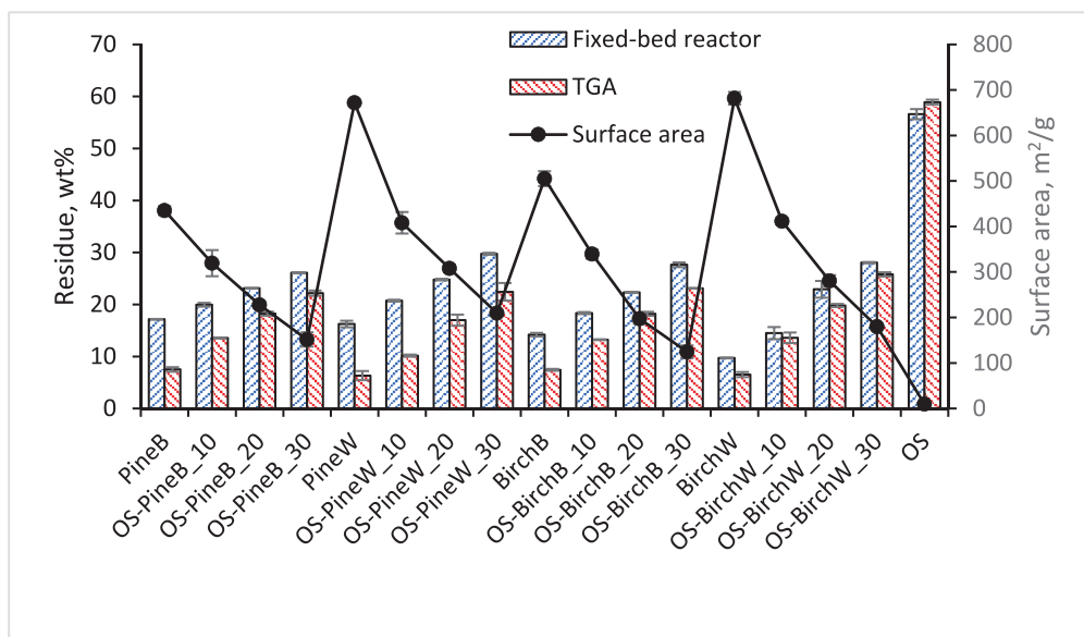
Fig. 2. Mass residues of gasification experiments in TGA and fixed-bed reactor and surface areas of char blends.
