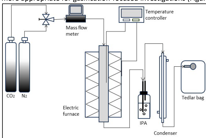
Figure 2. Schematic of the fixed-bed reactor (Paper III)
