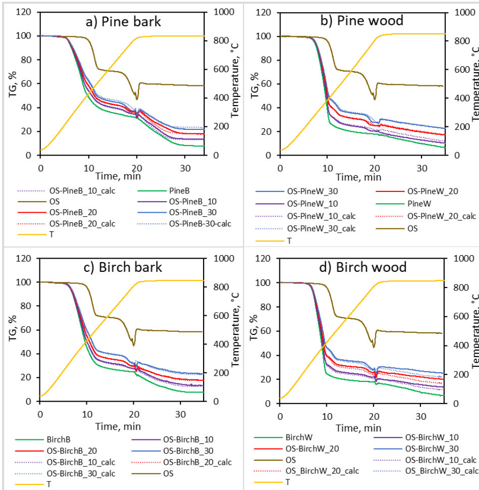
Figure 8. Comparison of experimental and calculated curves of TGA (Paper III)
