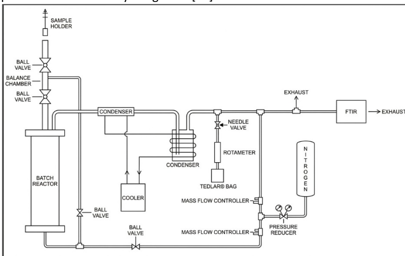
Figure 1. Schematic of the drop-in batch reactor (Paper I)
