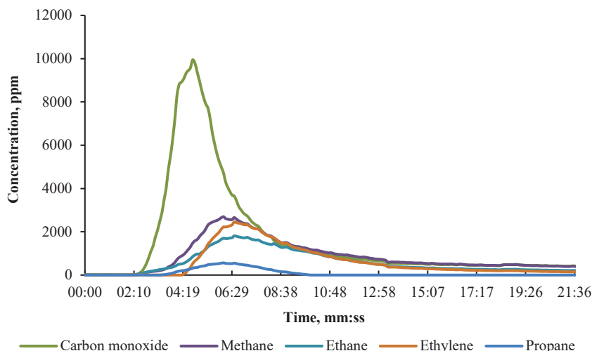
Fig. 4. Evolution of different gases during oil shale and biomass co-pyrolysis at 550 °C in the fixed bed reactor.
