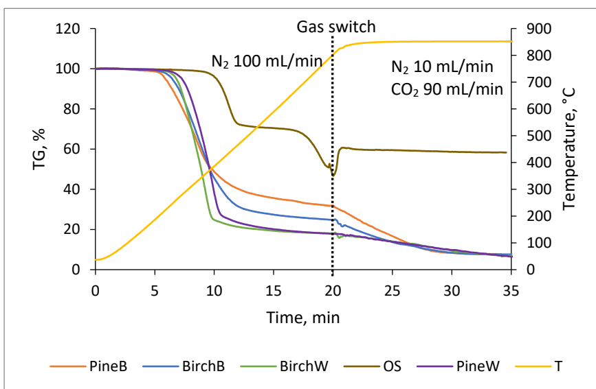
Figure 5. Mass loss curves of natural feedstocks (Paper III)
