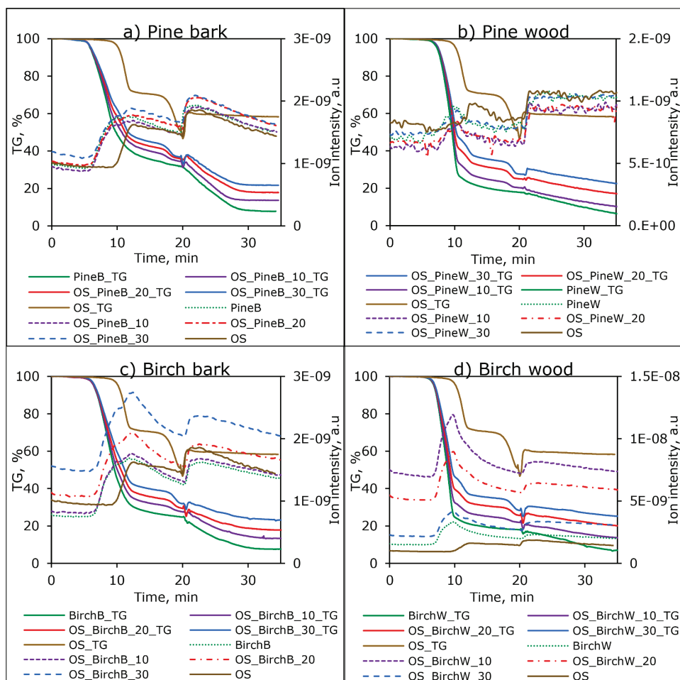
Fig. 5. Mass loss curves with the simultaneous evaporation of m/z 2 indicating the evaporation of H_2 in different BM blends.
