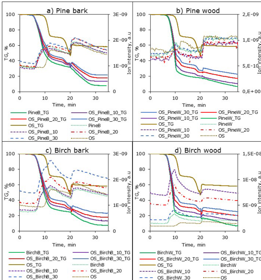
Figure 9. Mass loss curves with the simultaneous evaporation of m/z = 2 indicating evaporation of H_2 (Paper III)
