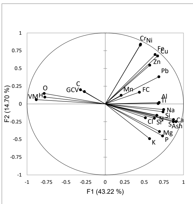
Figure 4. PCA loading plot showing the relationships between BM properties and elemental composition variables (Paper II); VM, volatile matter; H, hydrogen; O, oxygen; GCV, gross calorific value; C, carbon; FC, fixed carbon
