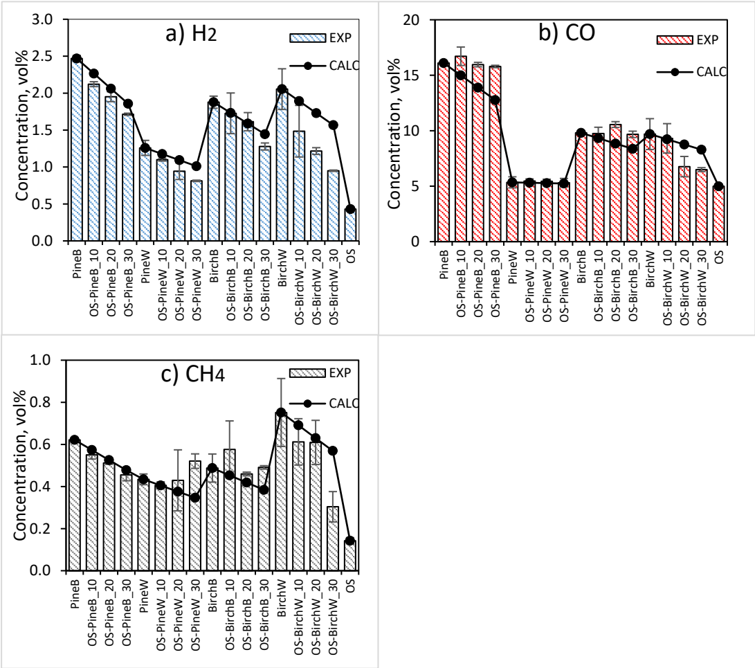
Figure 10. Gas concentrations and corresponding calculated values during gasification (Paper III)
