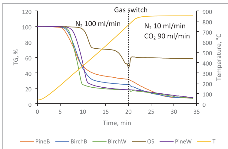
Fig. 3. Mass loss curves of natural feedstocks.
