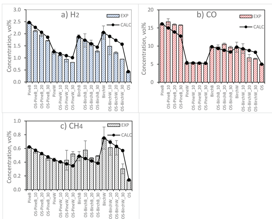
Fig. 6. Comparison of experimental and theoretical H_2 , CO and CH_4 concentrations.
