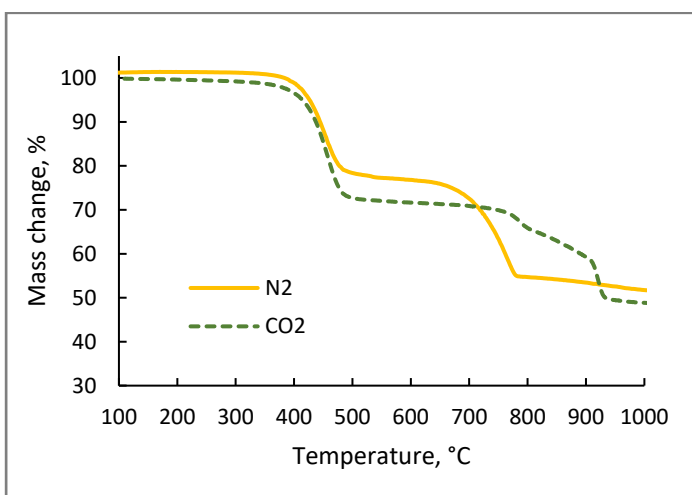
Figure 7. OS decomposition in N_2 and CO_2 atmospheres [95]
