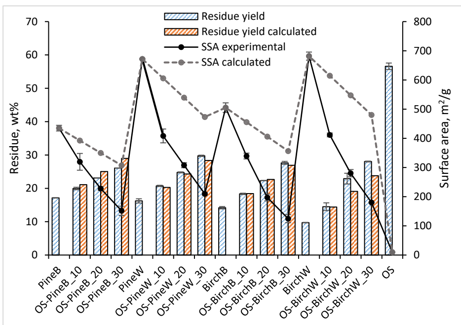
Figure 11. Solid residue yield and BET surface area of OS and BM blends obtained in the fixed-bed reactor (experimental data from Paper III; calculated SSA values and residue yields added for comparison)
