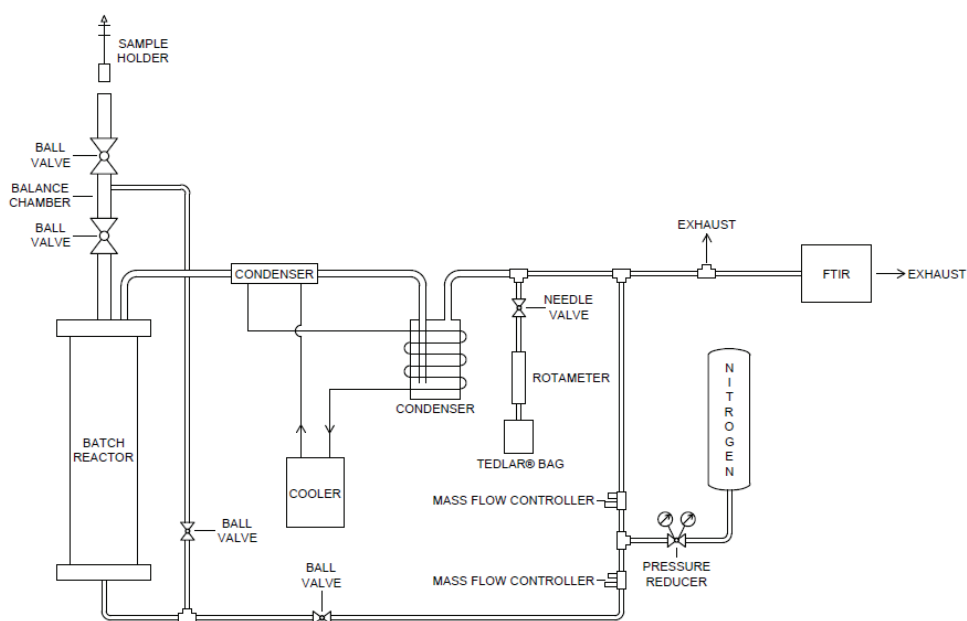
Fig. 1. Fixed bed reactor set-up.
