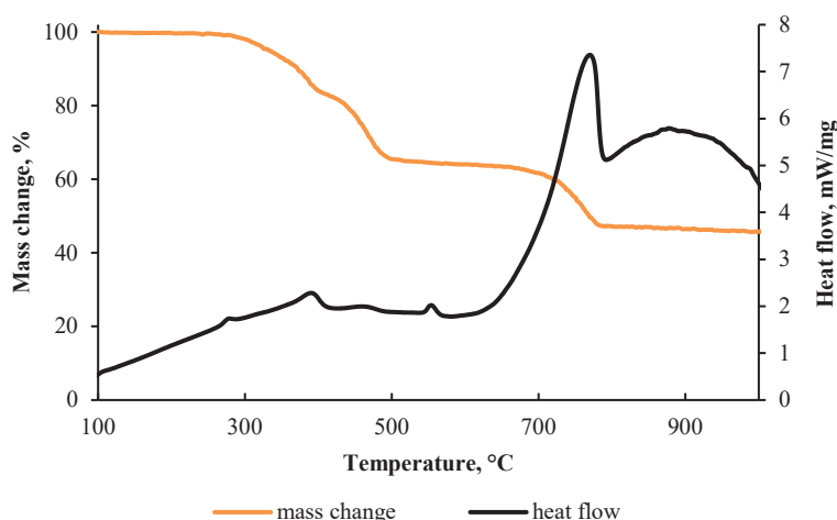
Fig. 3. Decomposition of oil shale and biomass mixture (80:20 w:w) in \text{N}_2 atmosphere.
