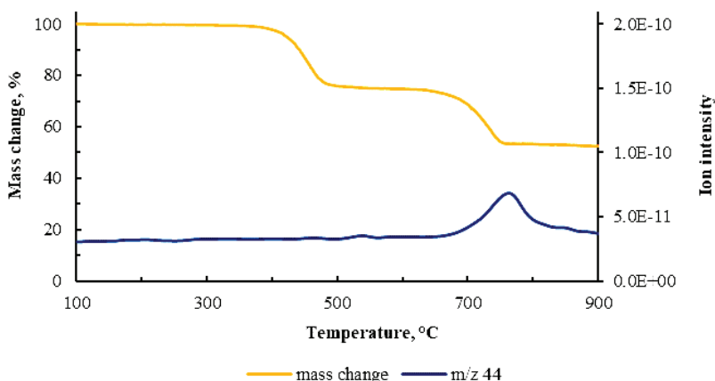
Fig. 2. Decomposition of oil shale and evolution of CO_2 in N_2 atmosphere.
