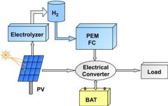
Figure 10: A stand-alone system configuration for house energy [44].
