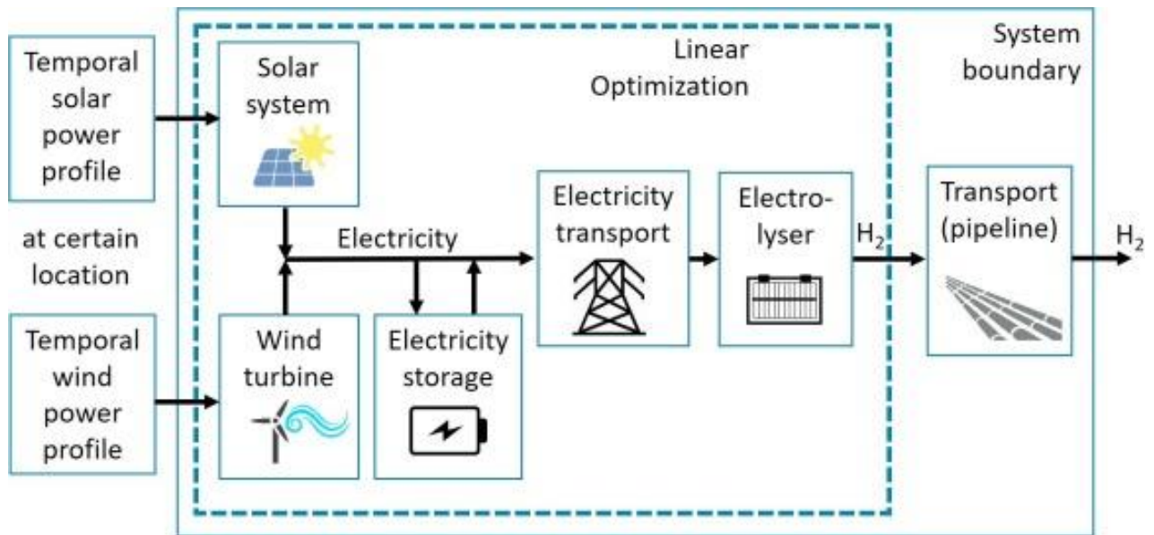
Figure 12: Hydrogen production from renewables and pipeline distribution between North Africa and Central Europe [59].
