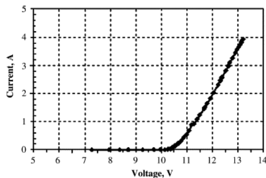
Figure 8: I-V characteristic of 50 W PEM electrolyzer [43].
