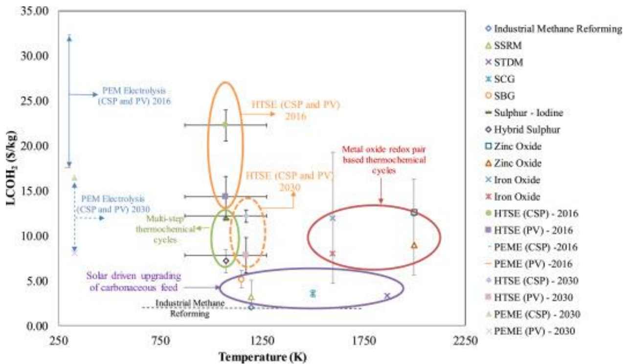
Figure 13: Economic chart for solar processed hydrogen methods [60].
