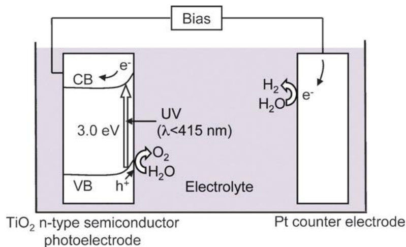
Figure 6: Water electrolysis using \text{TiO}_2 photoelectrode [40].
