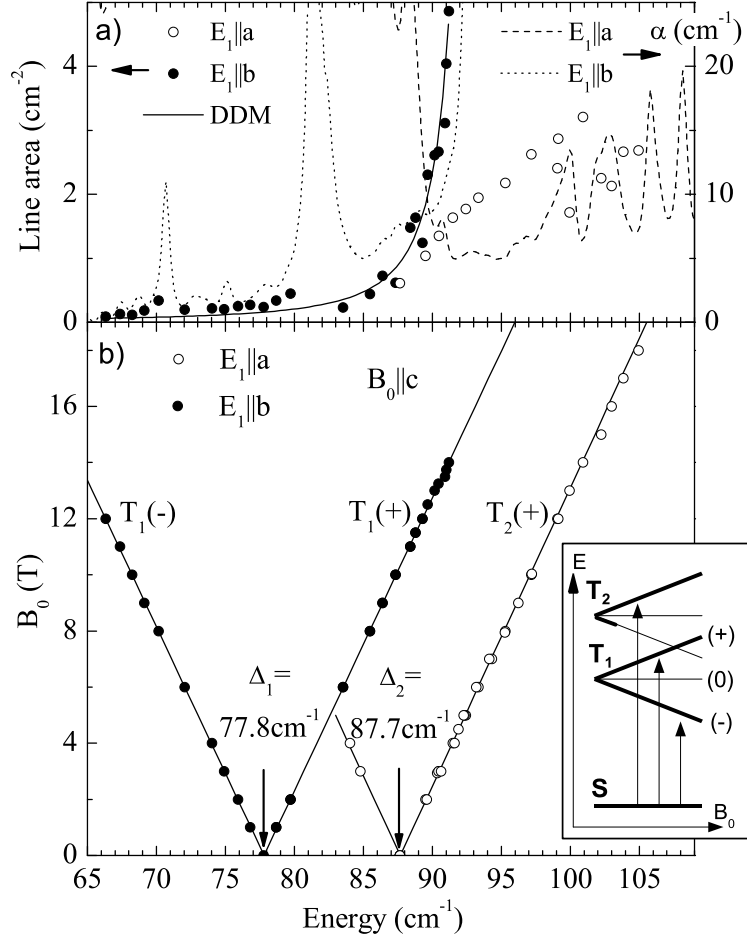
Figure 4.6: Magnetic field \mathbf{B}_0 \parallel \mathbf{c} dependence of line areas and positions. a) Line areas of triplet modes (left axis) and FIR absorption spectra (right axis) at temperature 4.4K for \mathbf{E}_1 \parallel \mathbf{a} and \mathbf{E}_1 \parallel \mathbf{b} polarizations. The solid line is the dynamic Dzyaloshinskii-Moriya interaction model fit of the T_1 absorption line area. b) T_1 and T_2 line positions as a function of magnetic field B_0 . The inset shows schematically the observed transitions.
