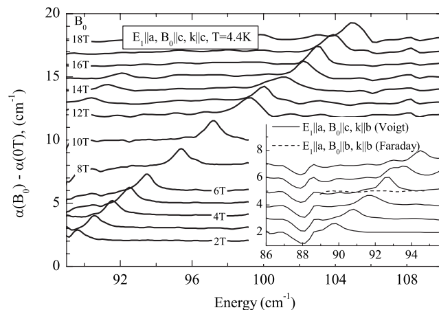
FIG. 2. Differential absorption spectra of triplet T_2 in magnetic field applied in the c axis direction with light \mathbf{k} vector \mathbf{k} \parallel \mathbf{c} and polarization \mathbf{E}_1 \parallel \mathbf{a} at 4.4 K measured using the ab -plane crystal. The spectra are offset in vertical direction by magnetic field value B_0 . The inset shows differential absorption spectra for the ac -plane crystal in Faraday (dashed line) and Voigt (solid line) configurations. Triplet T_2(+) is not infrared active when \mathbf{B}_0 \parallel \mathbf{b} , as shown by the dashed line for an arbitrary chosen B_0 = 5\text{ T} .
