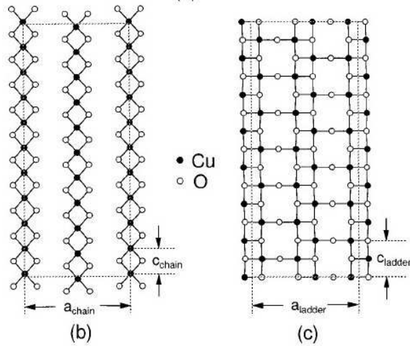
Figure 4.1: The crystal structure of \text{Sr}_{14}\text{Cu}_{24}\text{O}_{41} : a) alternating chain and ladder layers, b) \text{CuO}_2 chain layer structure, c) \text{Cu}_2\text{O}_3 ladder layer structure
