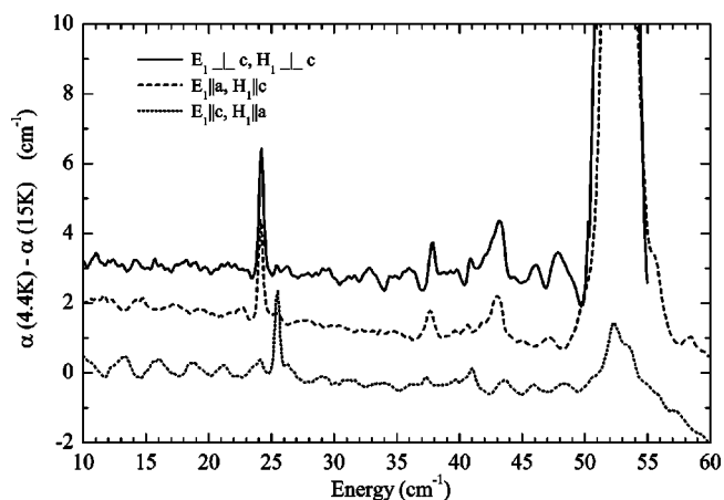
FIG. 2. Differential absorption in \mathbf{E}_1 \perp c (two upper curves) and \mathbf{E}_1 \parallel c (lower curve) polarization. Spectra have been offset in the vertical direction.
