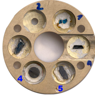
Figure 4.3: Sample wheel of the TeslaFIR spectrometer transmission probe. Positions No. 4 and 5 contain ( ab )-plane and ( ac )-plane \text{Sr}_{14}\text{Cu}_{24}\text{O}_{41} crystals respectively
