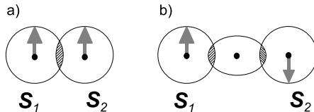
Figure 2.1: Exchange interactions: a) direct exchange interaction b) superexchange interaction via nonmagnetic ligand
