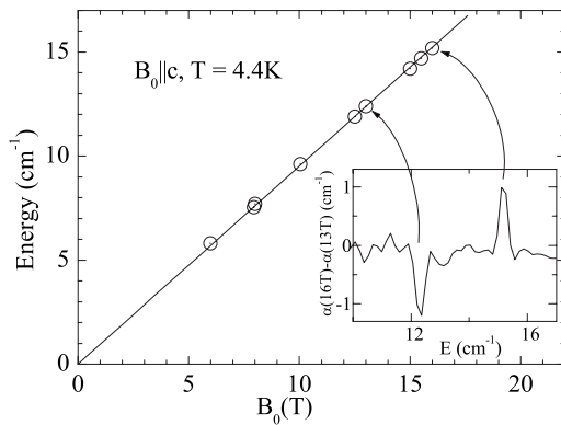
FIG. 4. Magnetic field dependence of the paramagnetic transition energy in B_0 \parallel c orientation. The line is a fit to the data yielding g_c = 2.038 \pm 0.016 . The inset demonstrates the paramagnetic transition signal in differential absorption spectrum. The linewidth is resolution limited by instrument to 0.3 \text{ cm}^{-1} .
