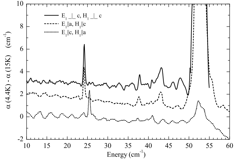
Figure 5.5: Differential absorption in \mathbf{E}_1 \perp \mathbf{c} (two upper curves) and \mathbf{E}_1 \parallel \mathbf{c} (lower curve) polarization. Spectra have been off-set in vertical direction.
