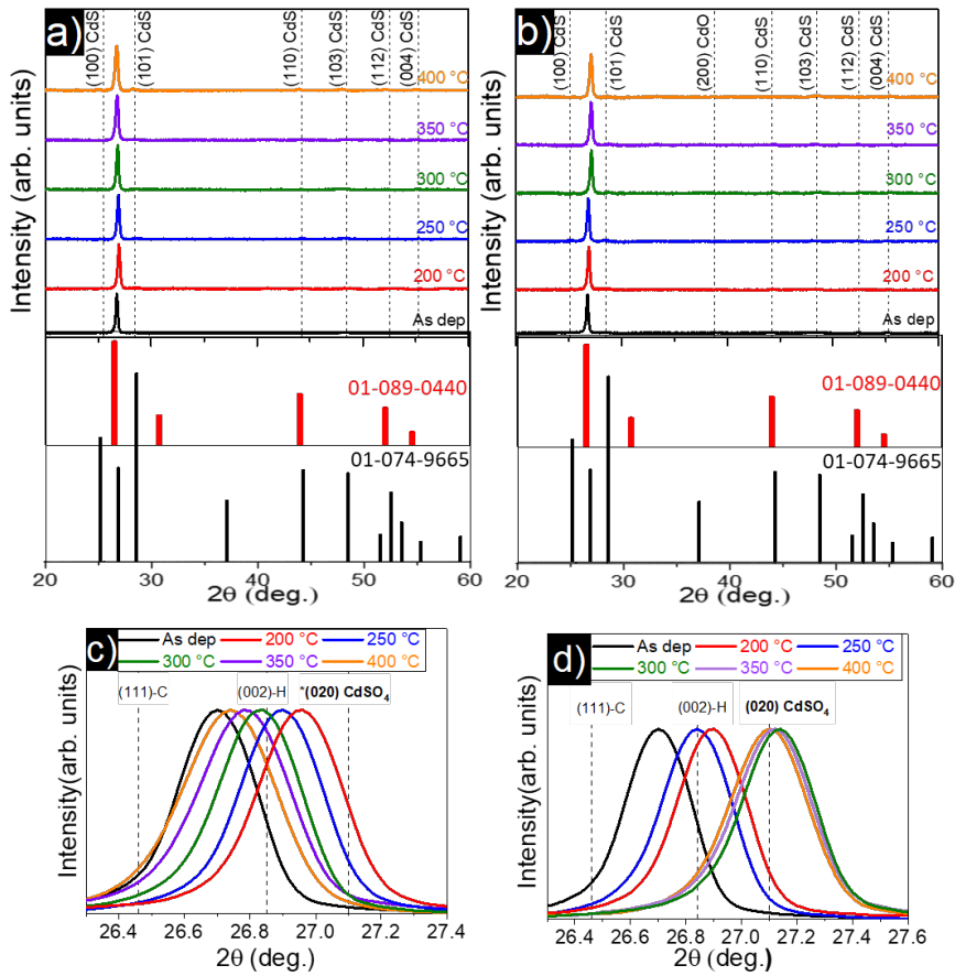
Figure 18. XRD pattern of a) vacuum annealed and b) air annealed CdS films, at 200 °C–400 °C temperatures for 30 min; displacement of dominant XRD peak depending on the c) vacuum and d) air annealing conditions.
