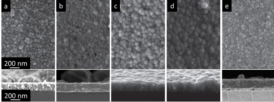
Figure 20. Surface and cross-section SEM images of CdS films deposited on glass substrates: a) as deposited, b) annealed in vacuum at 200 °C, c) annealed in air at 200 °C, d) annealed in vacuum at 400 °C, e) annealed in air at 400 °C with an annealing duration of 30 minutes.
