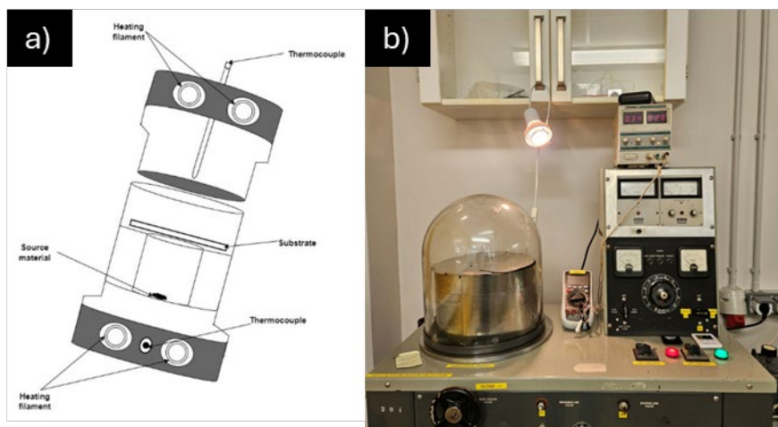
Figure 15. CSS set up a) schematic illustration and b) photograph of the actual experimental setup.
