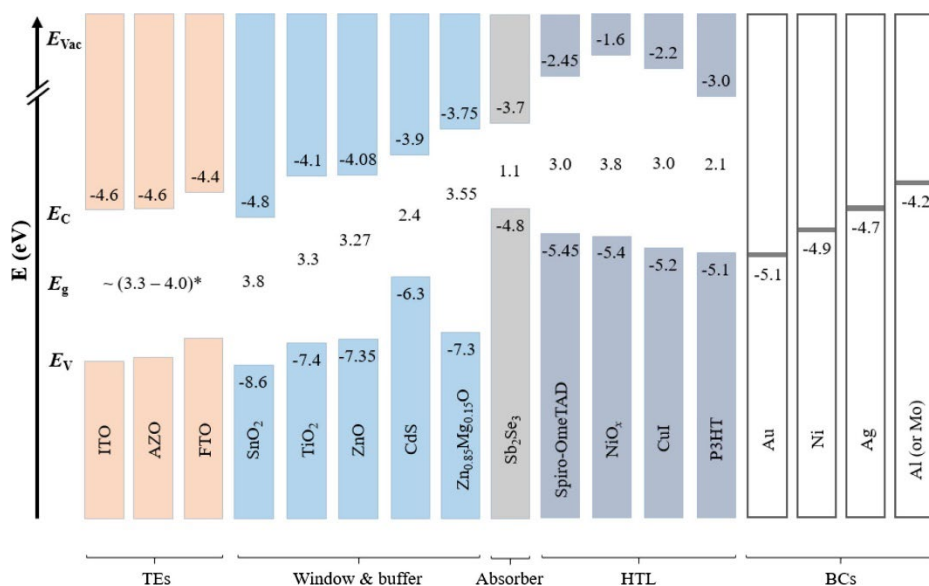
Figure 7. Schematic of the band alignment of \text{Sb}_2\text{Se}_3 solar cells with various ETL ( \text{SnO}_2 , \text{TiO}_2 , \text{ZnO} , \text{CdS} , \text{ZnMgO} ) along with front and back contacts [122].
