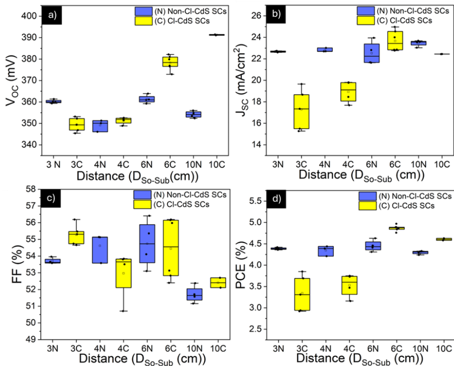
Figure 35. Variation of PV parameters cell a) V_{OC} b) J_{SC} c) FF and d) PCE of Non-Cl-CdS and Cl-CdS SCs at different D_{So-Sub} during VTD deposition.
