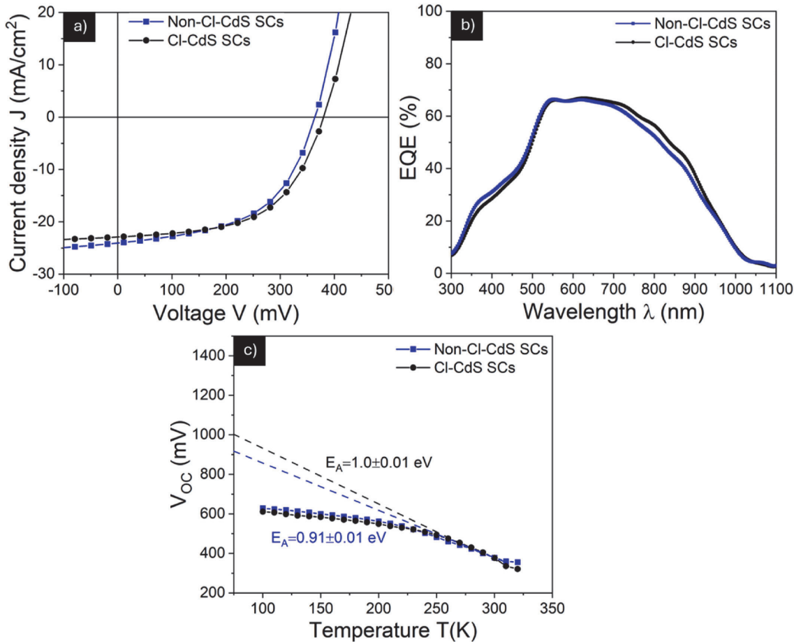
Fig. 4. (a) J-V characteristics and (b) EQE spectra of the best-performing Non-Cl-CdS and Cl-CdS SCs (c) V_{oc} - temperature dependence for Non-Cl-CdS and Cl-CdS SCs.
