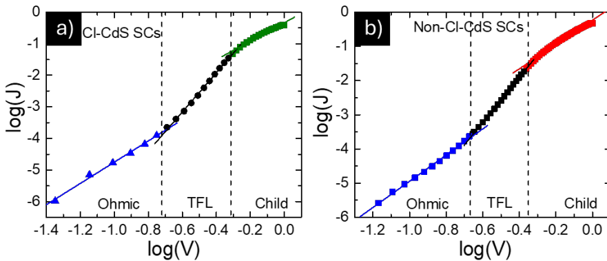
Figure 37. Log(J)-log(V) plots deduced from dark J-V curves of Cl-CdS SCs (a) and Non-Cl-CdS (b) SCs.
