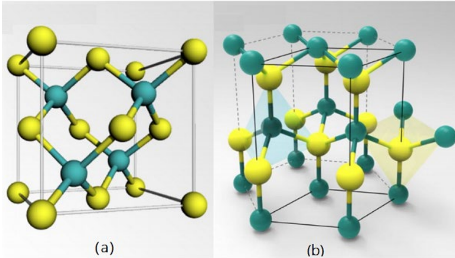
Figure 8. a) Cubic zinc blende and b) hexagonal wurtzite crystal structures of CdS [127].
