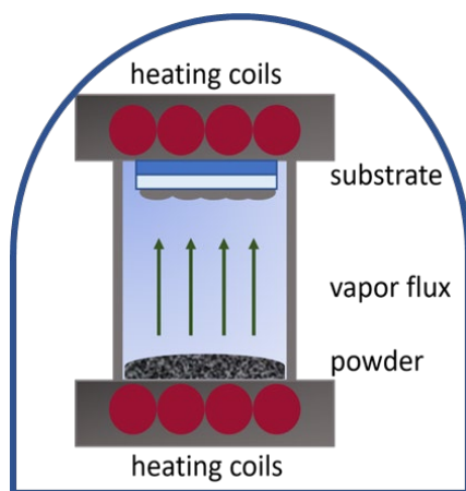
Figure 5. Schematic diagram of the CSS system [109].
