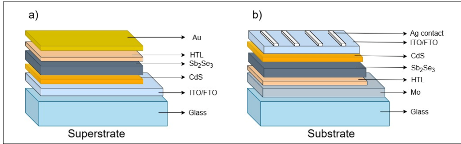
Figure 10. a) superstrate and b) substrate configuration of CdS/Sb 2 Se 3 solar cells.
