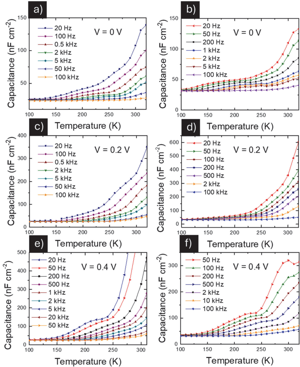
Fig. 6. C-f-T curves of Cl-CdS SCs measured under 0 V (a), 0.2 V (c), and 0.4 V (e) and Non-Cl-CdS SCs measured at 0 V (b), 0.2 V (d), and 0.4 V (f).
