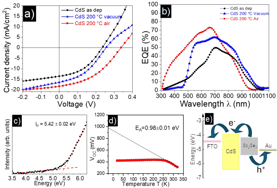
Figure 25. a) JV characteristics and b) EQE of CdS/ \text{Sb}_2\text{Se}_3 solar cells with as-deposited, air and vacuum annealed CdS at 200 °C, c) Ionization potential of \text{Sb}_2\text{Se}_3 d) activation energy calculated from V_{OC} -T plot, e) band alignment of FTO/CdS/ \text{Sb}_2\text{Se}_3 /Au solar cell structure.
