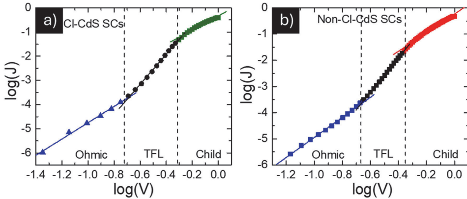
Fig. 5. Log(J)-log(V) plots deduced from dark J-V curves of Cl-CdS SCs (a) and Non-Cl-CdS (b) SCs.
