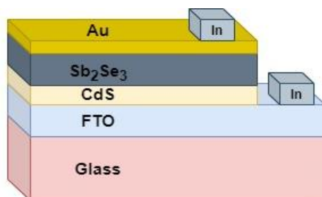
Figure 17. Superstrate configuration of solar cells used in this thesis study.
