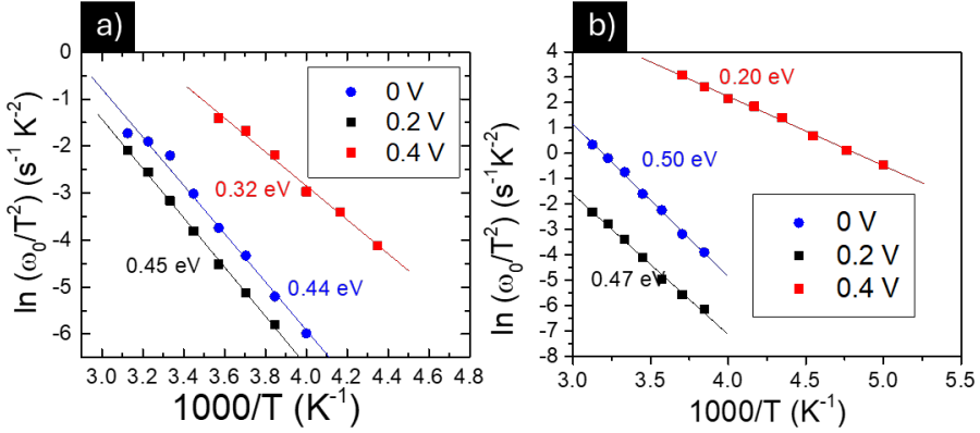
Figure 39. Arrhenius plot of the inflection frequencies of Cl-CdS SCs (a) and Non-Cl-CdS (b) SCs measured under 0 V, 0.2 V, and 0.4 V bias.
