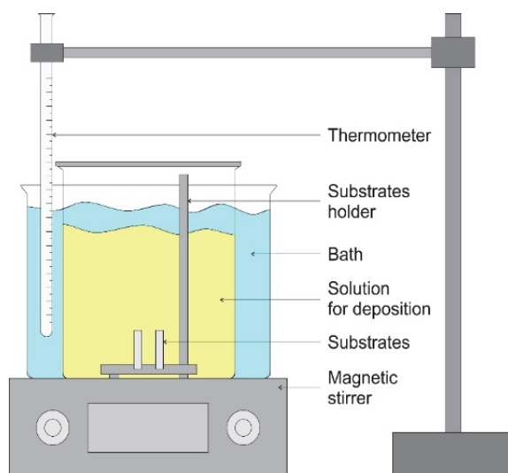
Figure 9. Schematic diagram of the CBD procedure of CdS films [174].
