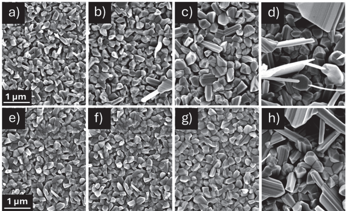
Fig. 2. (a–d) Surface SEM images of \text{Sb}_2\text{Se}_3 films deposited on Non-Cl-CdS films at 3, 4, 6 and 10 cm D_{\text{So-Sub}} (e–h) Surface SEM images of \text{Sb}_2\text{Se}_3 films deposited on Cl-CdS films at 3, 4, 6 and 10 cm D_{\text{So-Sub}} .
