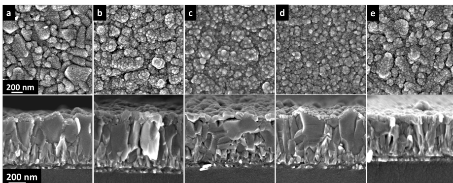
Figure 21. Surface and cross-section SEM images of CdS films deposited on FTO/glass substrates: a) as deposited, b) annealed in vacuum at 200 °C, c) annealed in air at 200 °C, d) annealed in vacuum at 400 °C, e) annealed in air at 400 °C with an annealing duration of 30 minutes.
