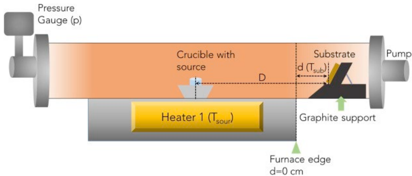
Figure 6. Schematic diagram of VTD setup used for thin film deposition [112].
