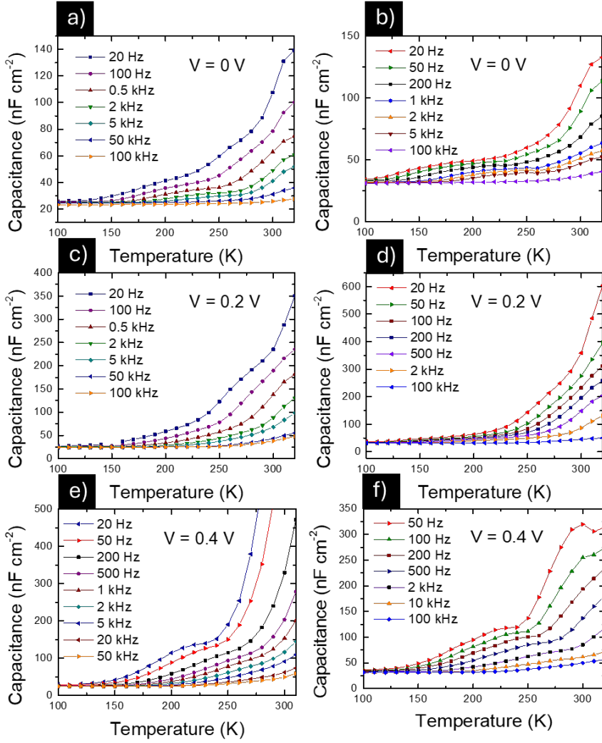
Figure 38. C-f-T curves of Cl-CdS SCs measured under 0 V (a), 0.2 V (c), and 0.4 V (e) and Non-Cl-CdS SCs measured at 0 V (b), 0.2 V (d), and 0.4 V (f).
