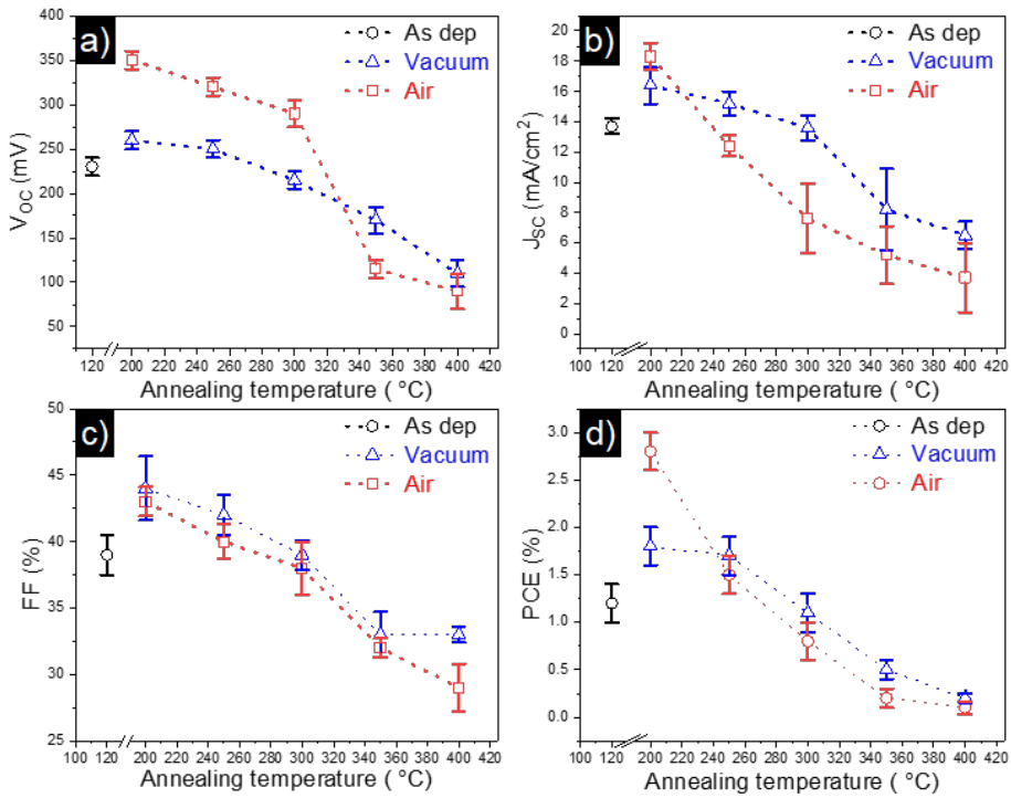
Figure 26. Main photovoltaic parameters, including a) open circuit voltage ( V_{OC} ), b) short circuit current density ( J_{SC} ), c) fill factor (FF), and d) photoconversion efficiency (PCE) with average values (marked as hollow squares) measured for Sb 2 Se 3 devices.
