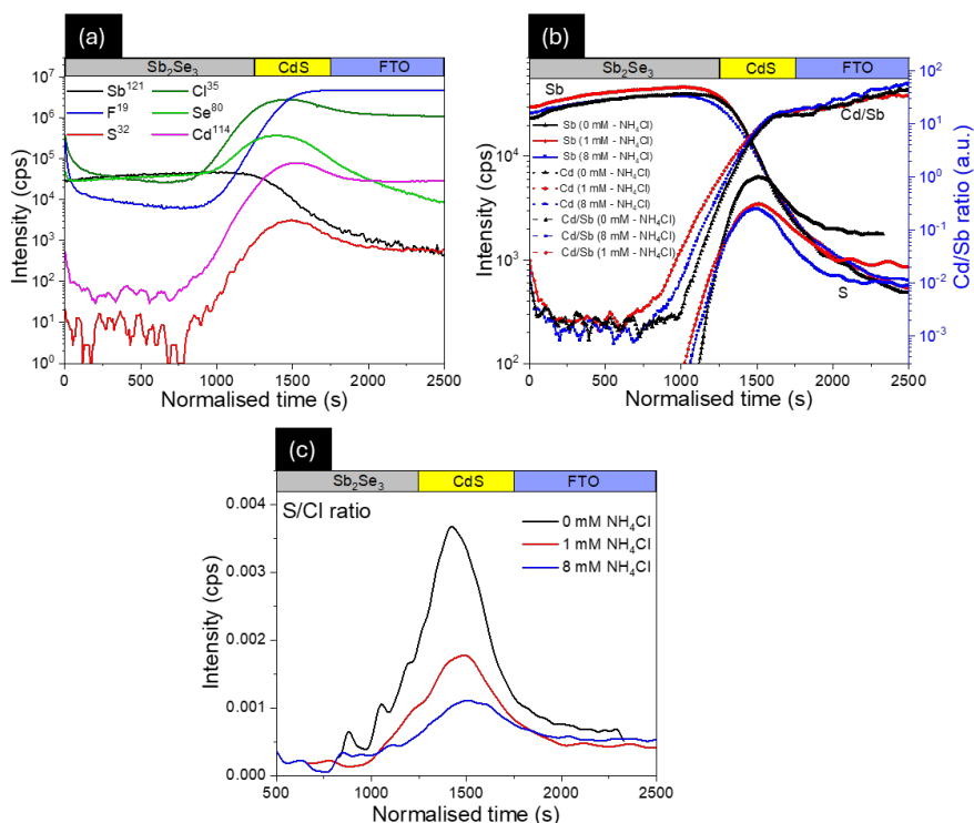
Figure 31. Secondary ion mass Spectroscopy (SIMS) depth profiles, a) Sb, Se, Cd, S, Cl, and F elemental distribution in 1 mM \text{NH}_4\text{Cl} -CdS samples b) Cd/Sb ratio at \text{NH}_4\text{Cl} -CdS/ \text{Sb}_2\text{Se}_3 interface c) S/Cl ratio of 0, 1, 8 mM \text{NH}_4\text{Cl} -CdS samples.
