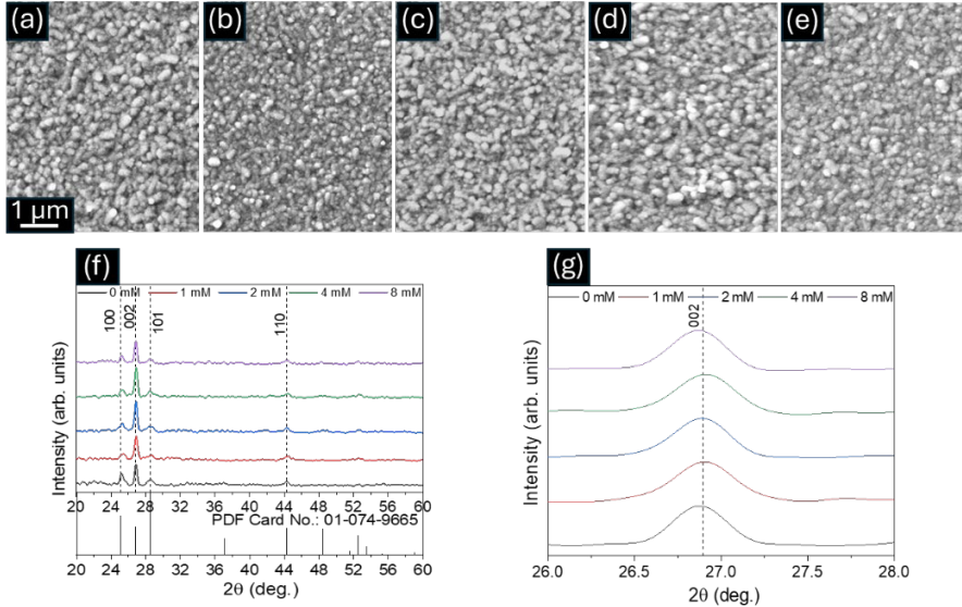
Figure 27. (a-e) Surface SEM images of CdS films prepared with 0, 1, 2, 4, and 8 mM \text{NH}_4\text{Cl} in the CBD precursor, (f) XRD pattern of CdS with different \text{NH}_4\text{Cl} concentration, (g) Variation of (002) peak of CdS films with different \text{NH}_4\text{Cl} concentration.
