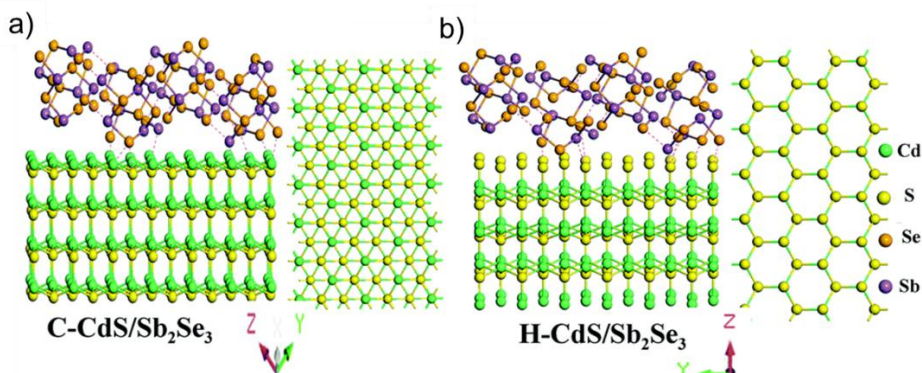
Figure 11. growth diagram of \text{Sb}_2\text{Se}_3 on, a) cubic (C-CdS) and b) hexagonal (H-CdS) CdS films.
