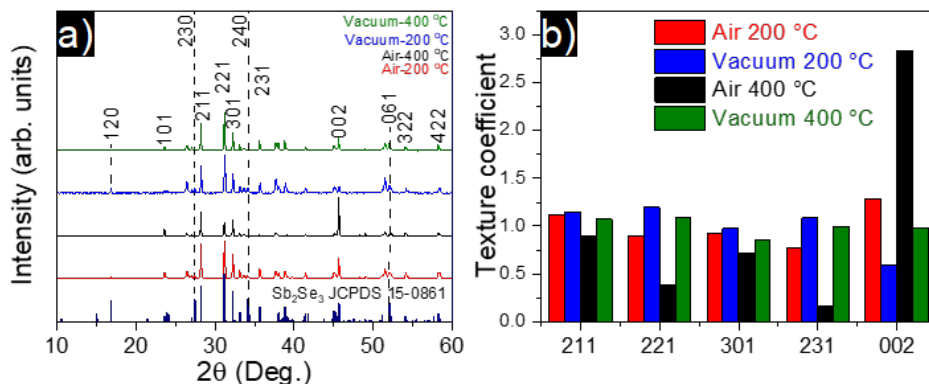
Figure 23. a) XRD spectrum and b) texture coefficient of \text{Sb}_2\text{Se}_3 on CdS annealed in vacuum and air at 200 °C and 400 °C.
