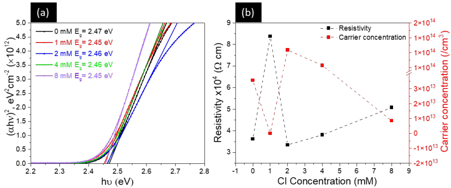
Figure 28. (a) Tauc plots, showing the variation in bandgap of CdS films processed with 0–8 mM \text{NH}_4\text{Cl} concentration (b) electrical properties (carrier concentration and resistivity) of CdS films with different \text{NH}_4\text{Cl} concentration.
