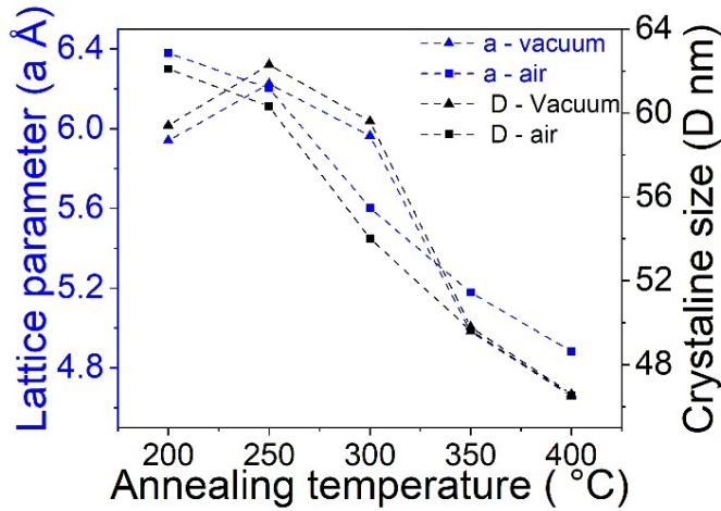
Figure 19. Variation of lattice parameter ( a ) and crystalline size ( D ) depending on the vacuum and air annealing temperatures.
