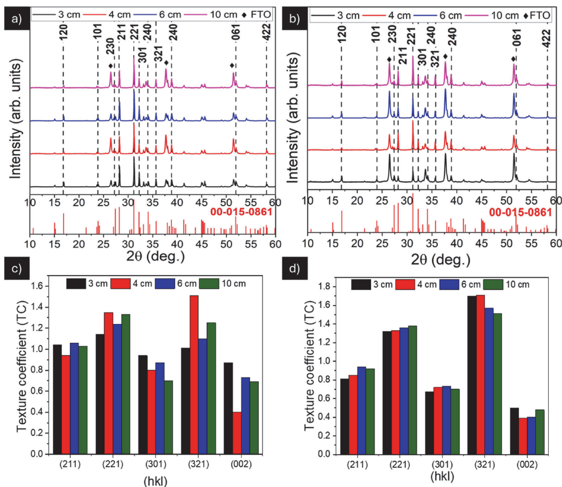
Fig. 1. a) & c) XRD pattern and Texture coefficient of Sb 2 Se 3 films (constant thickness of \sim 0.8 \mu m) deposited on Non-Cl-CdS films at 3, 4, 6 and 10 source to substrate VTD distance ( D_{\text{So-Sub}} ), b) & d) XRD pattern and Texture coefficient of Sb 2 Se 3 films deposited on Cl-CdS films at 3, 4, 6 and 10 D_{\text{So-Sub}} .
