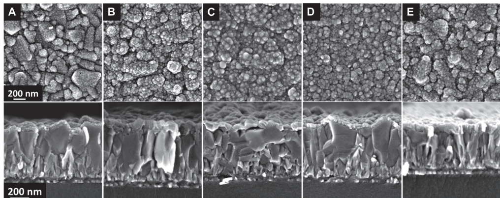
FIGURE 4 Surface and cross-section SEM images of CdS films deposited on FTO/glass substrates: (A) as deposited, (B) annealed in vacuum at 200°C, (C) annealed in air at 200°C, (D) annealed in vacuum at 400°C, (E) annealed in air at 400°C with an annealing duration of 30 min.
