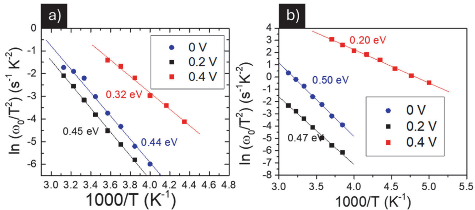
Fig. 7. Arrhenius plot of the inflection frequencies of Cl-CdS SCs (a) and Non-Cl-CdS (b) SCs measured under 0 V, 0.2 V, and 0.4 V bias.
