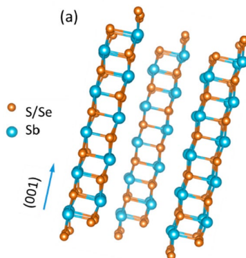
Figure 2. Sb chalcogenide 1D ribbon structure [72].
