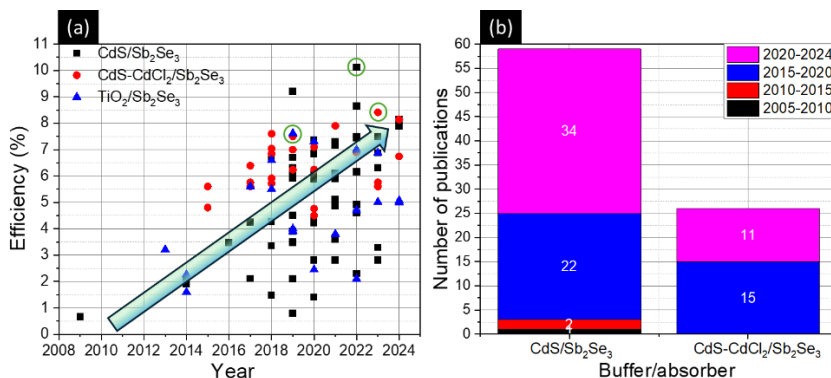
Figure 12. a) Evolution of \text{Sb}_2\text{Se}_3 solar cell efficiency with CdS, CdCl 2 -CdS and TiO 2 ETLs and b) the corresponding number of publications.
