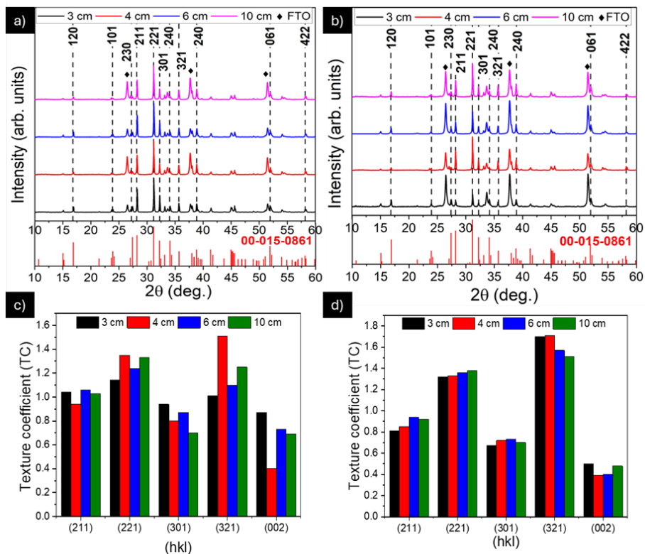
Figure 33. a) & c) XRD pattern and Texture coefficient of \text{Sb}_2\text{Se}_3 films (constant thickness of \sim 0.8 \mu\text{m} ) deposited on Non-Cl-CdS films at 3, 4, 6 and 10 source to substrate VTD distance ( D_{\text{So-Sub}} ), b) & d) XRD pattern and Texture coefficient of \text{Sb}_2\text{Se}_3 films deposited on Cl-CdS films at 3, 4, 6 and 10 D_{\text{So-Sub}} .
