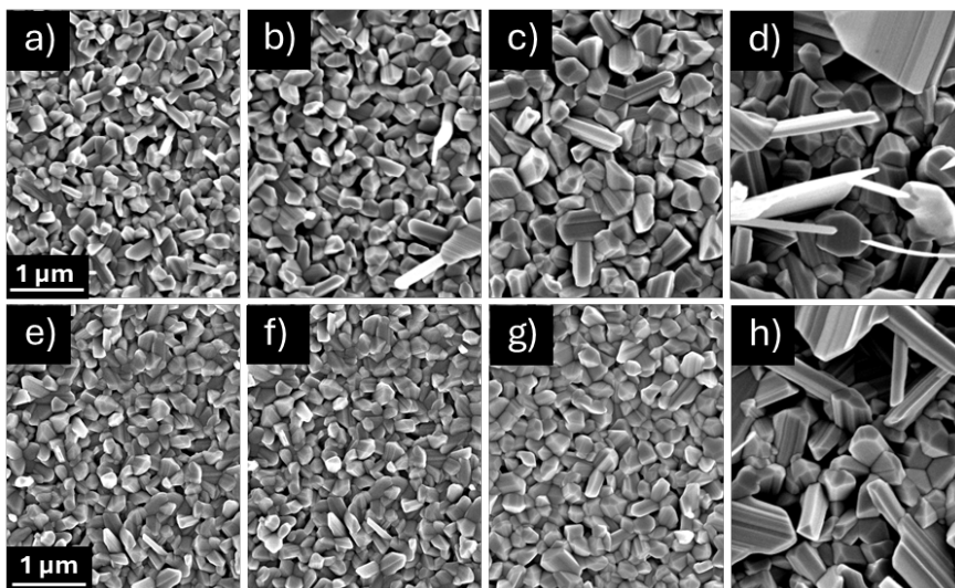
Figure 34. a-d) Surface SEM images of \text{Sb}_2\text{Se}_3 films deposited on Non-Cl-CdS films at 3, 4, 6 and 10 cm D_{\text{So-Sub}} (e-h) Surface SEM images of \text{Sb}_2\text{Se}_3 films deposited on Cl-CdS films at 3, 4, 6 and 10 cm D_{\text{So-Sub}} .
