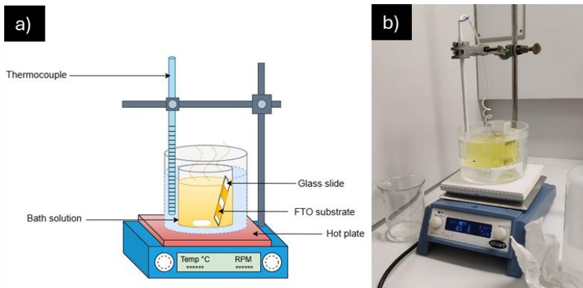
Figure 14. CBD set up a) schematic illustration and b) photograph of the actual experimental setup.
