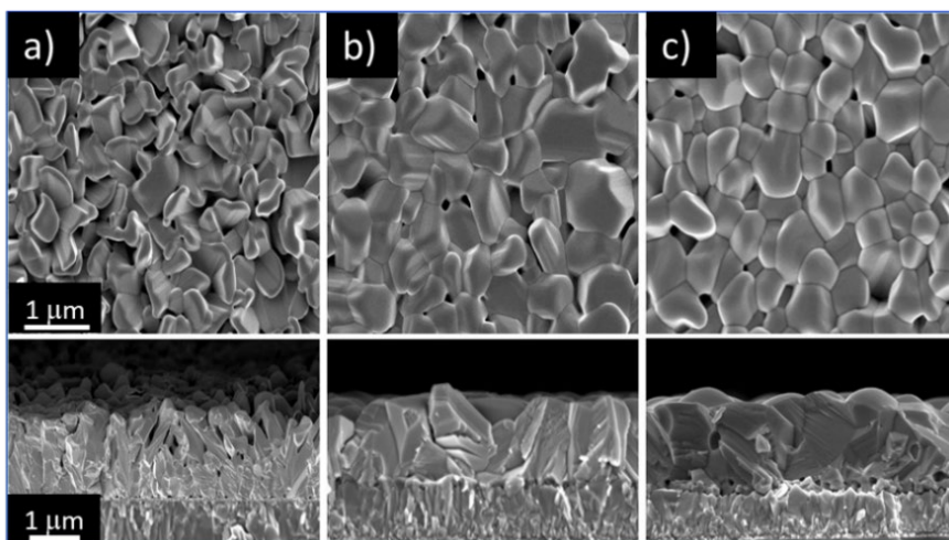
Figure 24. SEM images of superstrate configuration glass/FTO/CdS/Sb 2 Se 3 stack with CSS Sb 2 Se 3 absorber layer deposited at 460 °C: a) top-and cross-sectional view of absorber film deposited onto as-deposited CdS, b) top-and cross-sectional view of absorber deposited onto vacuum annealed CdS at 200 °C and c) top-and cross-sectional view of absorber deposited onto air annealed CdS at 200 °C.
