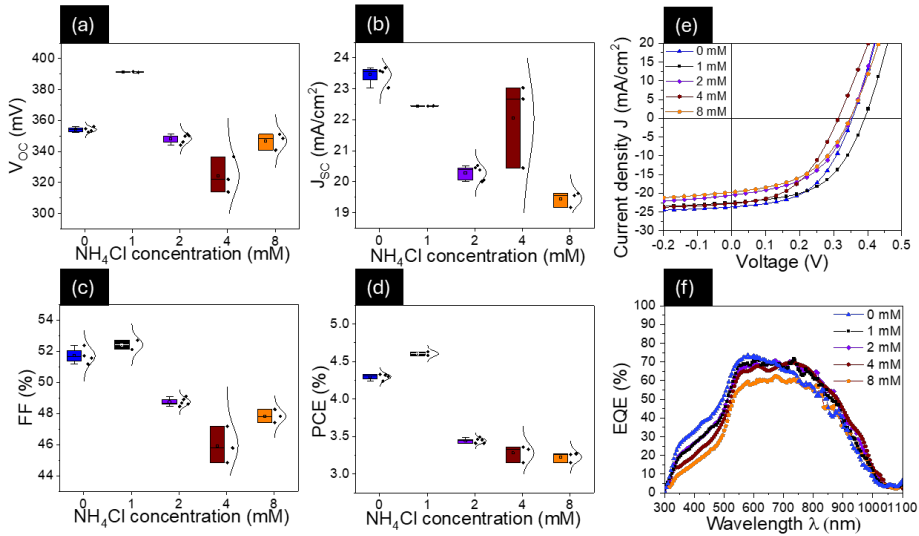
Figure 32. (a) open circuit voltage ( V_{oc} ), (b) short circuit current density ( J_{sc} ), (c) fill factor (FF), (d) power conversion efficiency (PCE), (e) JV characteristics and (f) external quantum efficiency (EQE) of \text{CdS}/\text{Sb}_2\text{Se}_3 solar cells with a change in \text{NH}_4\text{Cl} concentration in the CBD-CdS.
