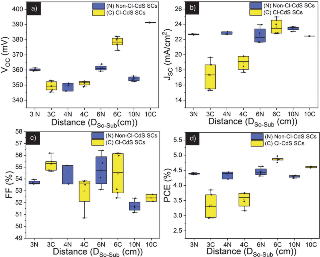
Fig. 3. Variation of PV parameters cell a) V_{\text{OC}} , b) J_{\text{SC}} , c) FF and d) PCE of Non-Cl-CdS and Cl-CdS SCs at different D_{\text{So-Sub}} during VTD deposition. (N) and (C) stand for Non-Cl-CdS SCs and C-CdS SCs, while the numbers on the x-axis indicate the source-to-substrate distance ( D_{\text{So-Sub}} ).
