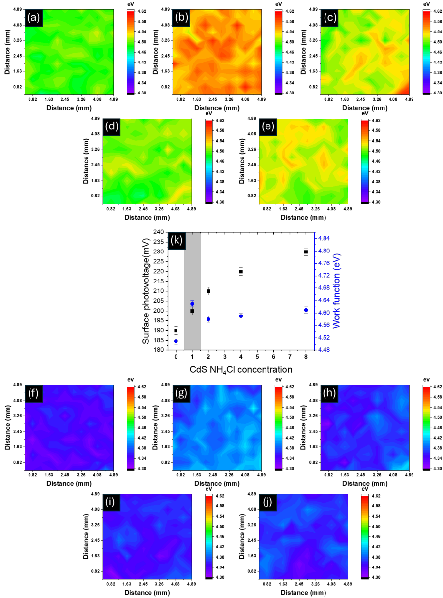
Figure 29. (a, b, c, d, e) dark and (f, g, h, i, j) light condition work function distribution of CdS films at 0, 1, 2, 4, and 8 mM NH 4 Cl in order (k) Variation of work function (WF) and surface photovoltage (SPV) with the change in NH 4 Cl concentration.
