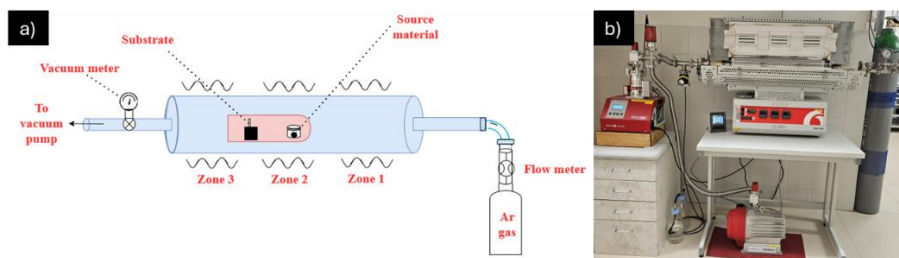
Figure 16. VTD set up a) schematic illustration and b) photograph of the actual experimental setup.
