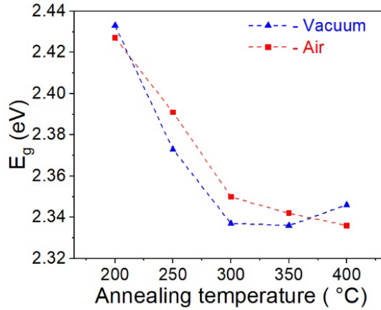
Figure 22. Variation in the bandgap of CdS films with vacuum and air annealing temperature.
