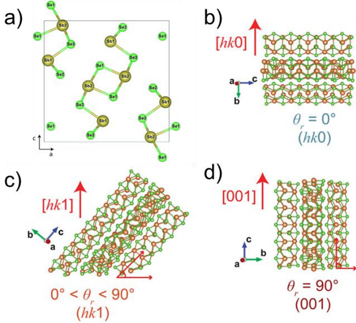
Figure 4. a) Schematic diagram of the \text{Sb}_2\text{Se}_3 unit cell and crystallographic orientations b) [hk0] c) [hk1] and d) [001] [87], [89].
