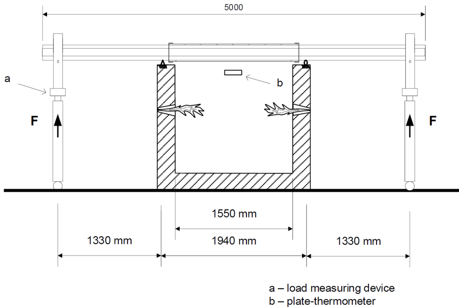
Figure 36. Loaded model-scale test setup from the FIRENWOOD report (Olofsson et al., 2022).
