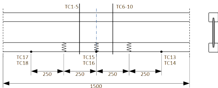
Figure 34. Location of thermocouples and finger-joints.
