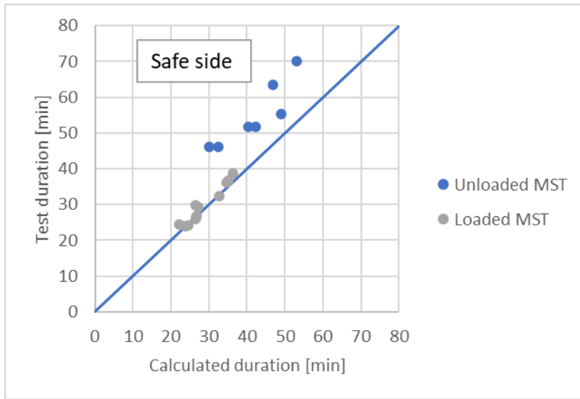
Figure 80. Comparison of calculated and tested durations to reach the same charred areas.
