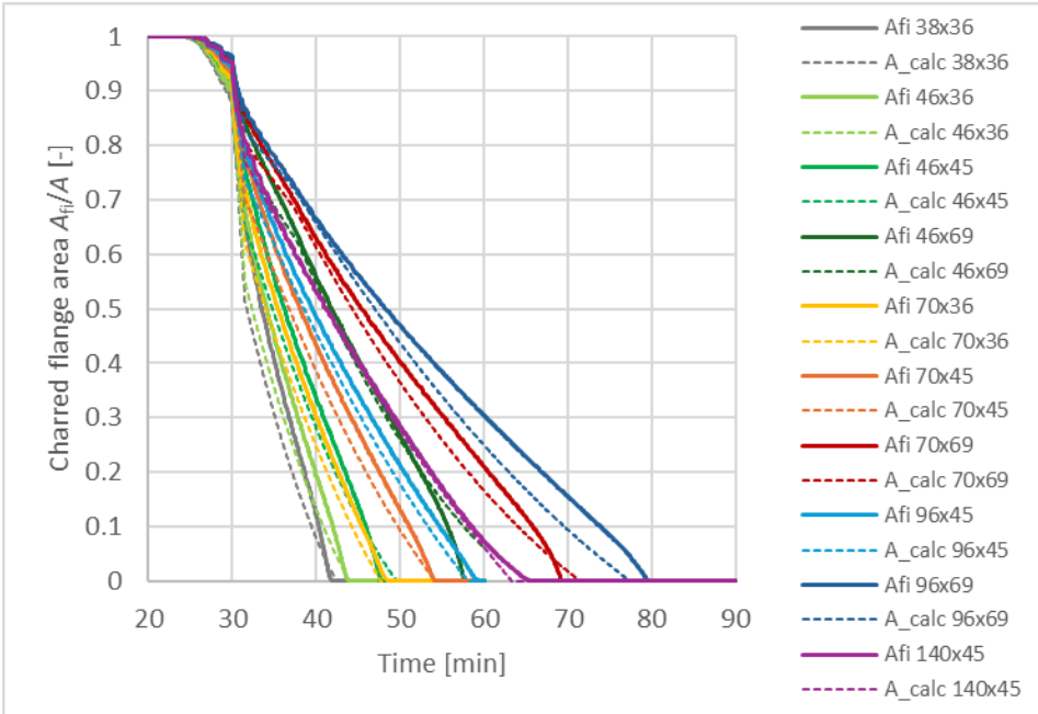
Figure 30. Comparison of simulated and calculated charred areas for assemblies insulated with stone wool and protected by 13-mm gypsum plasterboard with 30-minute fall-off time.
