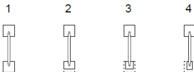
Figure 62. Types of reduced cross-sections of I-joists.
