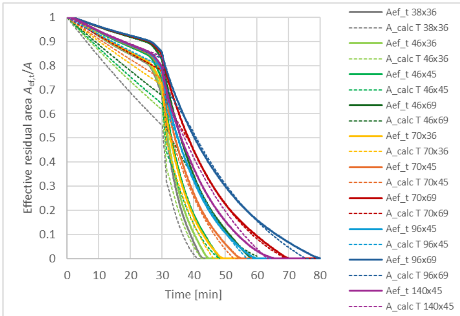
Figure 53. Comparison of simulated and calculated effective areas in tension for assemblies insulated with stone wool and protected by 15-mm gypsum plasterboard with 30-minute fall-off time.
