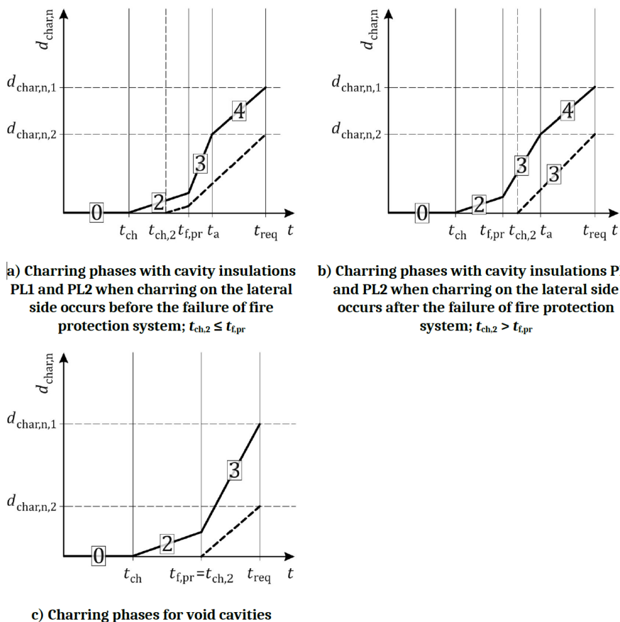
Figure 79. Design model for I-shaped timber members of timber frame assemblies according to FprEN 1995-1-2:2025 (CEN, 2025b).
