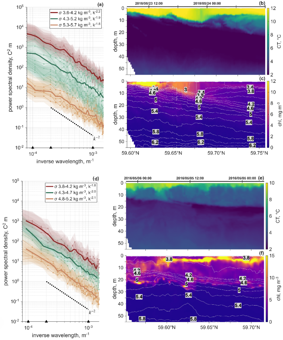
Figure 6. Wavenumber spectra and hydrographic structure during frontal missions in 2018 and 2016. Panels (a, d) show along-isopycnal temperature spectra for the 2018 and 2016 missions, respectively, grouped into three \sigma -ranges shown in red, green, and orange. The red range corresponds to the upper density layer, extending to approximately 10 m in 2018 and 15 m in 2016. The green range extends from the base of this upper layer to approximately 25 m, and the orange range corresponds to approximately 25–40 m. Thin lines show individual spectra, thick lines show mean spectra, and shaded envelopes indicate 95% confidence intervals. The dashed black line indicates a k^{-2} reference slope, and triangles mark wavelengths of 10, 5, and 1 km. Panels (b, c) and (e, f) show example temperature and chlorophyll distributions overlaid with \sigma -contours at 0.2 \text{ kg m}^{-3} intervals from 2018 and 2016, respectively.
