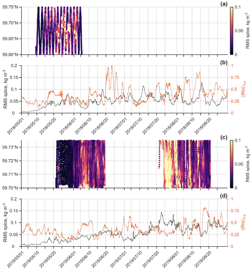
Figure 8. RMS spice in spring–summer 2018–2019, calculated over the density range extending from the surface to the depth of minimum temperature (approximately the upper 0–30 m). Panels (a, c) show the latitude–time distribution of RMS spice from the glider missions. Panels (b, d) show the corresponding model diagnostics within a 10×10 km study window: RMS spice in black and RMS surface Rossby number in orange. Modified from Paper II.
