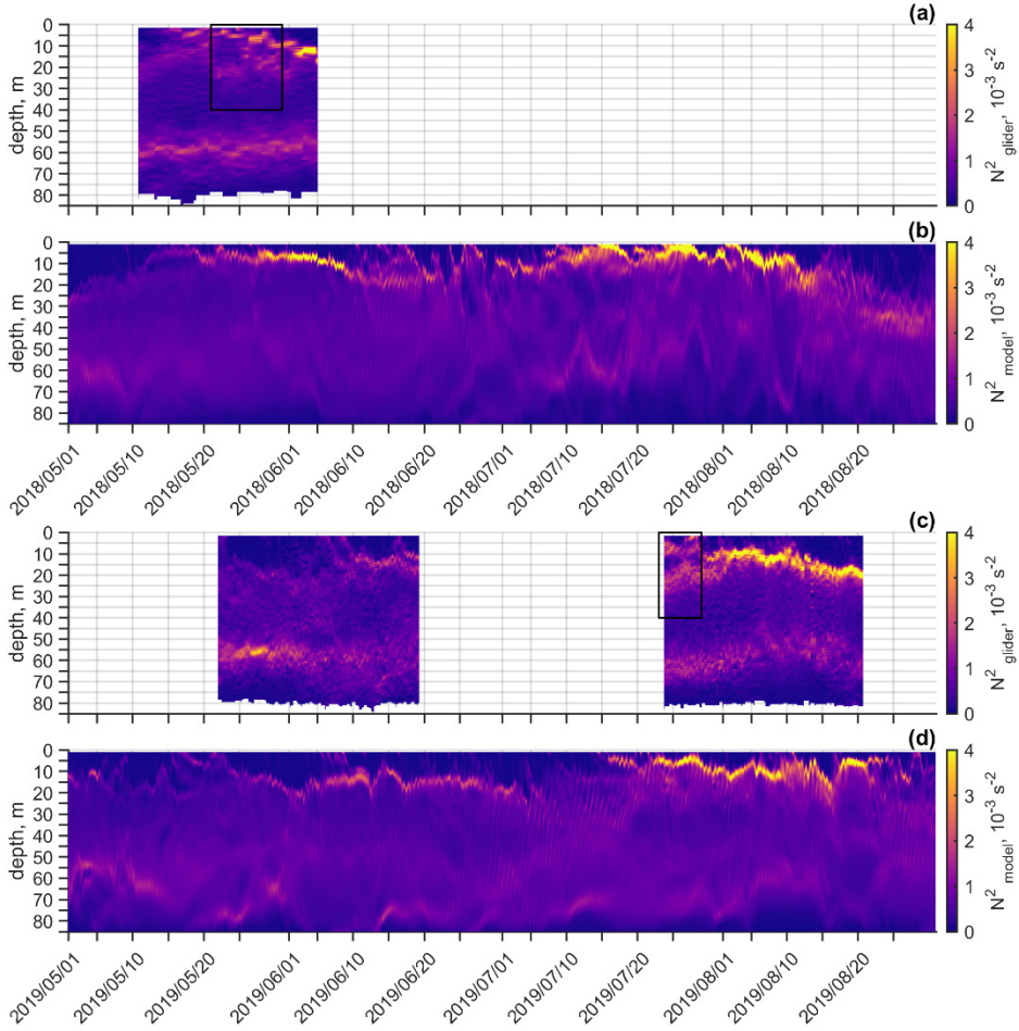
Figure 2. Vertical stratification variability expressed as the squared Brunt–Väisälä frequency ( N^2 ) derived from glider observations (a, c) and model output (b, d) for May–August 2018 (a, b) and 2019 (c, d). The glider data represent average profiles for each section within the selected area, based on observations collected along approximately 1 km of glider track, and thus form a composite vertical structure. The model data show average profiles within a 1×1 km window at each model output time. Black boxes indicate periods of two local maxima in N^2 : 21–30 May 2018 (a) and 23–28 July 2019 (c). Modified from Paper II.
