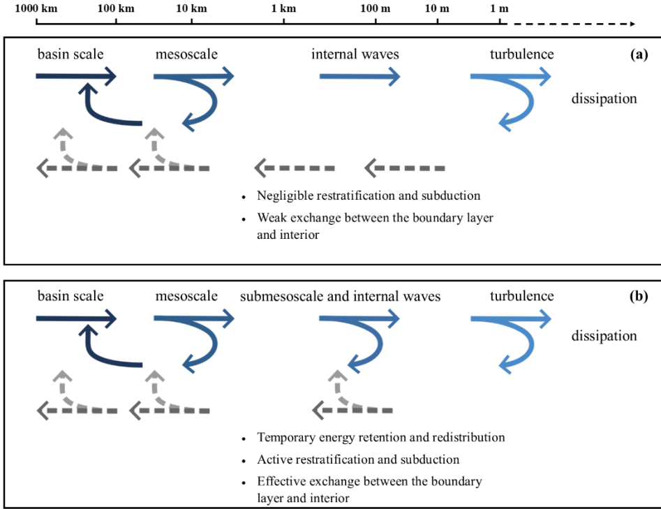
Figure 12. Schematic illustration of energy-transfer pathways across spatial scales. (a) Classical view in which mesoscale energy is transferred toward dissipation primarily via internal gravity waves. (b) Expanded framework including submesoscale processes, which introduce additional, dynamically active pathways for energy redistribution. In this view, energy extracted from mesoscale density gradients is temporarily retained, converted, and redistributed within the SMS range before contributing to dissipation. The schematic emphasises pathways rather than specific instability mechanisms. Modified from Paper III.
