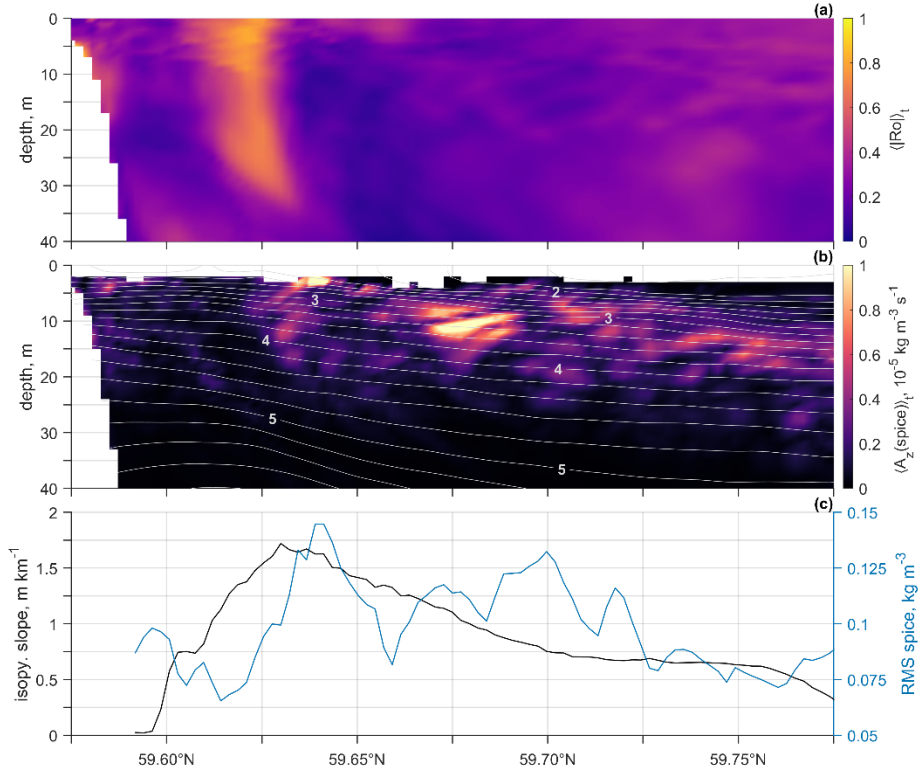
Figure 10. Period-mean dynamical and tracer diagnostics for the upwelling period of 26–31 July 2019 along the meridional transect at 25.25° E. Panels show (a) the magnitude of the Rossby number, and (b) the magnitude of the vertical advective tendency of spice. Panel (c) shows along-transect isopycnal slope and RMS spice, averaged from the surface down to the depth of minimum temperature.
