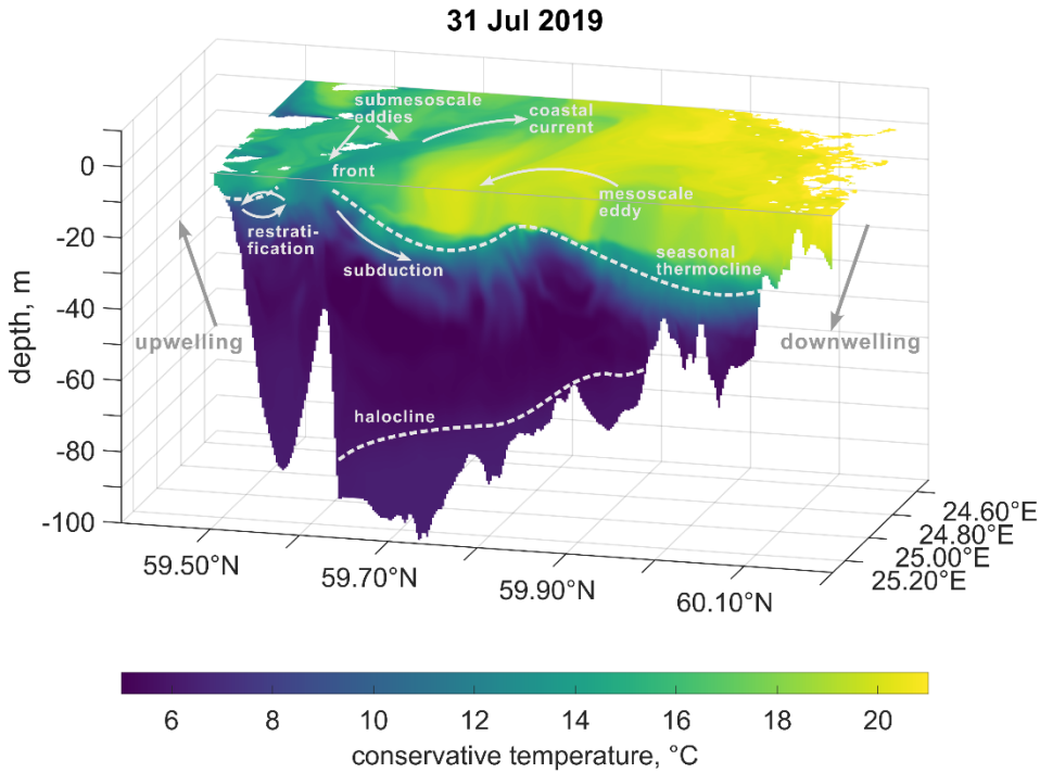
Figure 11. Conceptual three-dimensional view of water-column temperature across the Gulf of Finland on 31 July 2019. The horizontal view spans 59.50–60.20°N and 24.50–25.30°E, while the vertical section follows a meridional transect along 25.30°E. The stratified structure reveals oppositely sloping thermocline and halocline layers and a pronounced frontal zone along the southern coast. Hypothetical contours schematically indicate key features, including the coastal current, mesoscale and submesoscale eddies, frontal zone, subduction, and restratification near the base of the upper mixed layer.
