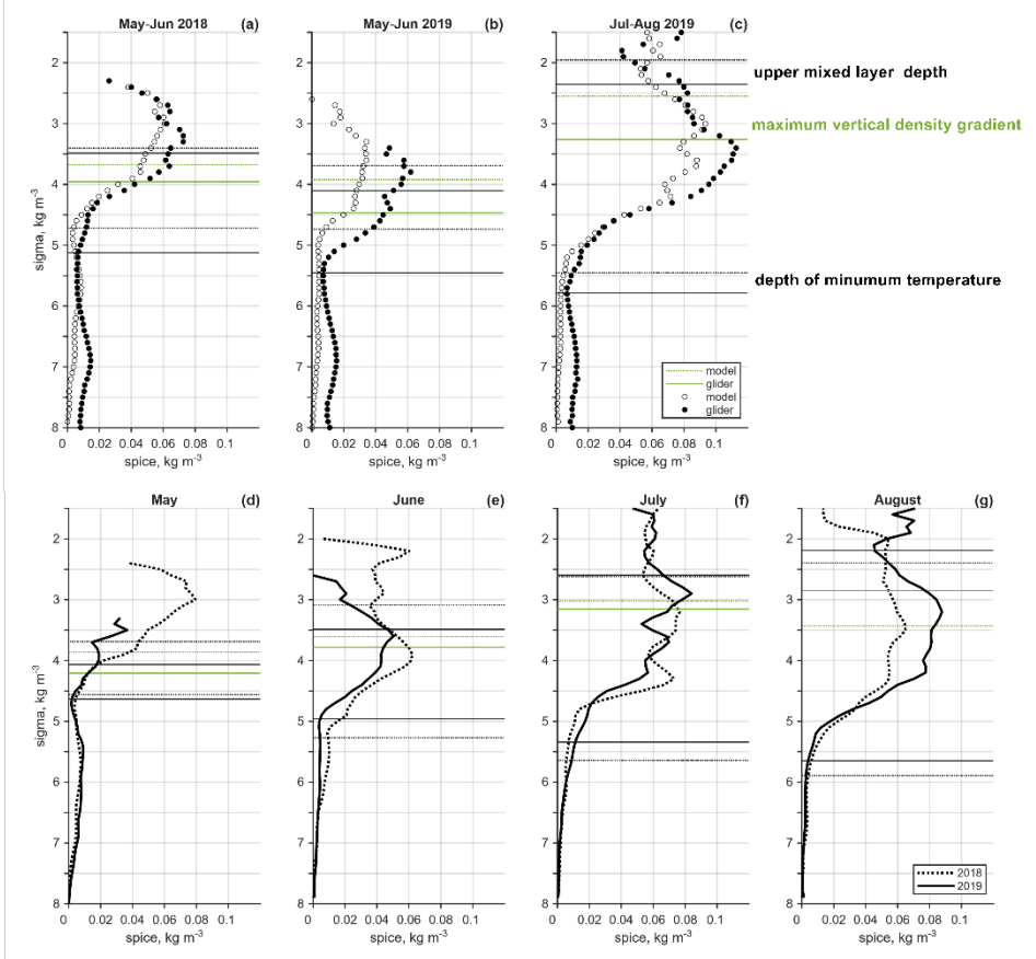
Figure 9. Vertical distribution of spice variability expressed as the standard deviation of spice. Panels (a–c) show spice variability from glider observations (black dots) and model output (white circles) for each glider mission period. Solid and dashed black lines indicate the average depth of the UML and the depth of minimum temperature derived from observations and model output, respectively. Green lines denote the average depth of the maximum Brunt–Väisälä frequency. Panels (d–g) show the monthly standard deviation of modelled spice from May to August for 2018 (dashed lines) and 2019 (solid lines). The same reference depths shown in panels (a–c) are indicated by black and green horizontal lines. From Paper II.
