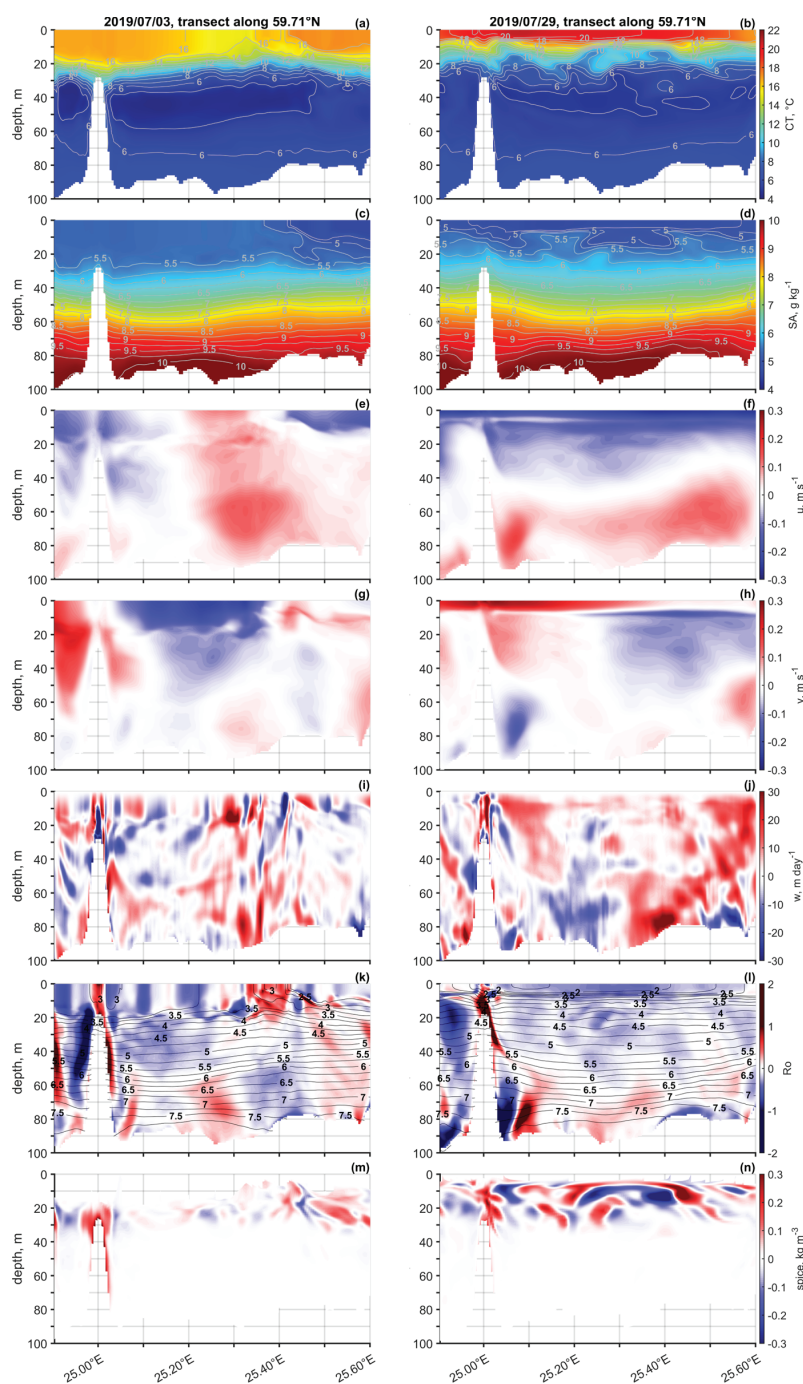
Figure 13. Vertical sections along zonal transects at 59.71^{\circ}\text{N} on 3 July (a, c, e, g, i, k, m) and 29 July 2019 (b, d, f, h, j, l, n), showing (a, b) Conservative Temperature ( ^{\circ}\text{C} ), (c, d) Absolute Salinity ( \text{g kg}^{-1} ), (e, f) zonal velocity u ( \text{m s}^{-1} ), (g, h) meridional velocity v ( \text{m s}^{-1} ), (i, j) vertical velocity w ( \text{m d}^{-1} ), (k, l) Rossby number ( Ro ) with overlaid isopycnals ( 0.25 \text{ kg m}^{-3} intervals), and (m, n) spice ( \text{kg m}^{-3} ).
