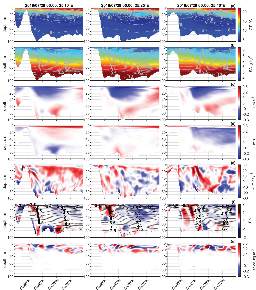
Figure 11. Vertical sections along three meridional transects at 25.10, 25.25, and 25.40° E on 29 July 2019, showing (a) Conservative Temperature (°C), (b) Absolute Salinity ( \text{g kg}^{-1} ), (c) zonal velocity u ( \text{m s}^{-1} ), (d) meridional velocity v ( \text{m s}^{-1} ), (e) vertical velocity w ( \text{m d}^{-1} ), (f) Rossby number ( Ro ) with overlaid isopycnals ( 0.25 \text{ kg m}^{-3} intervals), and (g) spice ( \text{kg m}^{-3} ). Transect locations are shown in Fig. 12f.
