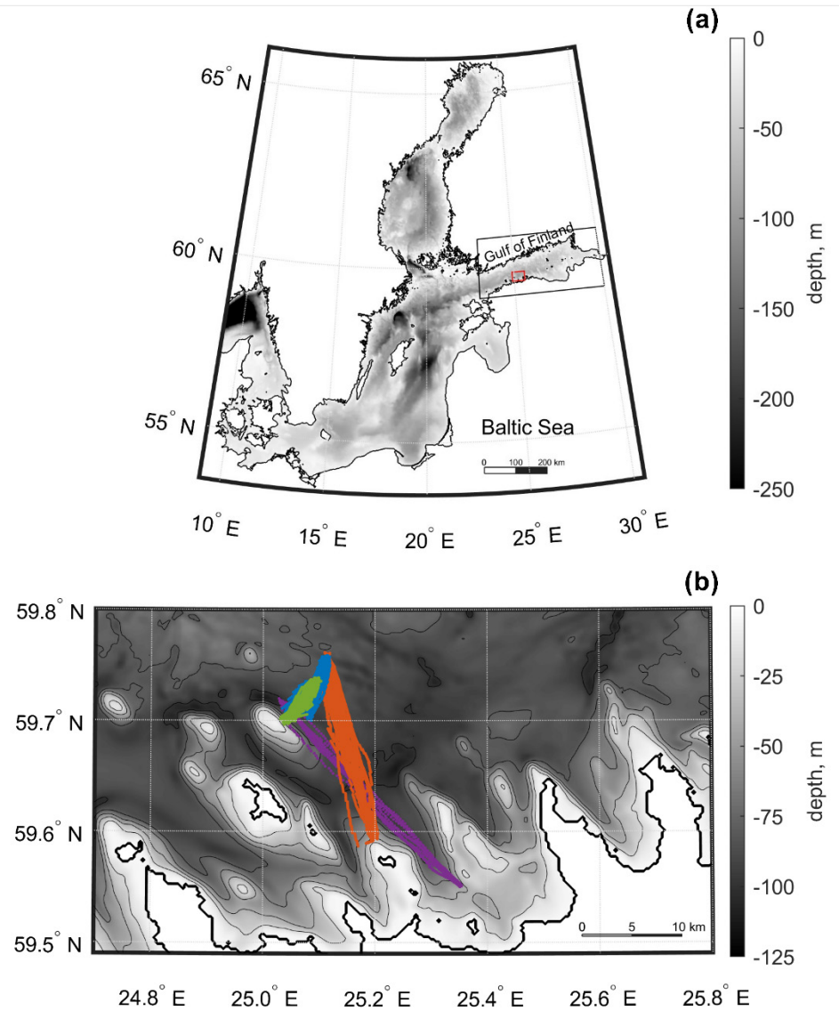
Figure 1. Map of the Baltic Sea (a), with the red rectangle marking the location of the study area shown in panel (b). The colormap indicates the bathymetry used in the model, while depth isolines in panel (b) are shown at 20 m intervals. Glider mission tracks from May 2016, May–June 2018, May–June 2019, and July–August 2019 are shown in purple, orange, blue, and green, respectively. Modified from Paper II.
