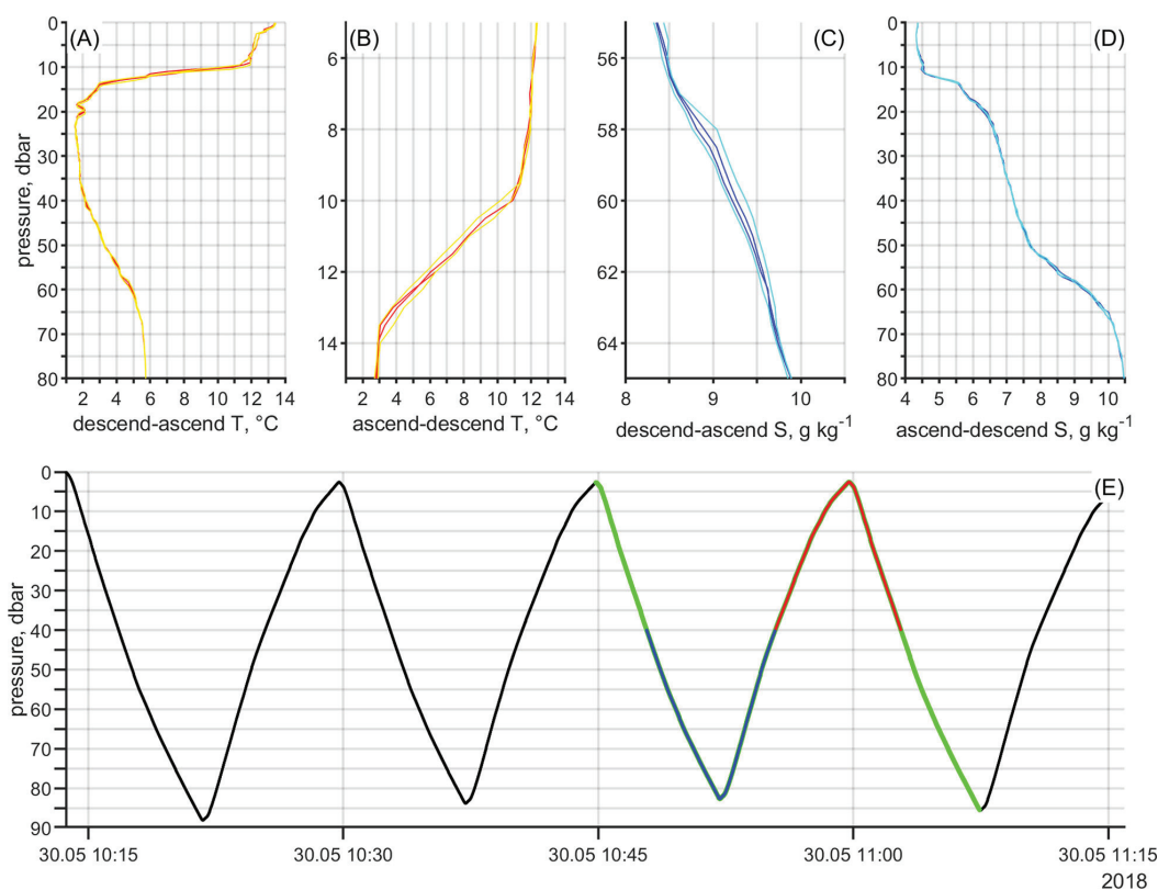
FIGURE 9 (A, B) Examples of raw (yellow) and corrected (response time, red) temperature profiles respectively over the water column and the thermocline depth range in case of descend-ascend (highlighted with blue in E) and ascend-descend (highlighted with red in E). (C, D) Examples of raw (cyan) and corrected (thermal lag, blue) salinity profiles respectively over the halocline depth range and the water column in case of descend-ascend and ascend-descend. (E) An example of a cycle shown as a time series of pressure. Green highlights the consecutive profiles. Overlaid blue shows the parts of profiles with a "V" shape, and red a "Λ" shape.
