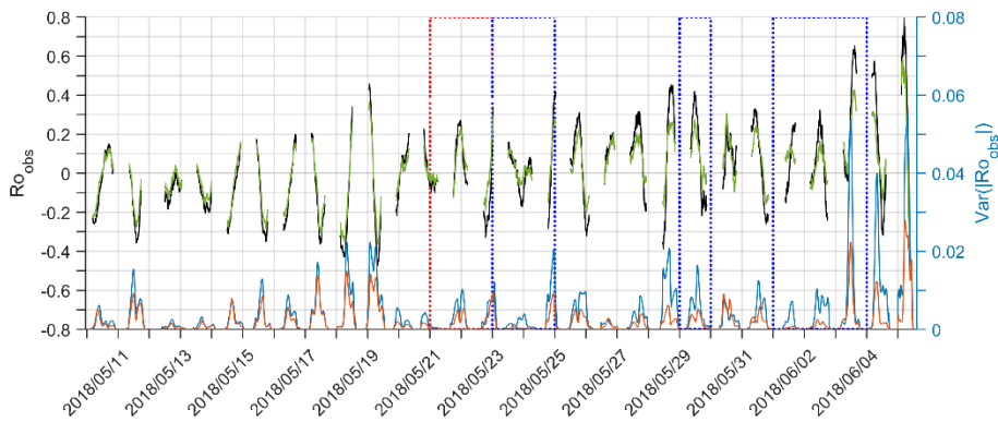
Figure 5. Observational Rossby number proxy ( Ro_{obs} ) estimated from glider observations and its moving-window variance. The Rossby number proxy is shown for vertical averaging over 0–10 m (black) and 0–30 m (green), while the corresponding moving-window variance is shown in blue (0–10 m) and orange (0–30 m). Red and blue rectangles denote periods of enhanced equivalent heat flux associated with baroclinic and wind-driven processes, respectively.
