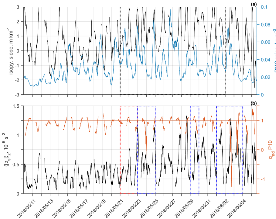
Figure 4. Time series of diagnostics indicative of SMS activity derived from glider observations during the May–June 2018 mission. (a) Isopycnal slope (black; \text{m km}^{-1} ), computed over a 5 km
