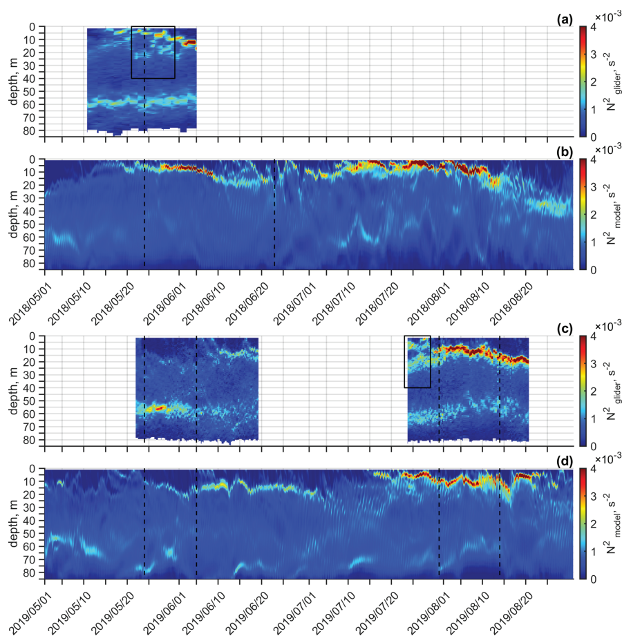
Figure 5. Variability of vertical stratification presented as Brunt–Väisälä frequency squared ( N^2 ) based on glider data ( a , c ) and model data ( b , d ) for May–August 2018 ( a , b ) and 2019 ( c , d ). The glider data represent average profiles for each section within the selected area, forming a composite salinity field. The model data show average profiles within a 1 \times 1 km window at each model output time. Vertical black lines indicate the dates shown in Fig. 8: 24 May and 23 June 2018 ( a , b ); 24 May, 5 June, 31 July, and 14 August 2019 ( c , d ). Black boxes indicate periods of two observed local maxima in N^2 : 21–30 May 2018 ( a ) and 23–28 July 2019 ( c ).
