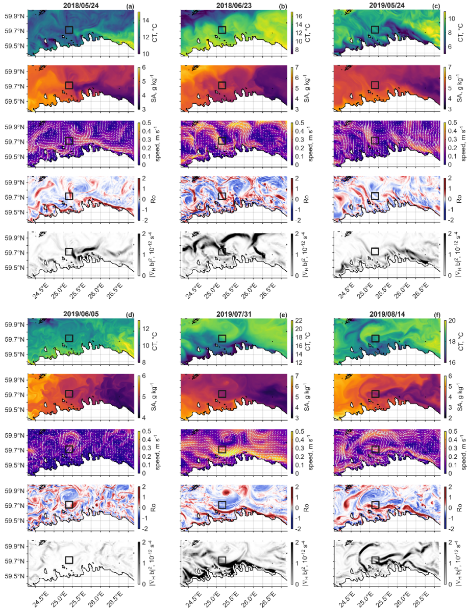
Figure 7. Overview of surface hydrographic and dynamical conditions in the GoF during spring–summer 2018–2019, illustrating the variability of SMS-relevant fields. Example dates characterizing the evolving dynamical background are shown in (a–c) first row: 24 May 2018, 23 June 2018, and 24 May 2019, and in (d–f) second row: 5 June, 31 July, and 14 August 2019. For each date, panels from top to bottom display surface (0–3 m) Conservative Temperature ( ^{\circ}\text{C} ), Absolute Salinity ( \text{g kg}^{-1} ), velocity ( \text{m s}^{-1} ), Rossby number, and squared horizontal buoyancy gradient modulus ( \text{s}^{-4} ). The black box marks the 10\times 10 km study window. Modified from Paper II.
