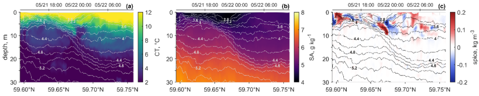
Figure 3. Representative example of SMS-related thermohaline deformation observed by a glider crossing a mesoscale front. Panels showing (a) temperature, (b) salinity, and (c) spice, with density contours overlaid at 0.2 \text{ kg m}^{-3} intervals, based on glider data from 21–22 May 2018. The area between ticks presenting latitude is approximately 5.5 km. Modified from Paper I.
